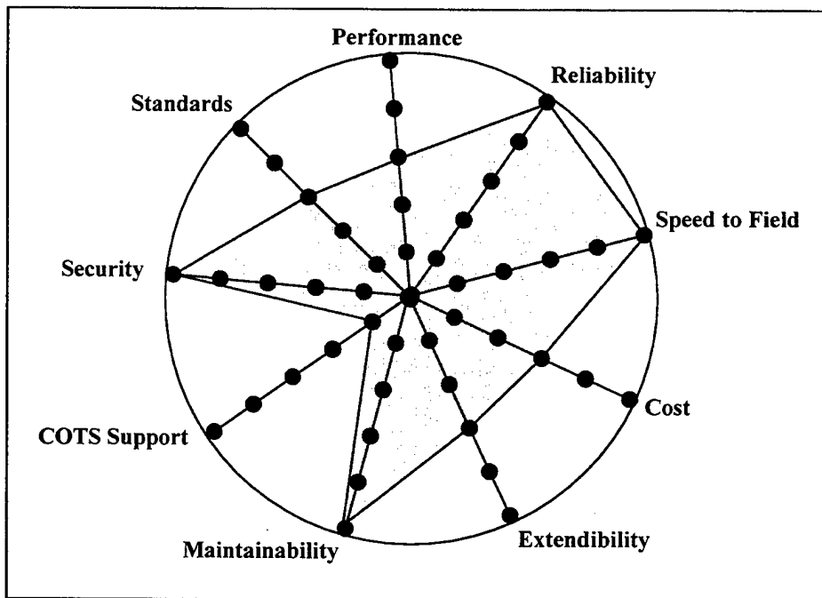
JINI Kiviatt Graph
