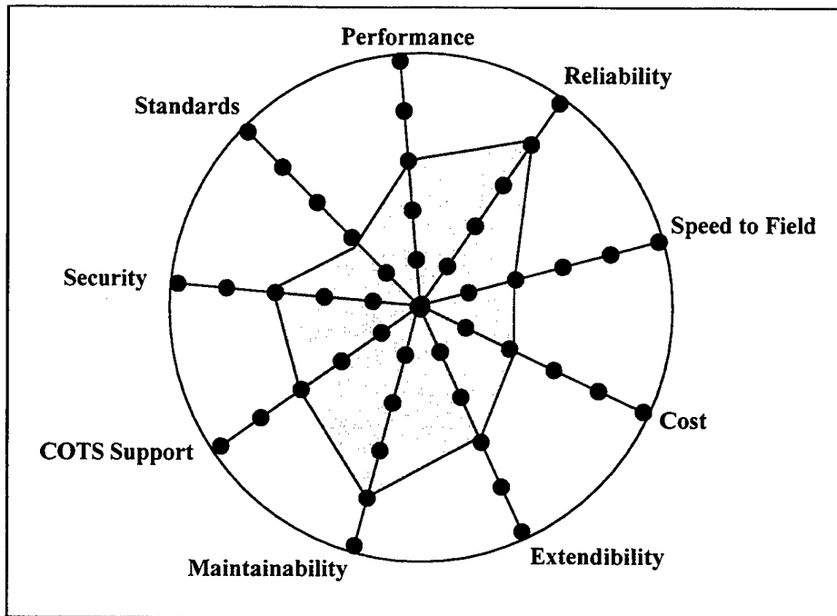
Data Mediator Kiviatt Graph
