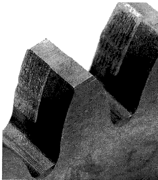
Figure 11.—Post test photograph at 100% torque, 10 000 RPM, and air jet only after primary lubrication termination.
