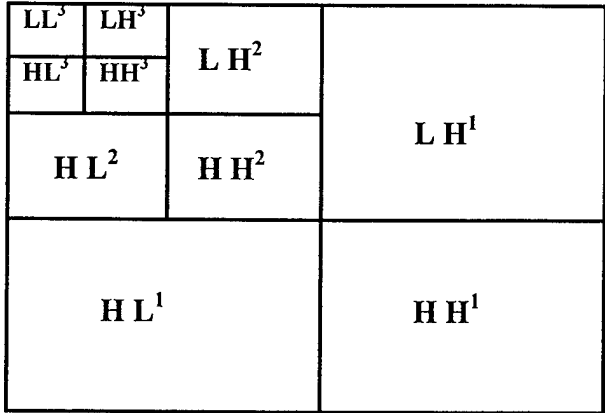
Figure 3, Three levels of wavelet decomposition
