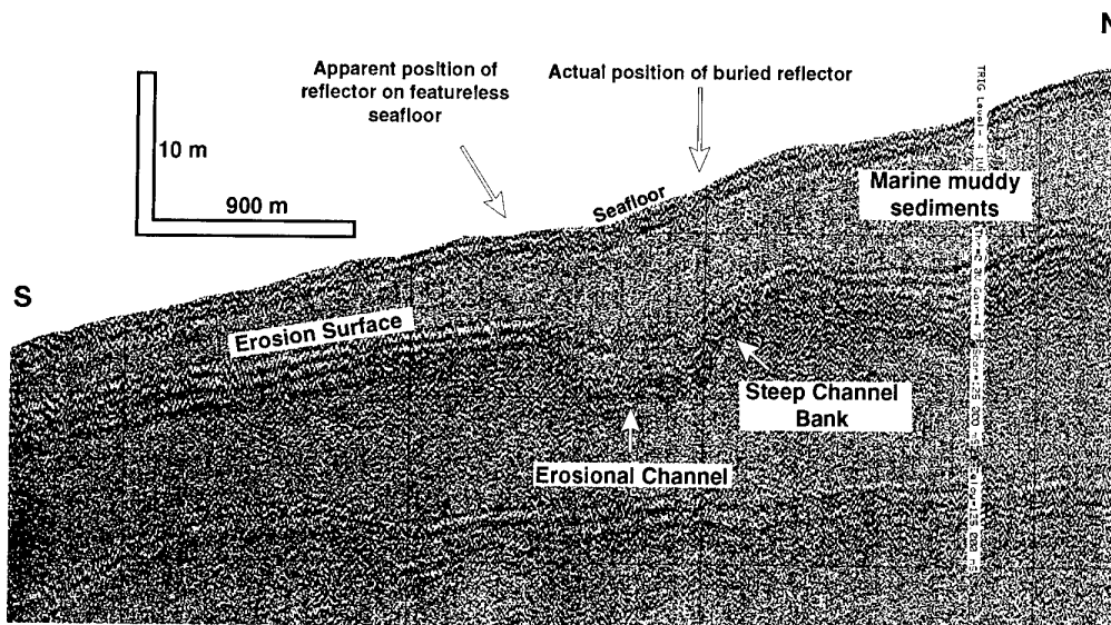
Figure 5 Buried symmetrical river channel. Note filling of lower part of channel with re-worked sands.
