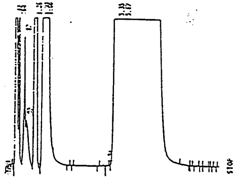
Figure 12: GC Chromatograms of the Gas Phase Analyses. (a) Standard Sample; (b) Effluent from Cetane Reaction; and (c) Effluent from Diesel Reaction.
