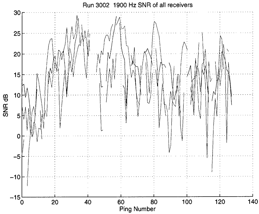
Figure 12 Analysis of Run 3002, 1900 Hz. SNR of the three receivers (1: blue; 2: green; 3: red) versus ping number.
