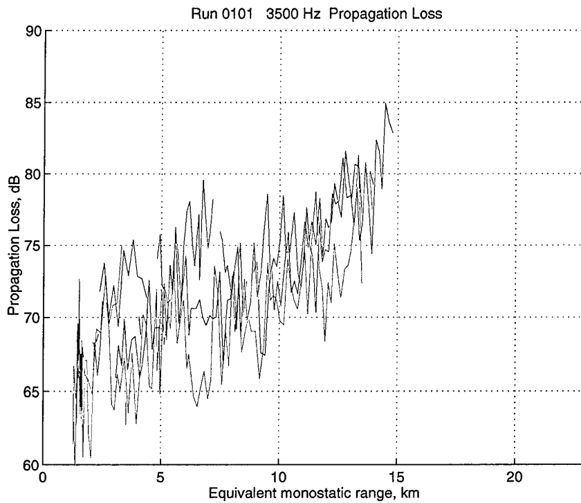
Figure 42 Run 0101, 3500 Hz. Propagation Loss for the three receivers (1: blue; 2: green; 3: red) versus equivalent monostatic range. Trajectory F.
