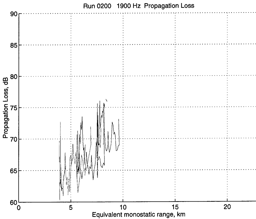
Figure 47 Run 0200, 1900 Hz. Propagation Loss for the three receivers (1: blue; 2: green; 3: red) versus equivalent monostatic range. Trajectory D.
