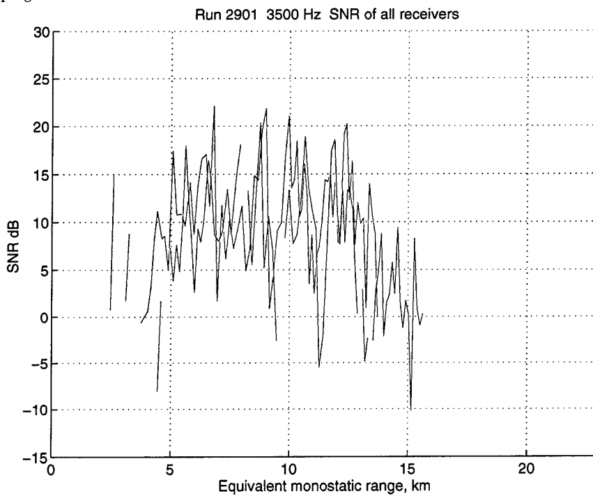
Figure 15 Analysis of Run 2901, 3500 Hz. SNR of the three receivers (1: blue; 2: green; 3: red) versus equivalent monostatic range.
