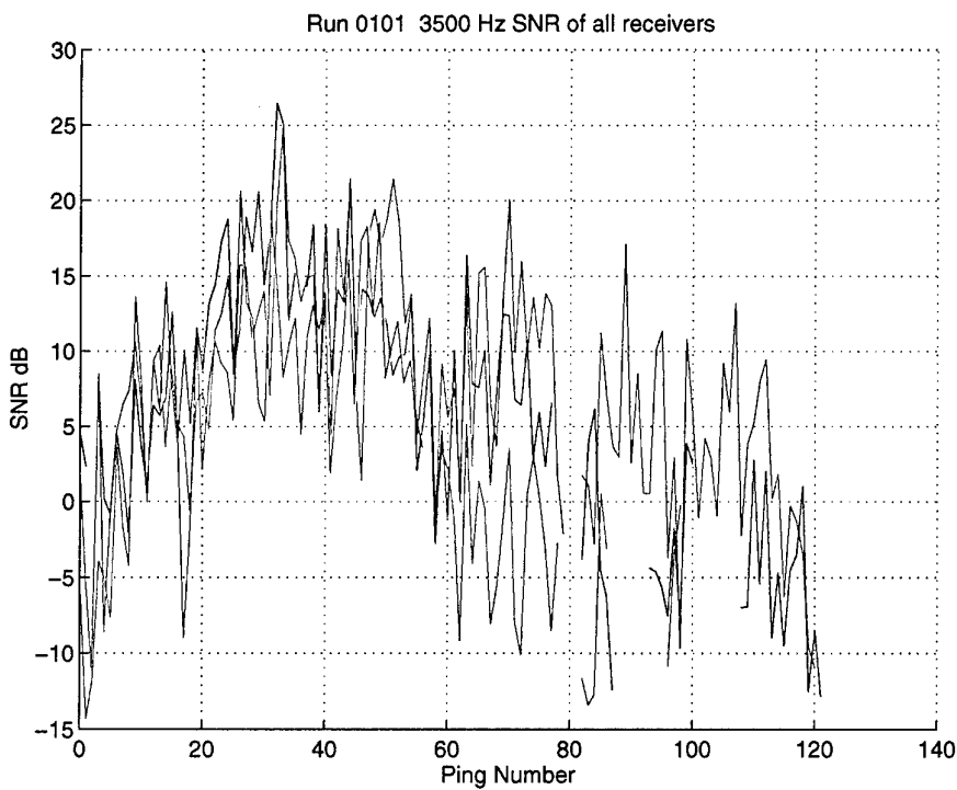
Figure 21 Analysis of Run 0101, 3500 Hz. SNR of the three receivers (1: blue; 2: green; 3: red) versus ping number.
