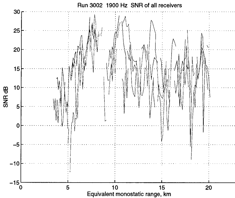
Figure 9 Analysis of Run 3002, 1900 Hz. SNR of the three receivers (1: blue; 2: green; 3: red) versus equivalent monostatic range
