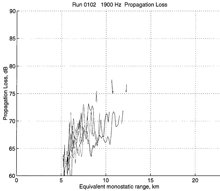
Figure 44 Run 0102, 1900 Hz. Propagation Loss for the three receivers (1: blue; 2: green; 3: red) versus equivalent monostatic range. Trajectory C.
