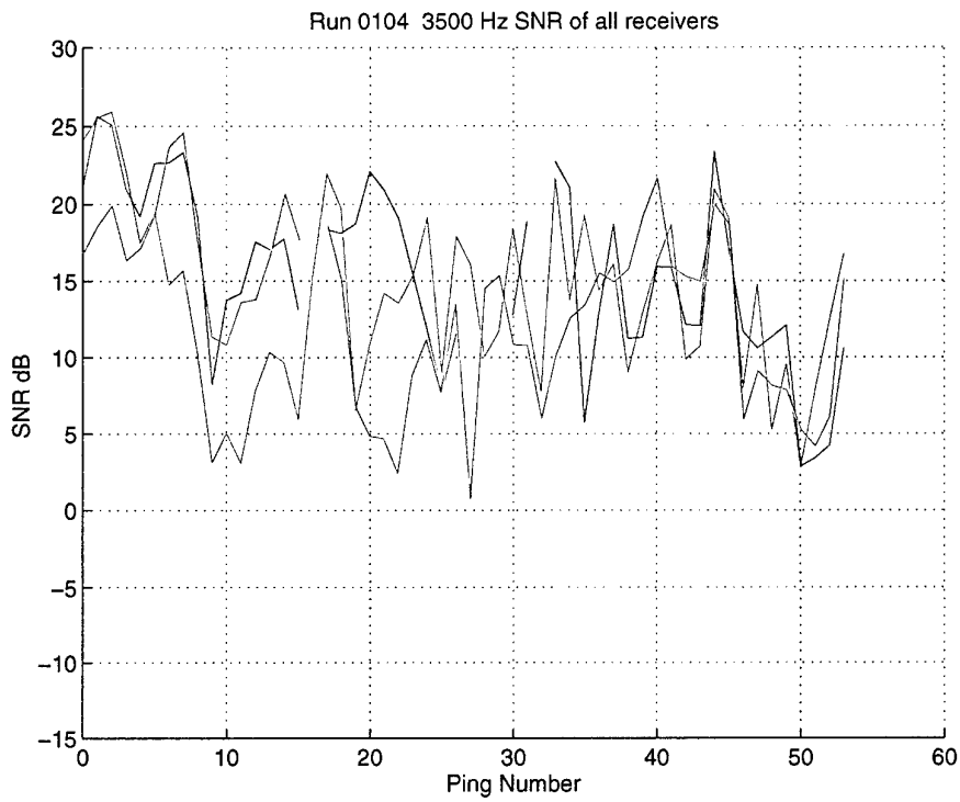
Figure 36 Analysis of Run 0104, 3500 Hz. SNR of the three receivers (1: blue; 2: green; 3: red) versus ping number.
