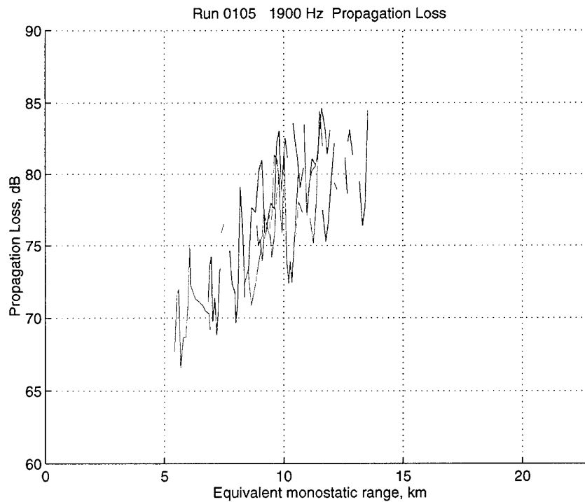
Figure 41 Run 0105, 1900 Hz. Propagation Loss for the three receivers (1: blue; 2: green; 3: red) versus equivalent monostatic range. Trajectory F.
