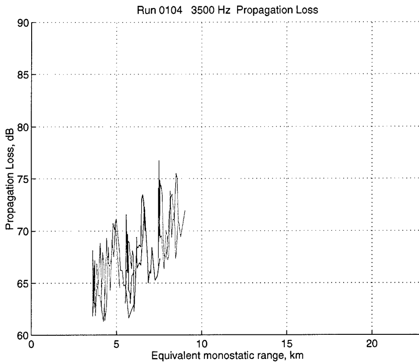
Figure 48 Run 0104, 3500 Hz. Propagation Loss for the three receivers (1: blue; 2: green; 3: red) versus equivalent monostatic range. Trajectory D.
