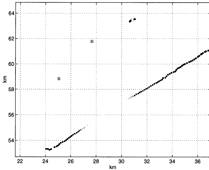
Figure 29 Analysis of Run 0102, 1900 Hz. Target trajectory from GPS data.
