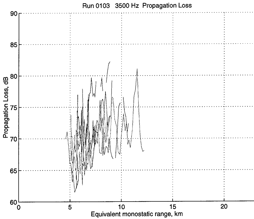
Figure 46 Run 0103, 3500 Hz. Propagation Loss for the three receivers (1: blue; 2: green; 3: red) versus equivalent monostatic range. Trajectory C.
