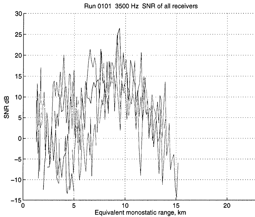
Figure 16 Analysis of Run 0101, 3500 Hz. SNR of the three receivers (1: blue; 2: green; 3: red) versus equivalent monostatic range.
