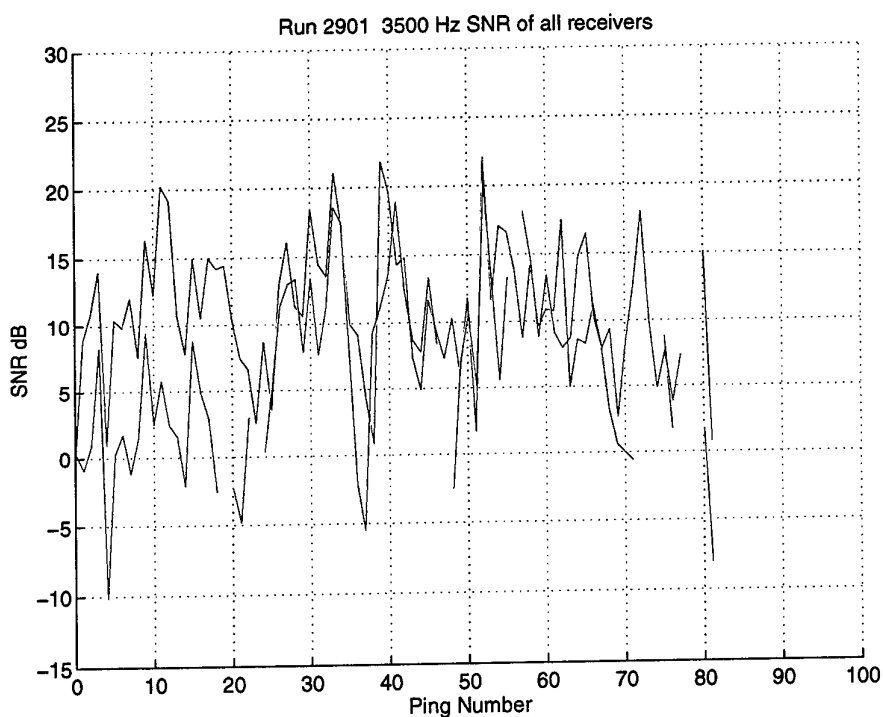
Figure 19 Analysis of Run 2901, 3500 Hz. SNR of the three receivers (1: blue; 2: green; 3: red) versus ping number.
