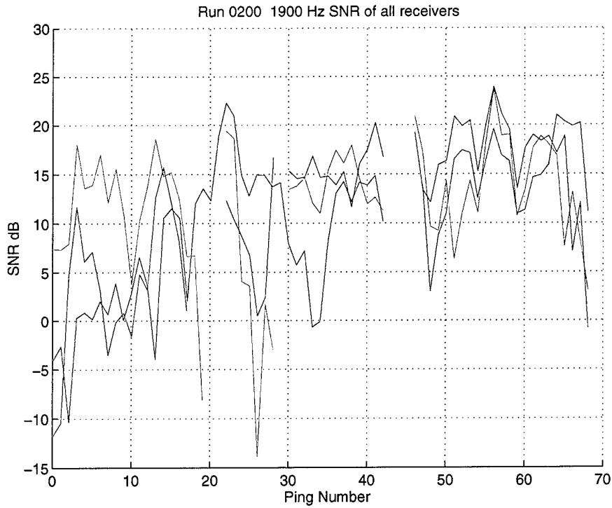
Figure 38 Analysis of Run 0200, 1900 Hz. SNR of the three receivers (1: blue; 2: green; 3: red) versus ping number.
