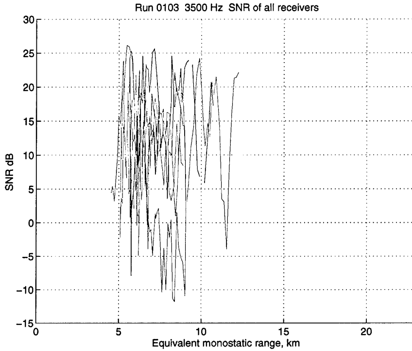
Figure 24 Analysis of Run 0103, 3500 Hz. SNR of the three receivers (1: blue; 2: green; 3: red) versus equivalent monostatic range.
