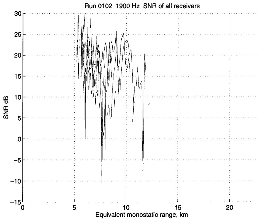
Figure 25 Analysis of Run 0102, 1900 Hz. SNR of the three receivers (1: blue; 2: green; 3: red) versus equivalent monostatic range.
