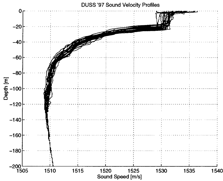
Figure 4. Sound velocity profiles measured during the tests.
