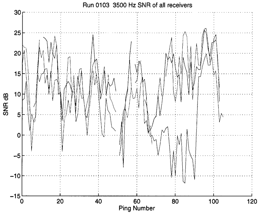
Figure 28 Analysis of Run 0103, 3500 Hz. SNR of the three receivers (1: blue; 2: green; 3: red) versus ping number.
