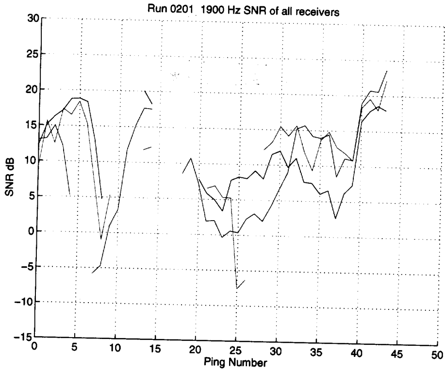
Figure 32 Analysis of Run 0201, 1900 Hz. SNR of the three receivers (1: blue; 2: green; 3: red) versus ping number.
