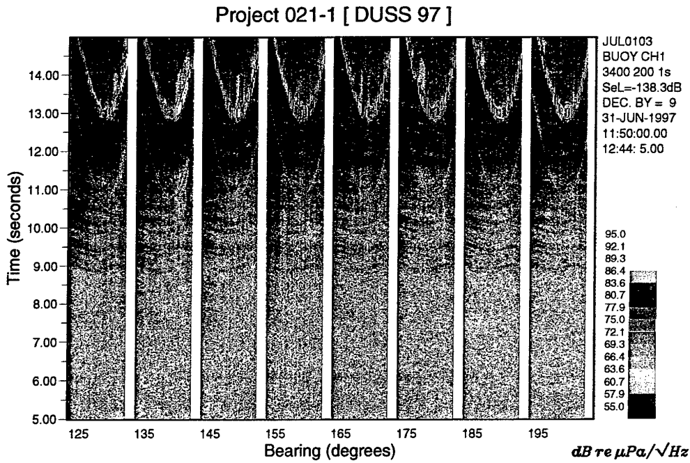
Figure 6 A significant example of detection display, with evident target track. Each column corresponds to a beam aiming at a fixed direction. Color corresponds to calibrated echo energy ( dB re \mu Pa \cdot \sqrt{s} ) and reverberation level (power spectral density, dB re \mu Pa/\sqrt{Hz} ). In each of these columns the X axis shows ping number and Y axis shows time after ping transmission.
