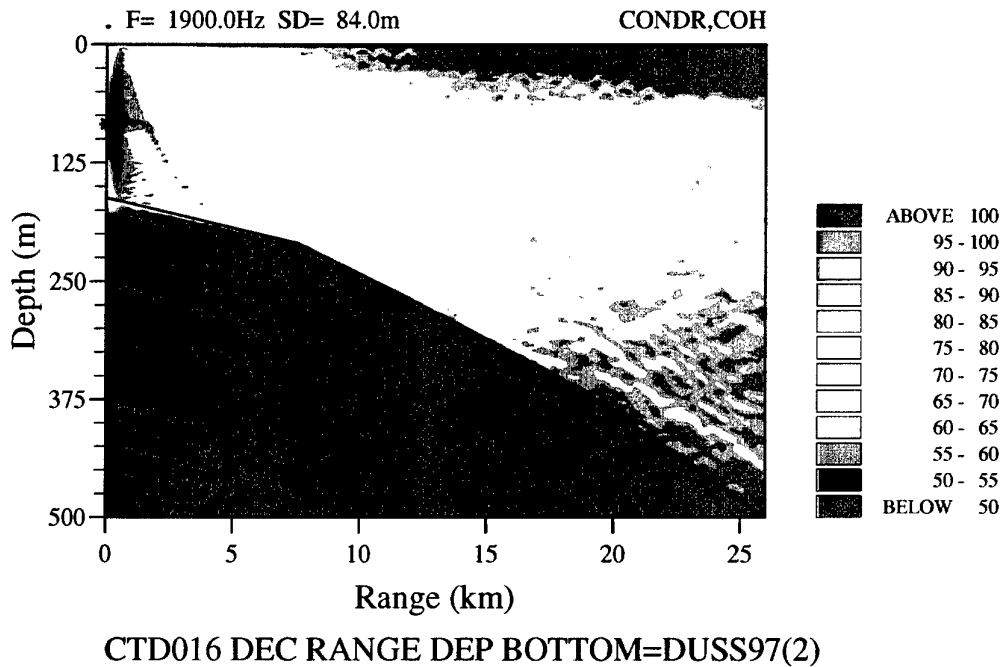
Figure 5 Propagation Loss computed with C-SNAP.
