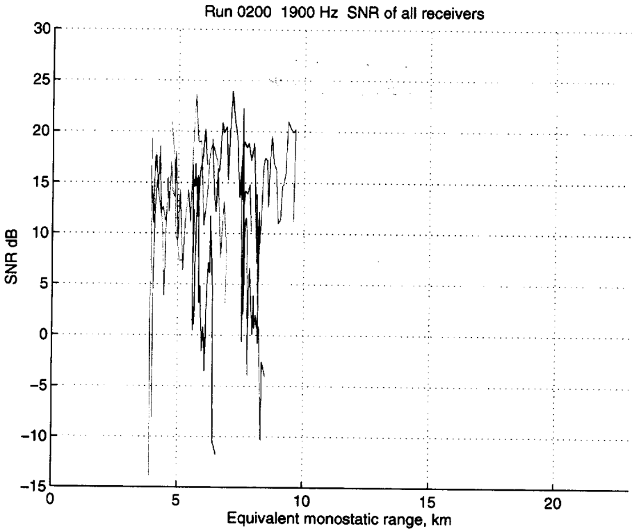
Figure 34 Analysis of Run 0200, 1900 Hz. SNR of the three receivers (1: blue; 2: green; 3: red) versus equivalent monostatic range.
