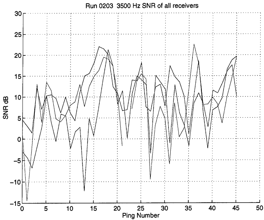
Figure 14 Analysis of Run 0203, 3500 Hz. SNR of the three receivers (1: blue; 2: green; 3: red) versus ping number.
