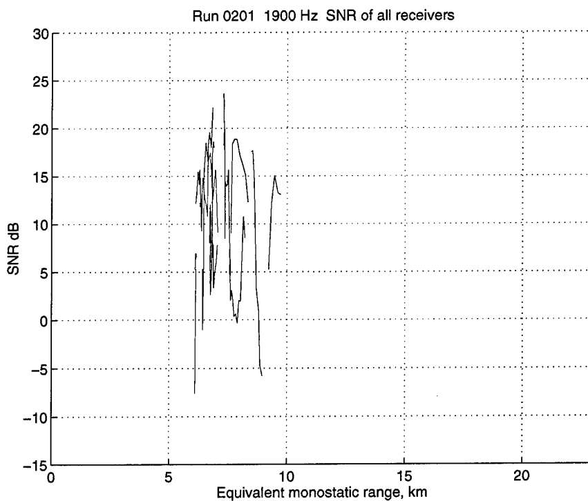
Figure 26 Analysis of Run 0201, 1900 Hz. SNR of the three receivers (1: blue; 2: green; 3: red) versus equivalent monostatic range.
