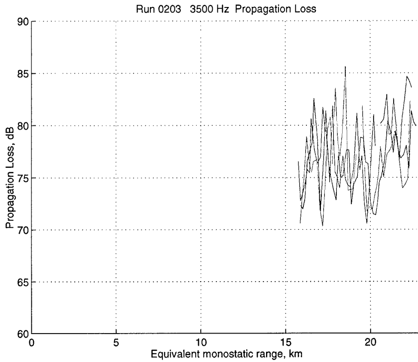
Figure 40 Run 0203, 3500 Hz. Propagation Loss for the three receivers (1: blue; 2: green; 3: red) versus equivalent monostatic range. Trajectory A.
