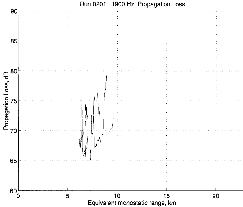
Figure 45 Run 0201, 1900 Hz. Propagation Loss for the three receivers (1: blue; 2: green; 3: red) versus equivalent monostatic range. Trajectory C.
