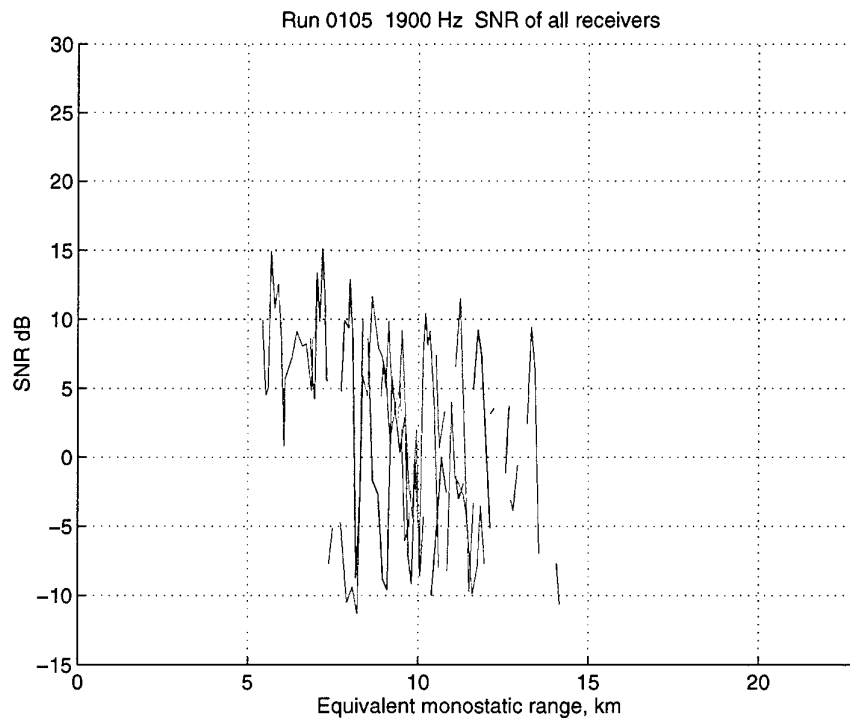
Figure 17 Analysis of Run 0105, 1900 Hz. SNR of the three receivers (1: blue; 2: green; 3: red) versus equivalent monostatic range.
