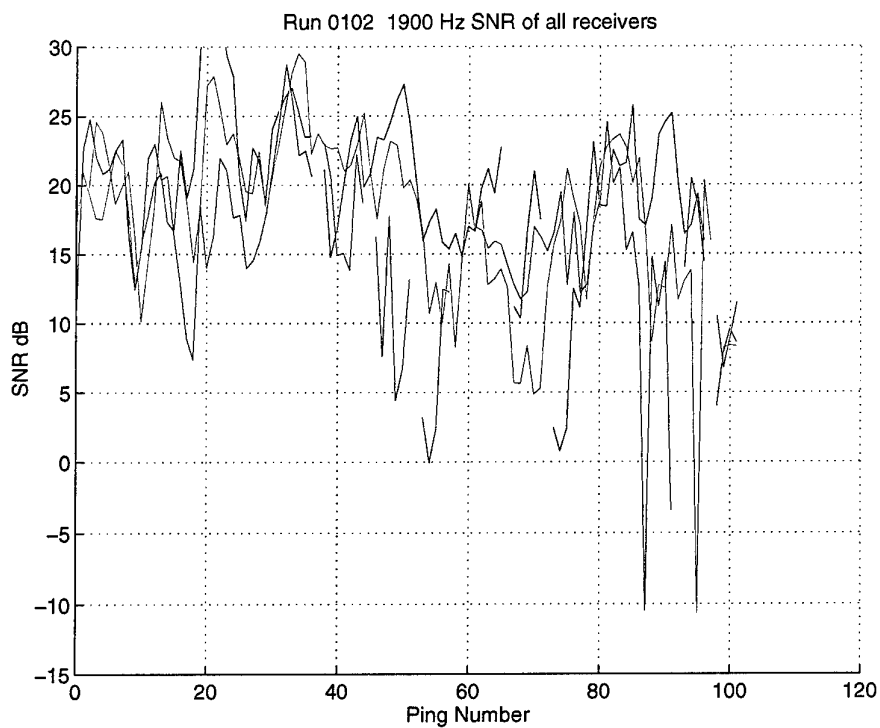
Figure 30 Analysis of Run 0102, 1900 Hz. SNR of the three receivers (1: blue; 2: green; 3: red) versus ping number.
