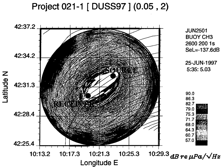
Figure 7 Polar display of reverberation.
