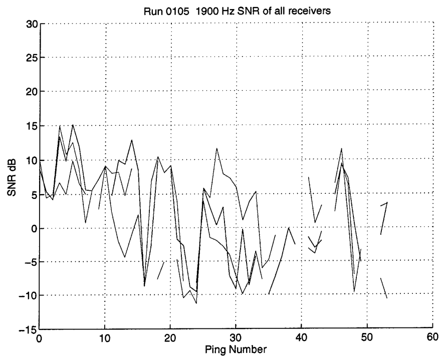
Figure 23 Analysis of Run 0105, 1900 Hz. SNR of the three receivers (1: blue; 2: green; 3: red) versus ping number.
