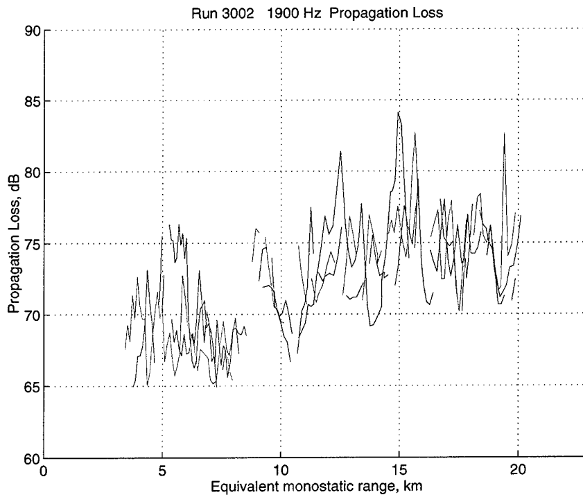
Figure 39 Run 3002, 1900 Hz. Propagation Loss for the three receivers (1: blue; 2: green; 3: red) versus equivalent monostatic range. Trajectory A.
