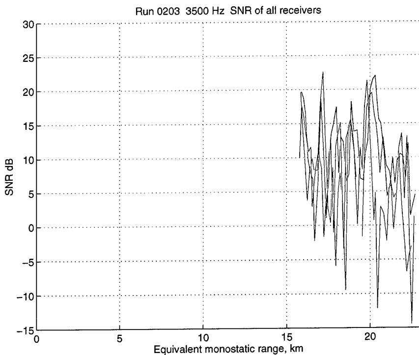
Figure 10 Analysis of Run 0203, 3500 Hz. SNR of the three receivers (1: blue; 2: green; 3: red) versus equivalent monostatic range.
