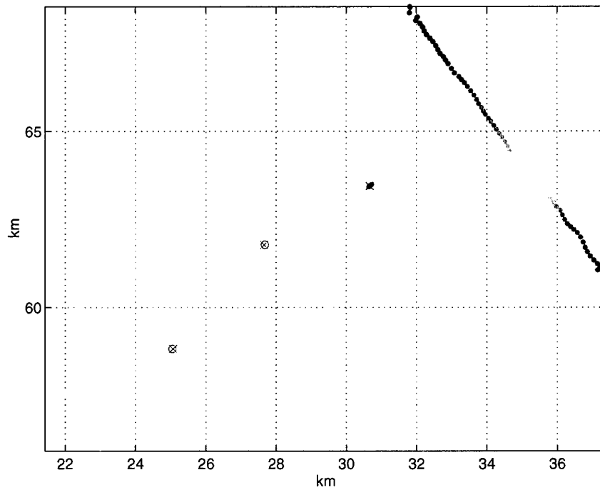
Figure 37 Analysis of Run 0200, 1900 Hz. Target trajectory from GPS data.
