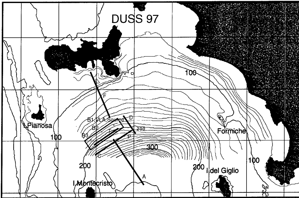
Figure 2 Geographical map of the test area, showing bottom bathymetry and deployment positions of sonar elements. The box indicates the reserved area for system deployment. Target trajectories (A..F) and towing ship trajectories (T) are shown.
