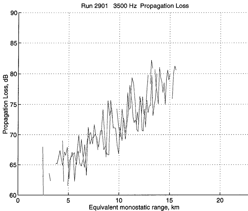
Figure 43 Run 02901, 3500 Hz. Propagation Loss for the three receivers (1: blue; 2: green; 3: red) versus equivalent monostatic range. Trajectory F.
