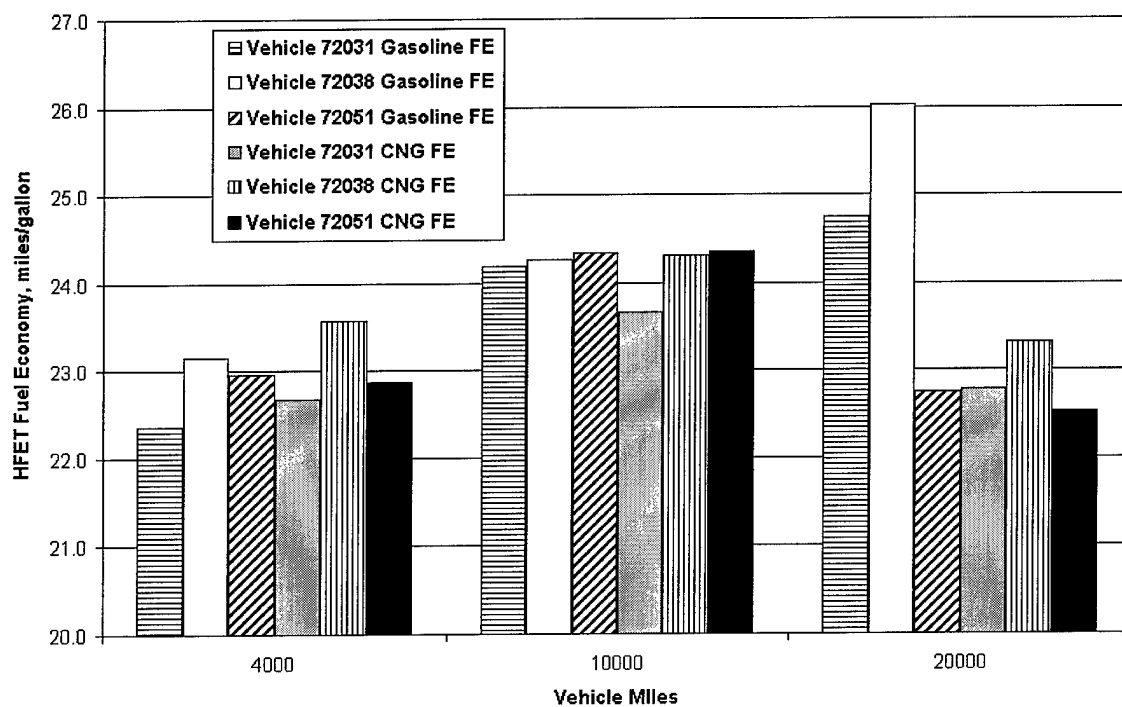
Figure 25. HFET Fuel Economy
