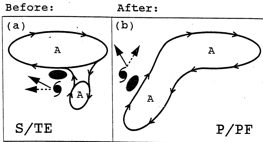
Figure 13. A conceptual model for the Ridge Modification by a TC (RMT) transformation from the (Before) Standard/Tropical Easterlies (S/TE) to the (After) Poleward/Poleward Flow (P/PF) synoptic pattern/region. A smaller (larger) TC will move along the dashed (solid) arrow because of the beta-effect propagation [from Carr and Elsberry (1999)].
