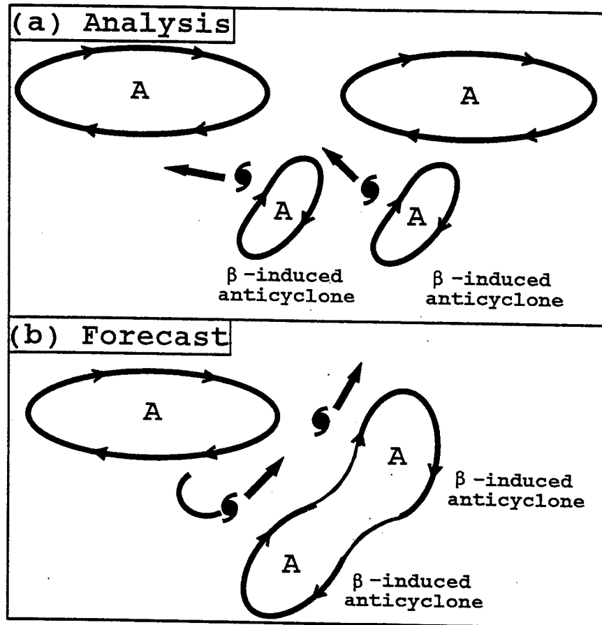
Figure 17. Conceptual model as in Fig. 13, except for a Reverse Trough Formation (RTF).
