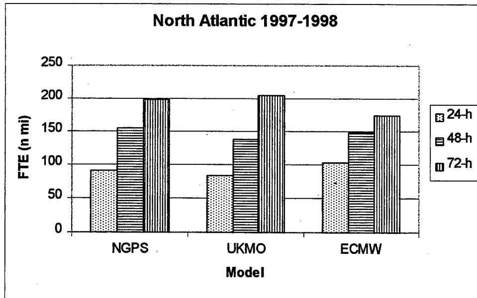
Figure 5. Average FTE for the NOGAPS, UKMO, and ECMWF during the 1997 and 1998 hurricane seasons.
