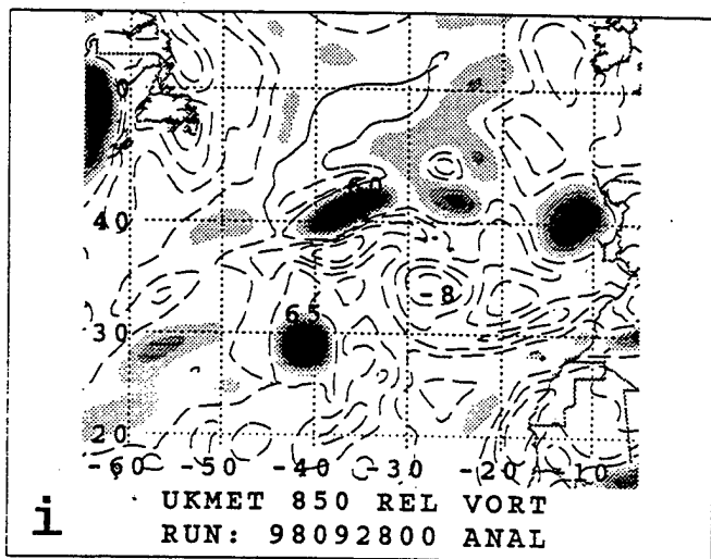
Figure 10. (a) Track of TC Jeanne (98-10L) and forecast tracks by selected models (see inset), with the dynamical models beginning at 0000 UTC 28 September 1998. The 72-h (asterisk) positions are shown for the dynamical models. Panels (b)-(h) as in Fig. 8,
