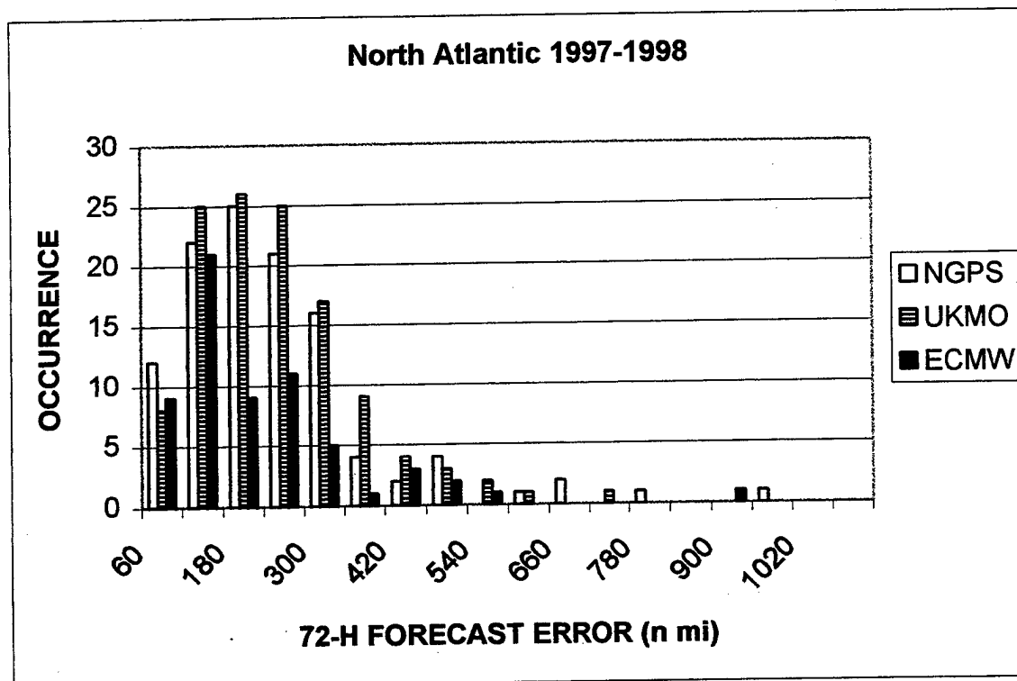
Figure 4. Frequency of occurrence of 72-h track errors for the NOGAPS, UKMO, and ECMWF forecasts of North Atlantic TCs during the 1997 and 1998 hurricane seasons.
