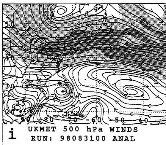
Figure 19. As in Fig. 8, except for NOGAPS and UKMO 500-mb wind forecasts for Danielle initiated at 0000 UTC 31 August 1998.
