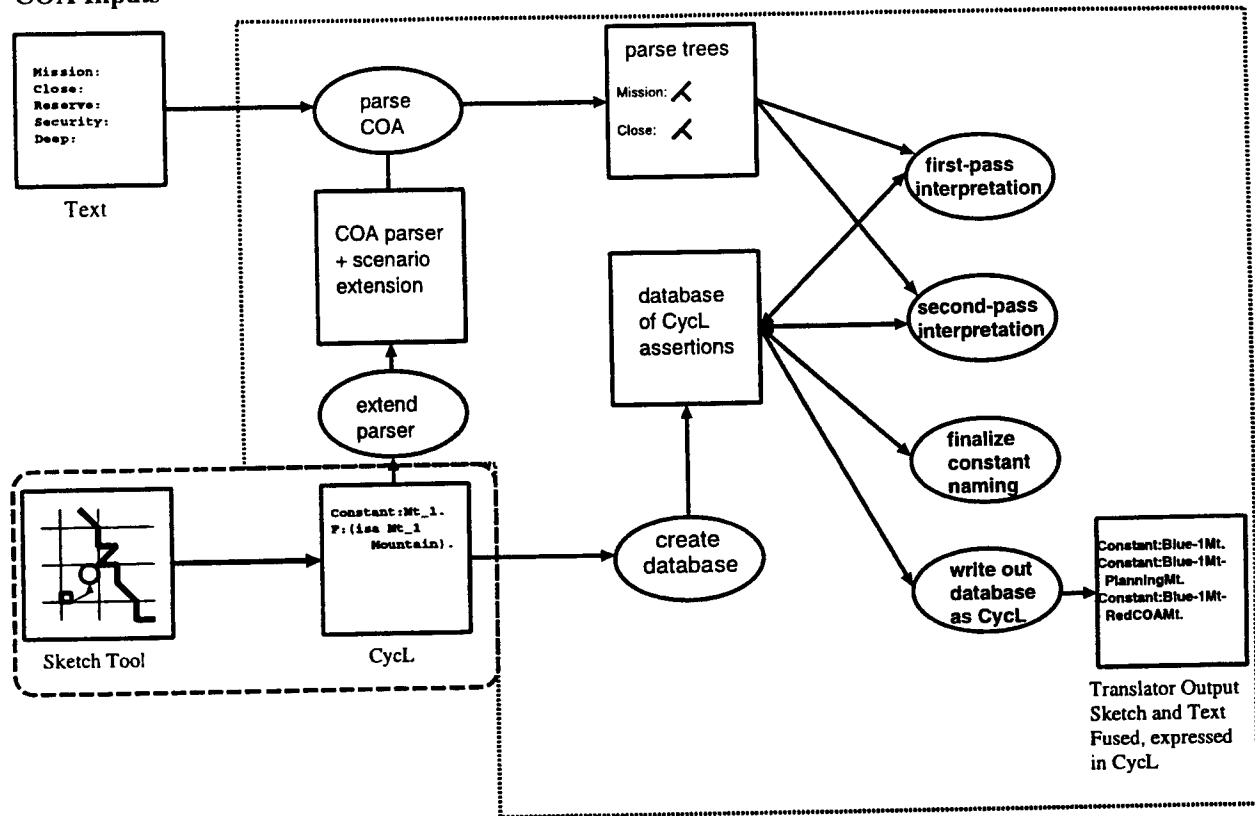
Figure 11: Translator Architecture
