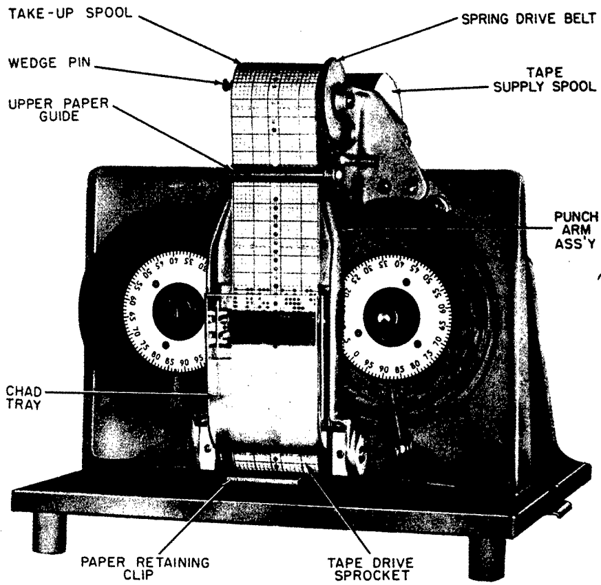
FIGURE III. Digital recorder.
