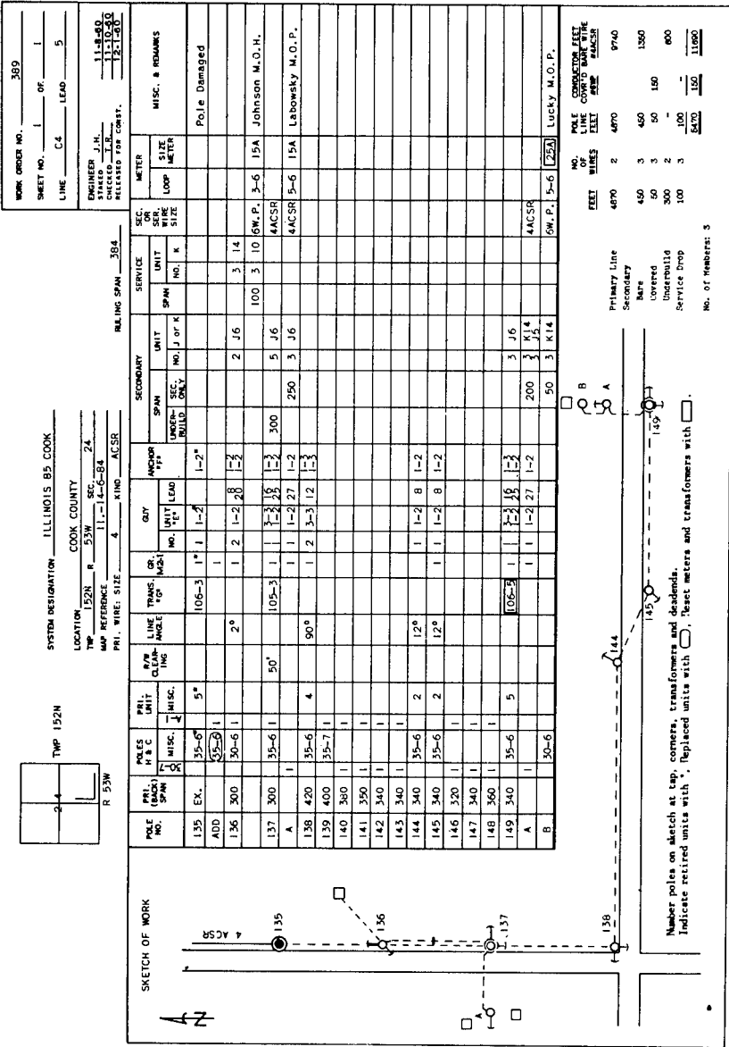
FIGURE VII. Staking sheet.
