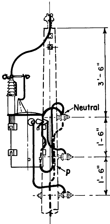
FIGURE IV. Single-phase transformer.
