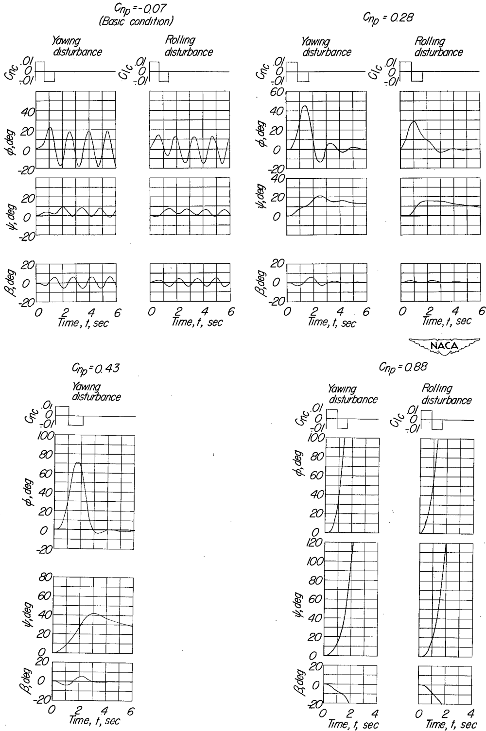
Figure 17.- Calculated response of model to yawing or rolling disturbance for various values of C_{np} .
