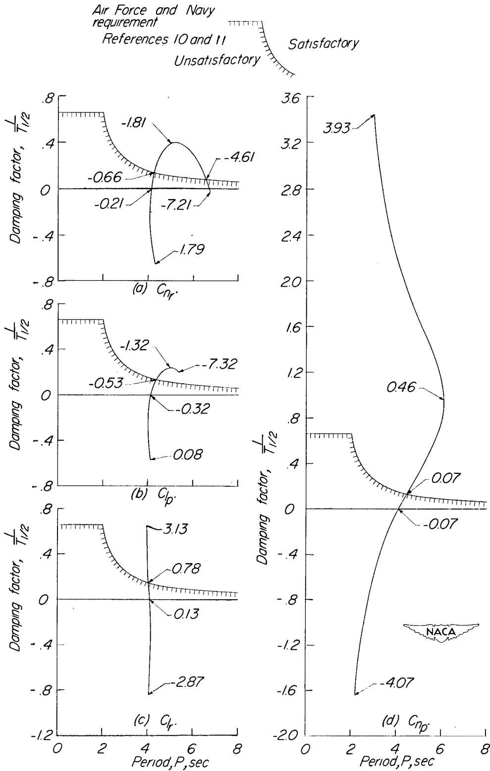
Figure 20.- Effect of change in rotary derivatives on damping of lateral oscillation and comparison with Air Force and Navy requirement.
