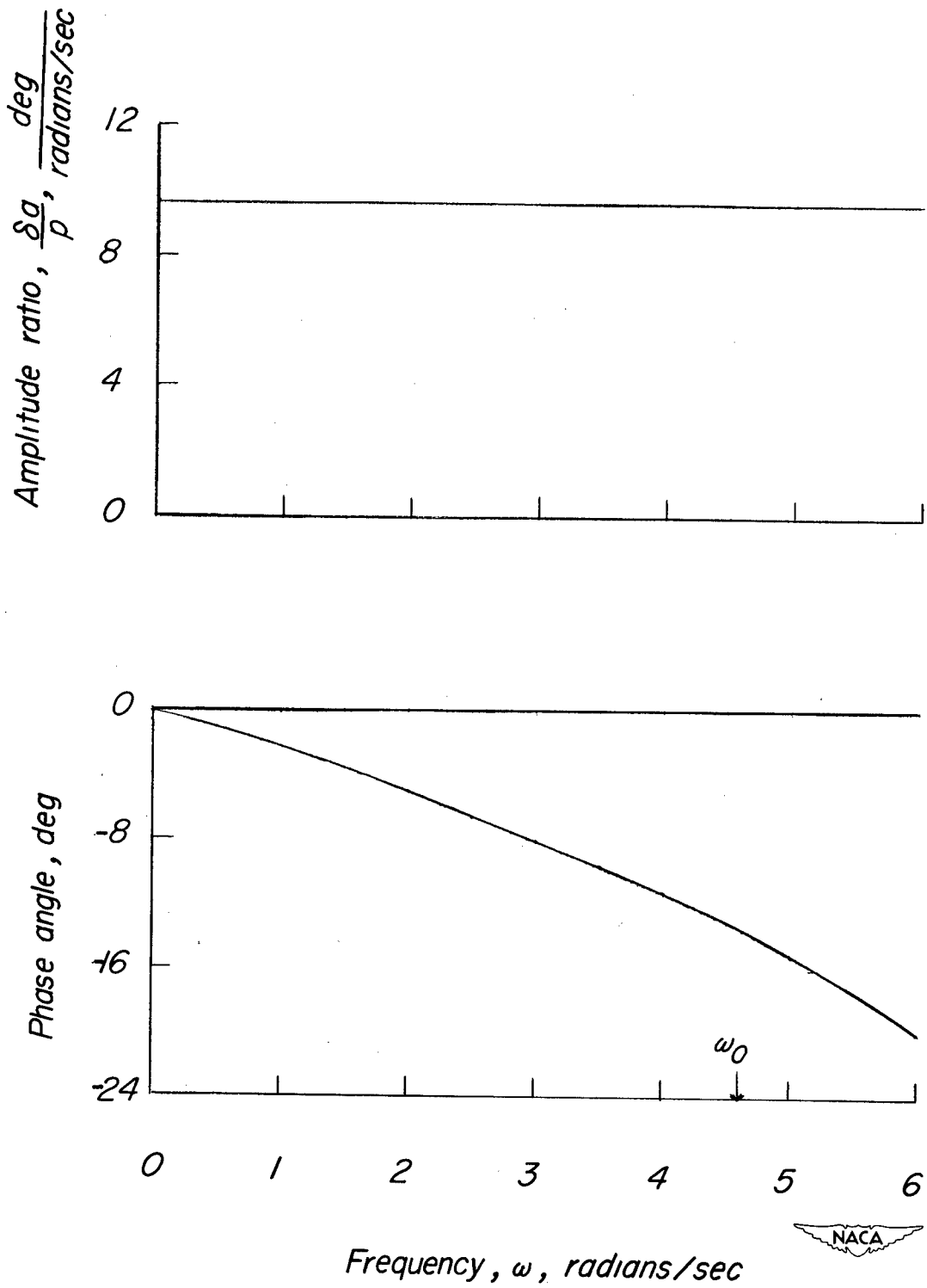
Figure 5.- Example of frequency-response data for artificial-stabilization device. (Case shown is for C_{l_p} = -1.0 .)
