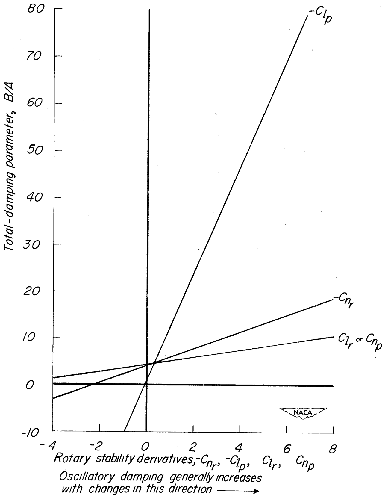
Figure 19.- Calculated effect of rotary stability derivatives on total damping.
