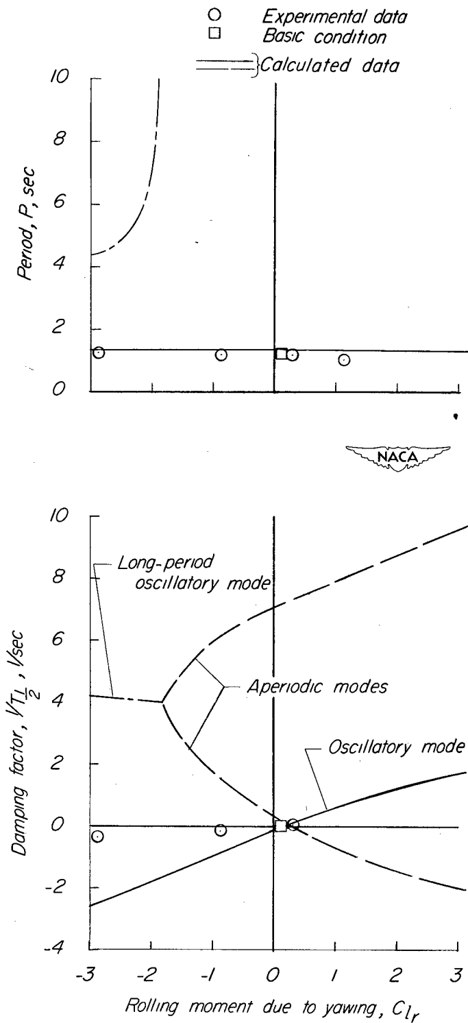
Figure 13.- Calculated effect of C_{lr} on stability and comparison with experimental data.
