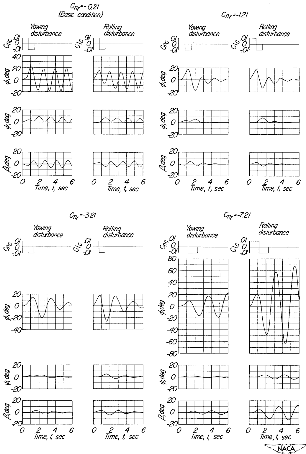
Figure 8.- Calculated response of model to yawing or rolling disturbance for various values of C_{nr} .
