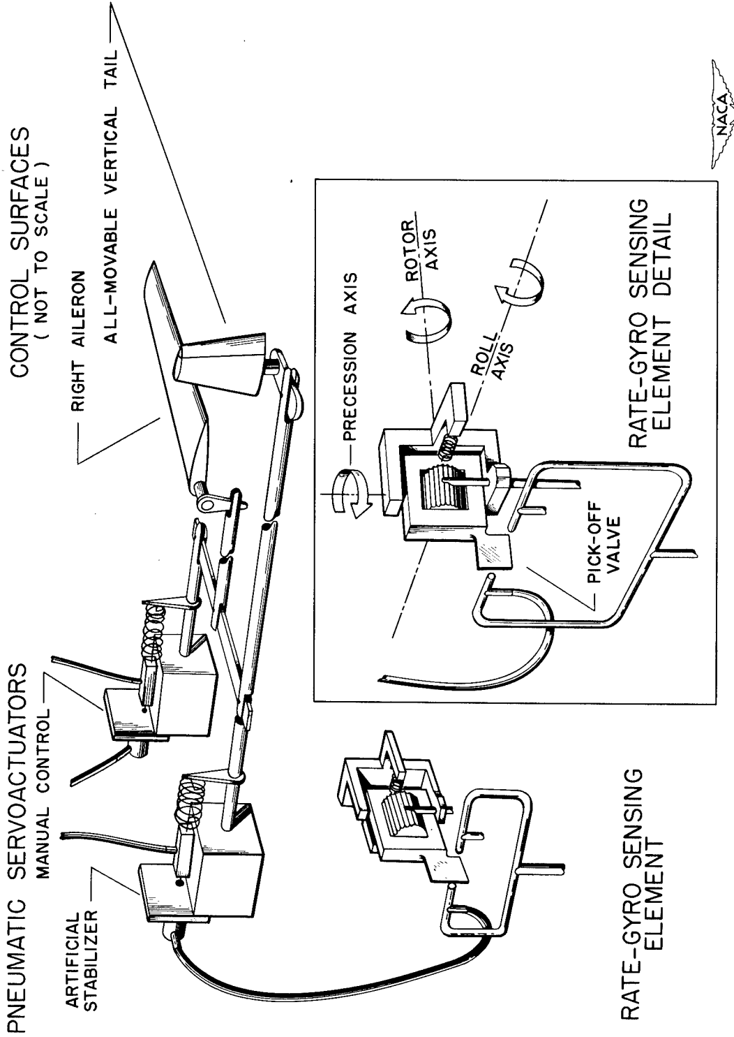
Figure 4.- Sketch of artificial-stabilization system. Arrangement for producing C_{lp} is shown.
