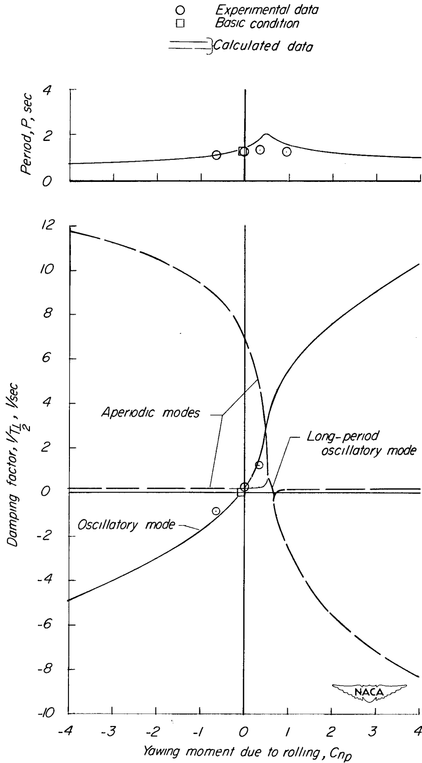
Figure 16.- Calculated effect of C_{np} on stability and comparison with experimental data.
