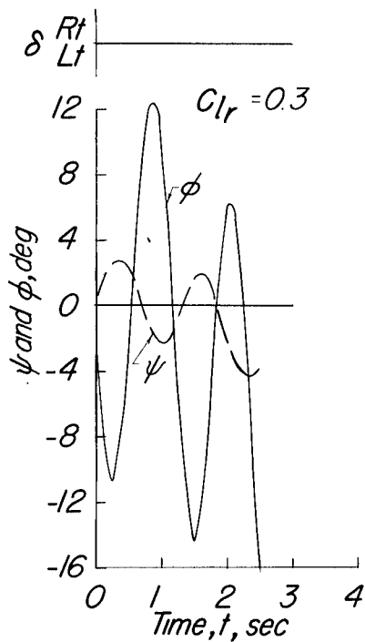
Figure 12.- Flight records of the lateral motions for various values of C_{lr} .
