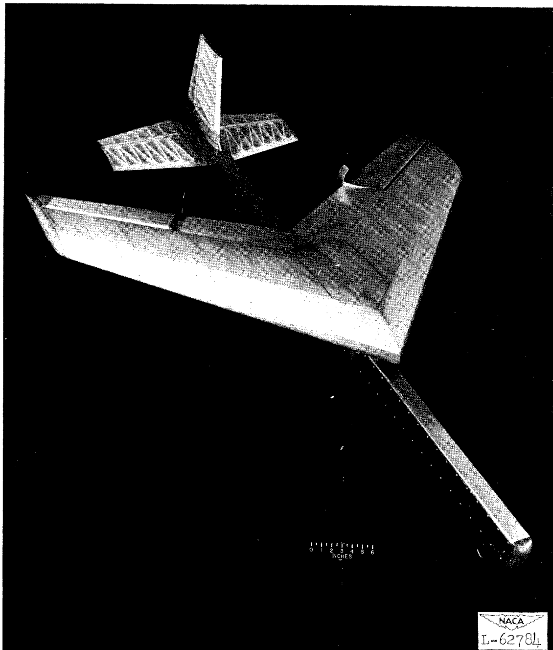
Figure 3.- Model used in free-flight tunnel tests.
