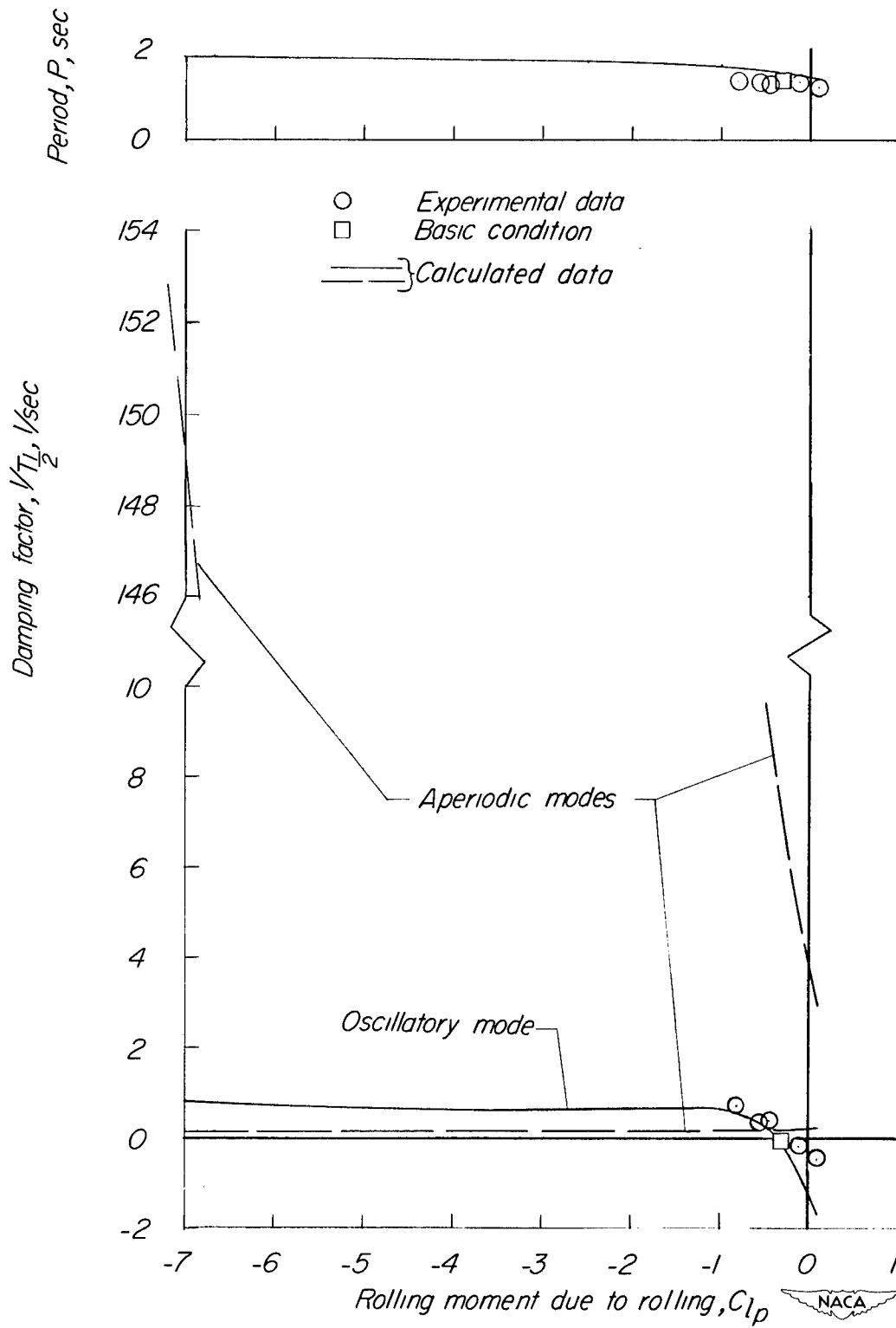
Figure 10.- Calculated effect of C_{l_p} on stability and comparison with experimental data.
