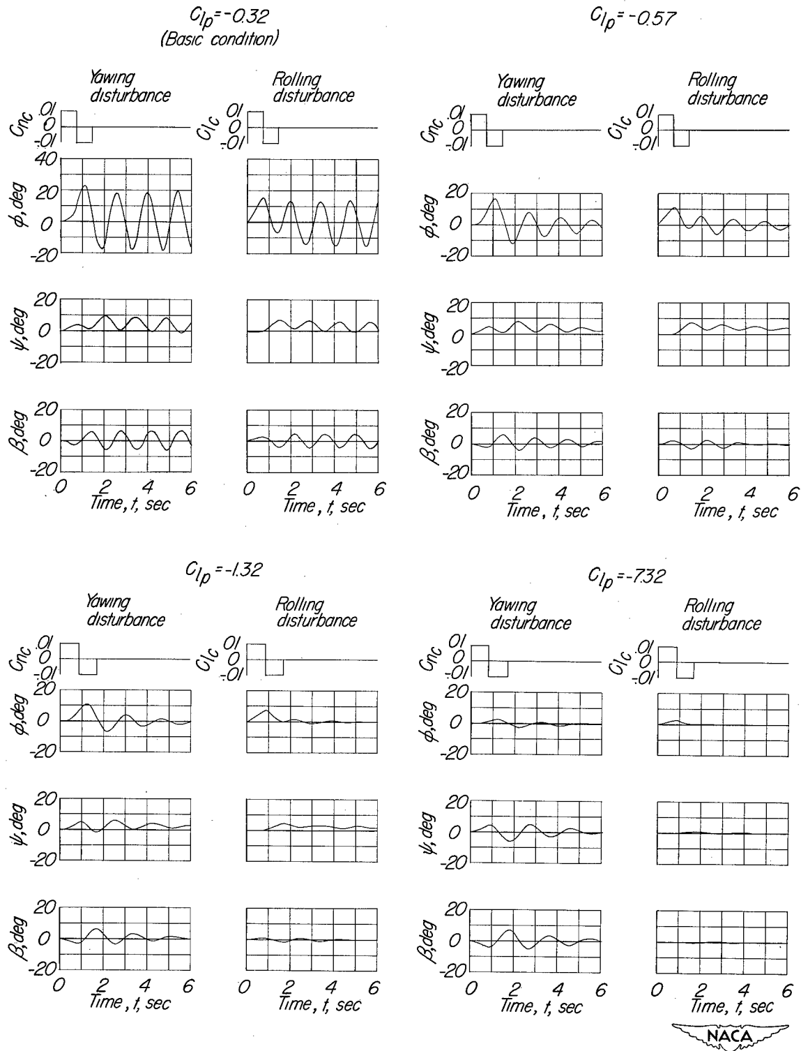
Figure 11.- Calculated response of model to yawing or rolling disturbance for various values of C_{l_p} .
