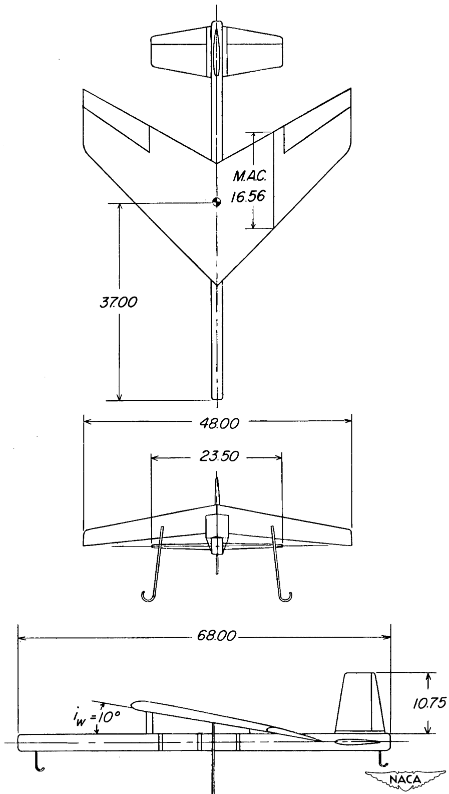
Figure 2.- Three-view drawing of test model. All dimensions in inches.
