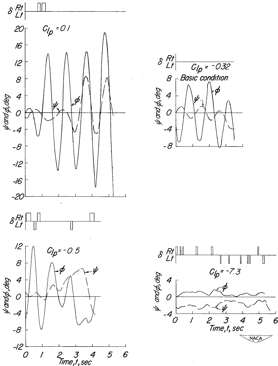
Figure 9.- Flight records of the lateral motions for various values of C_{lp} .
