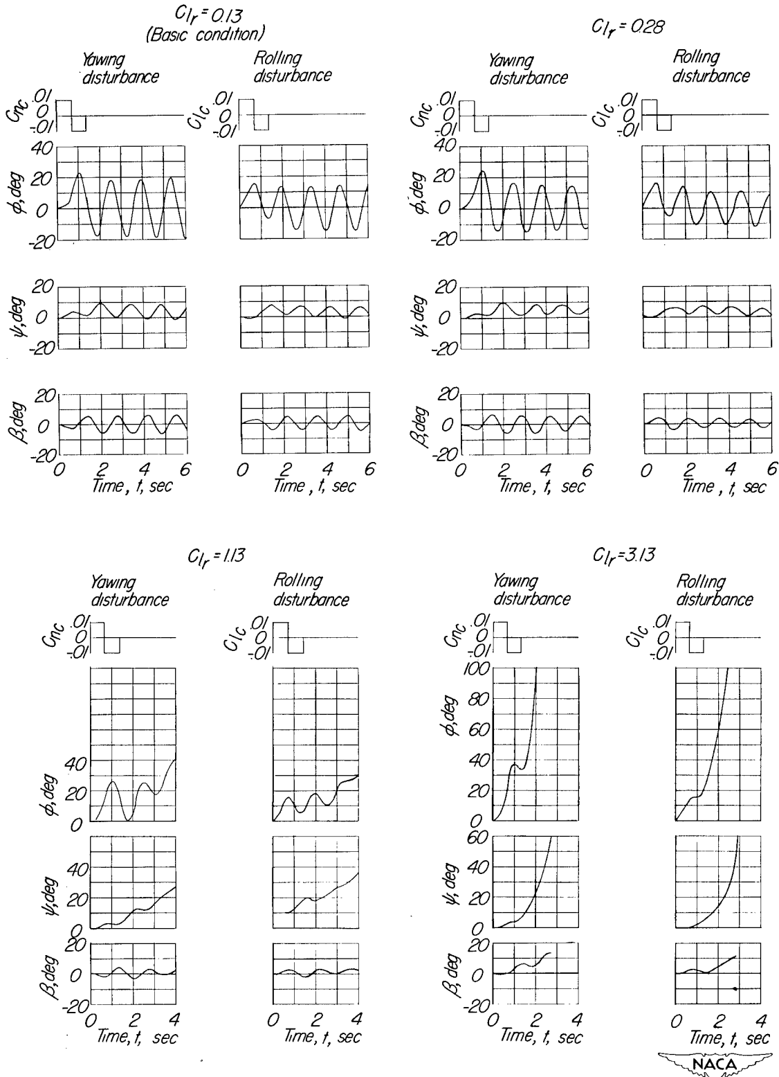
Figure 14.- Calculated response of model to yawing or rolling disturbance for various values of C_{l_r} .
