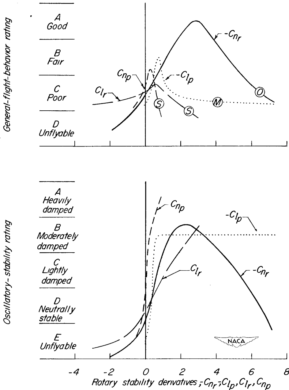
Figure 18.- Effect of variation in rotary derivatives on general flight behavior and oscillatory stability. (Data from table II.)
