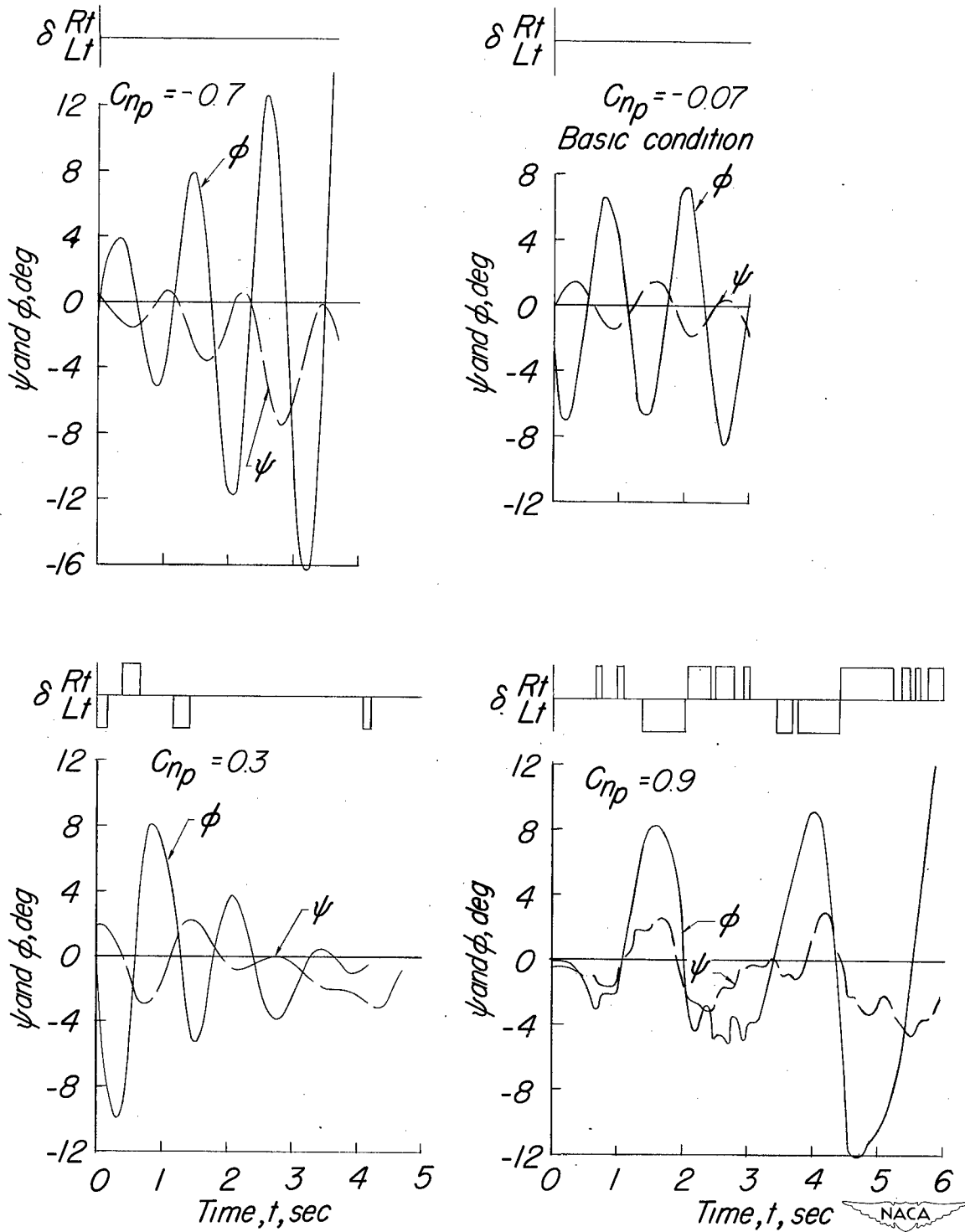
Figure 15.- Flight records of the lateral motions for various values of C_{np} .
