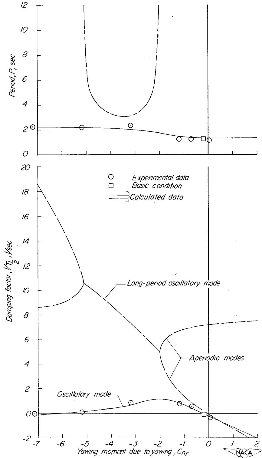
Figure 7.- Calculated effect of C_{nr} on stability and comparison with experimental data.
