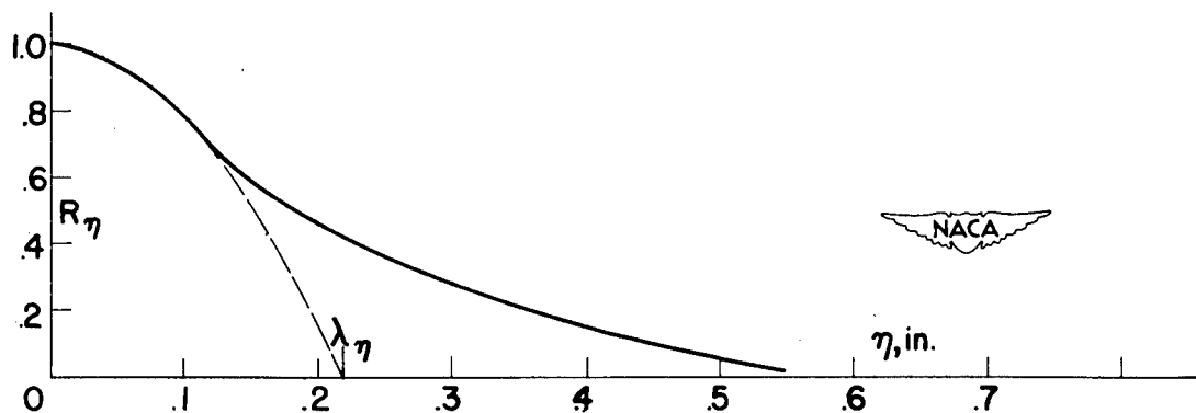
(b) Correlation function R_\eta .
