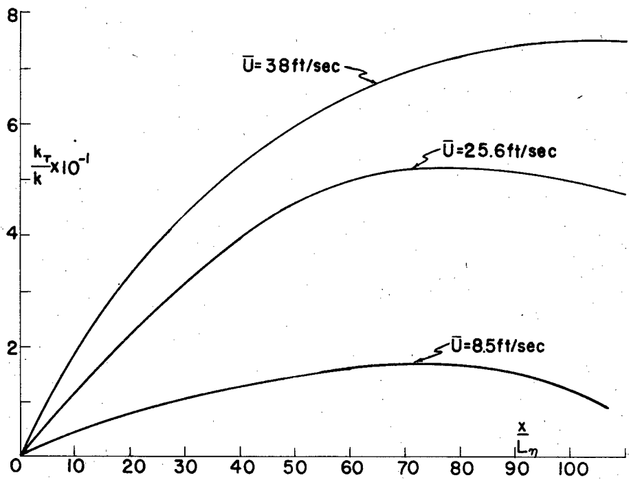
(a) Turbulent-heat-transfer coefficient at three air speeds. M = 1 inch and \frac{x_0}{M} = 43.4 .
