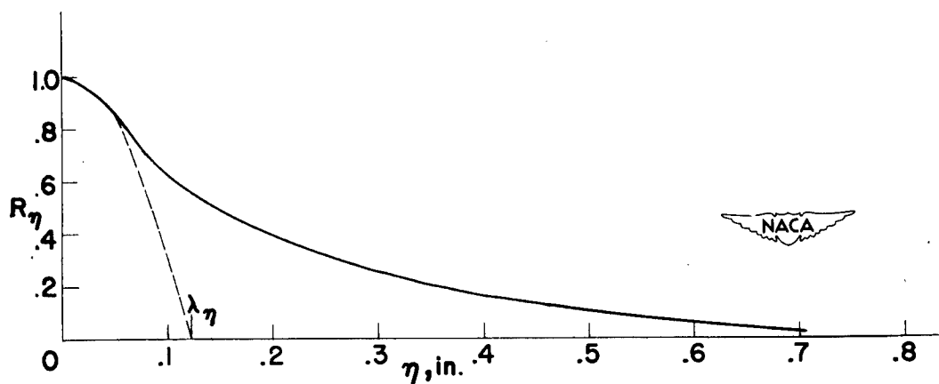
(b) Correlation function R_\eta .
