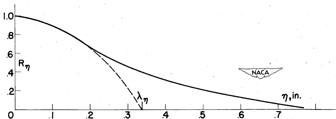
(b) Correlation function R_\eta .
