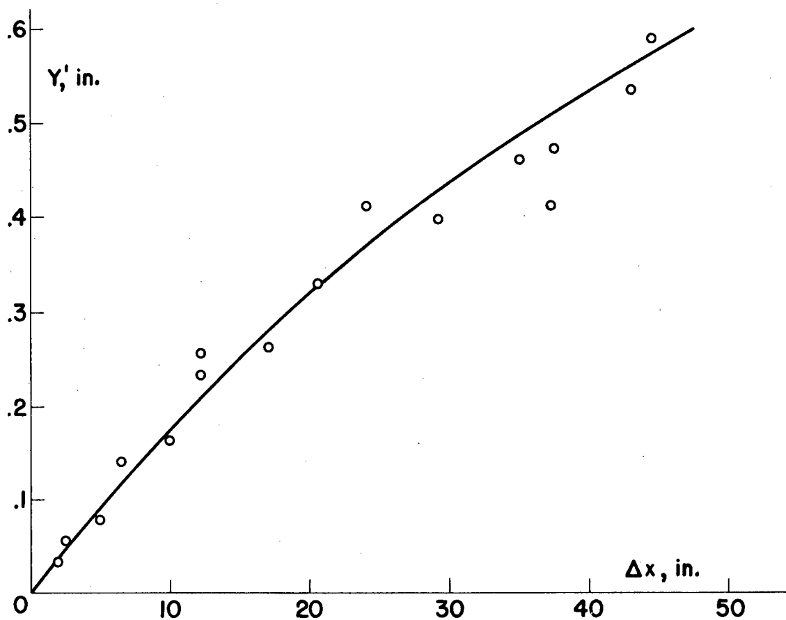
(a) Spread of heat from a line source.
