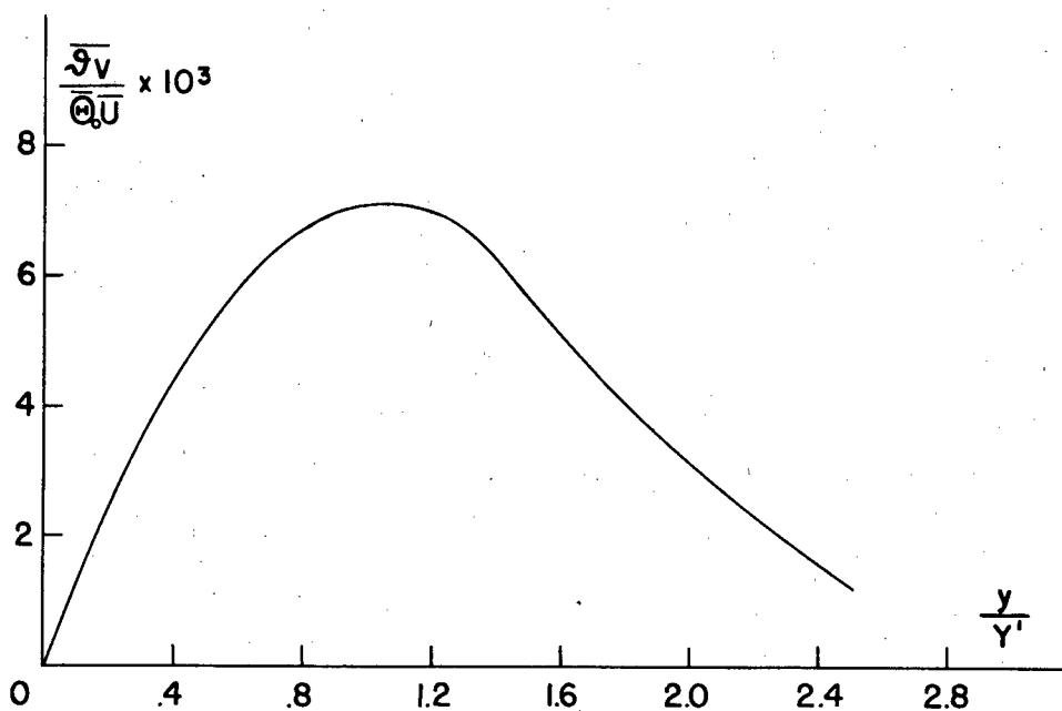
(a) \frac{\overline{\partial v}}{\partial_0 U} against \frac{y}{Y'} .
