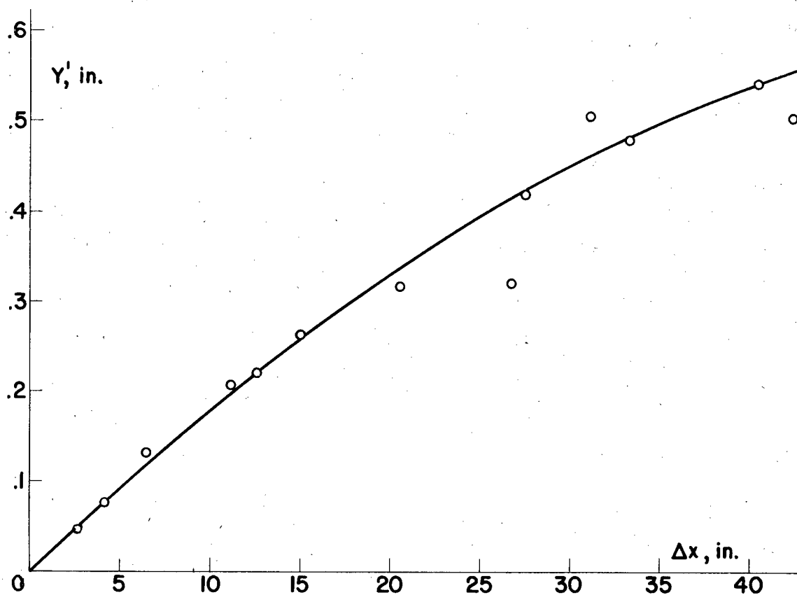
(a) Spread of heat from a line source.
