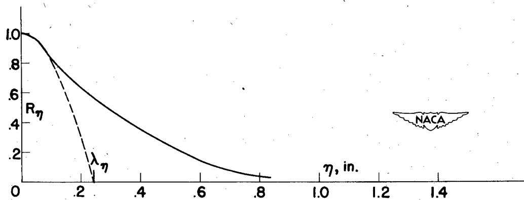
(b) Correlation function R_\eta .
