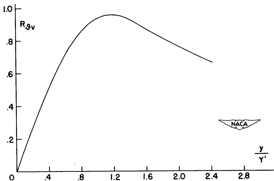
(b) R_{\partial v} against y/Y' .
