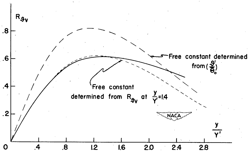
(b) R_{\partial v} against y/Y' . Dashed curves are result of analysis based on rectangular temperature pulses.
