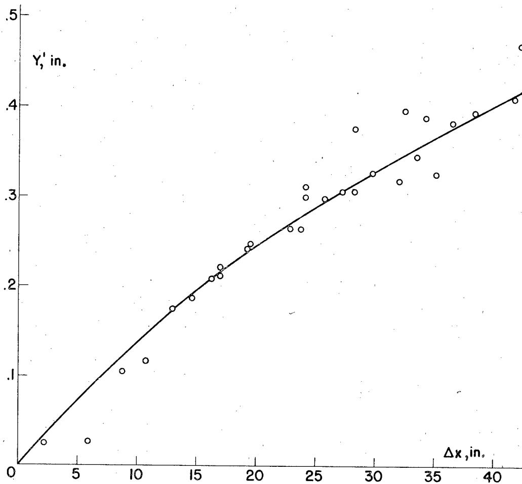
(a) Spread of heat from a line source.
