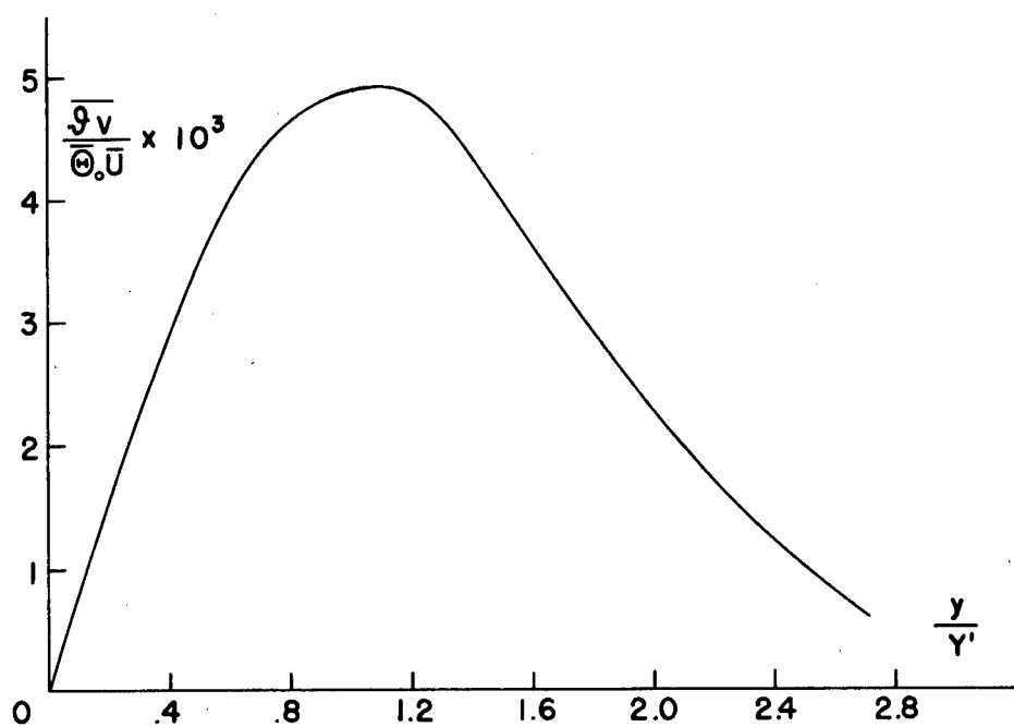
(a) \frac{\overline{\partial v}}{\partial_0 \bar{U}} against \frac{y}{Y'} .
