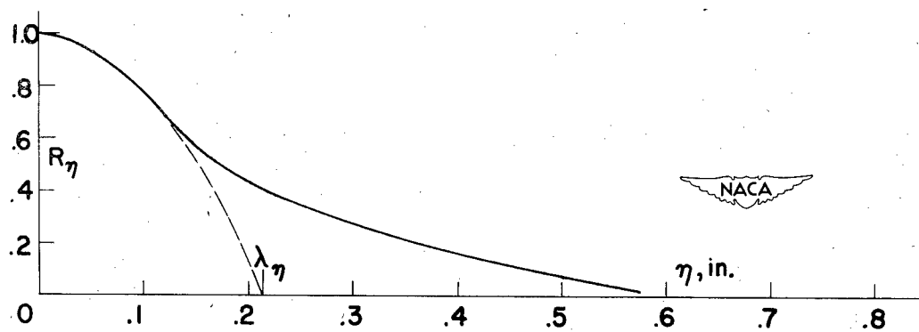
(b) Correlation function R_\eta .
