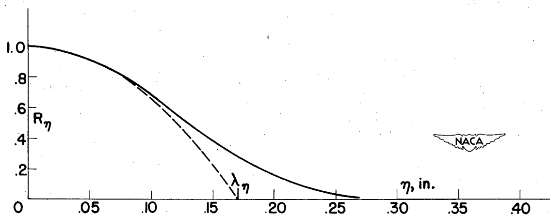
(b) Correlation function R_\eta .
