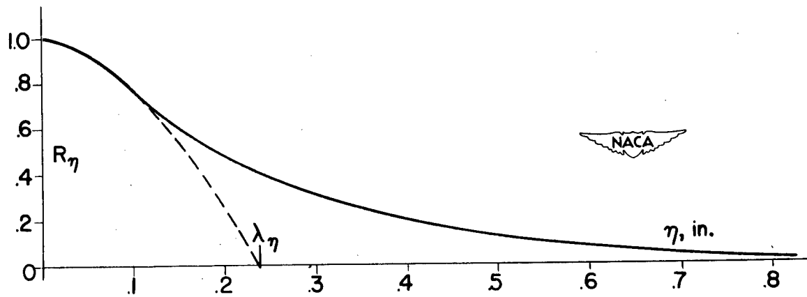
(b) Correlation function R_\eta .
