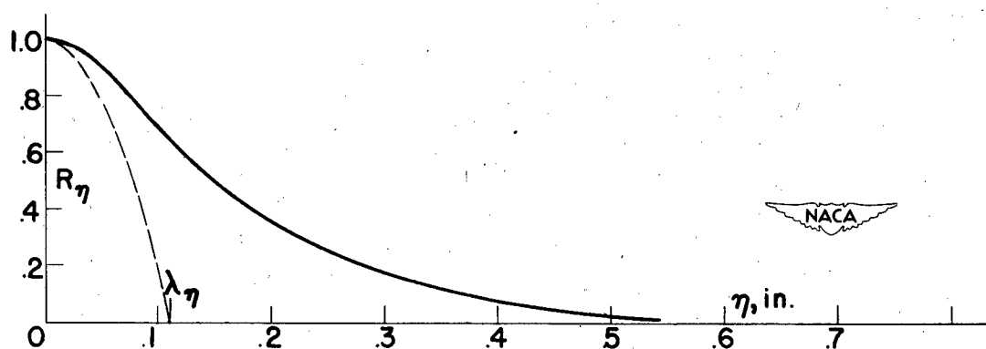
(b) Correlation function R_\eta .
