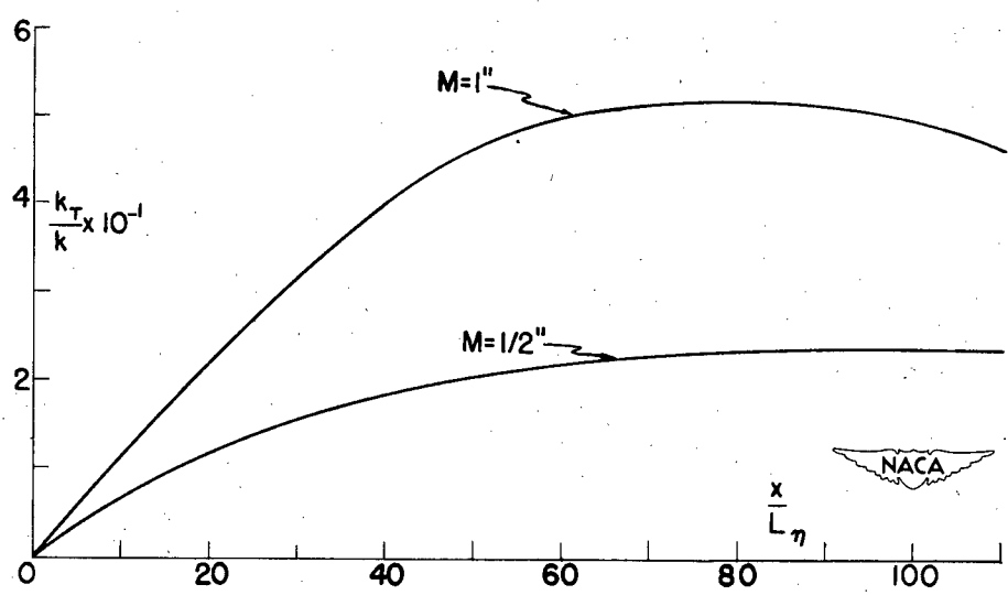
(b) Turbulent-heat-transfer coefficient for two different grids. \bar{U} = 25.6 feet per second and \frac{x_0}{M} = 43.4 .
