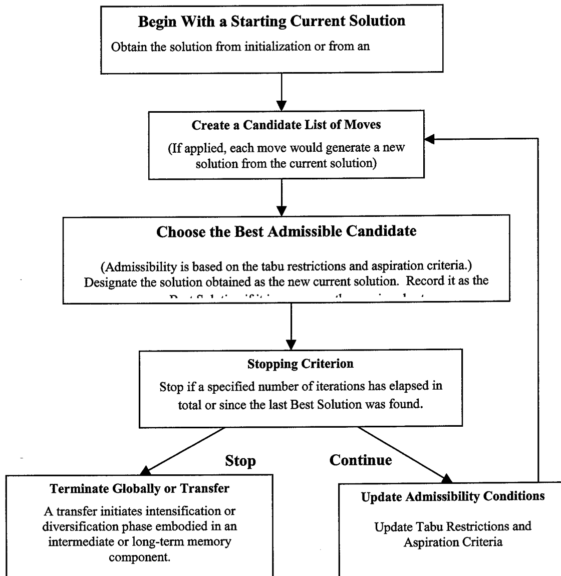
Figure 13. Common Steps in a Tabu Search [Glover, p. 78, 1990]
