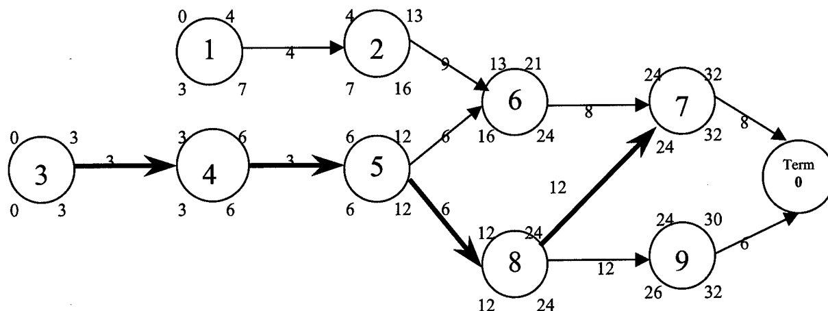
Figure 7. AON network for CPM example displaying ES,EF,LS,LF
