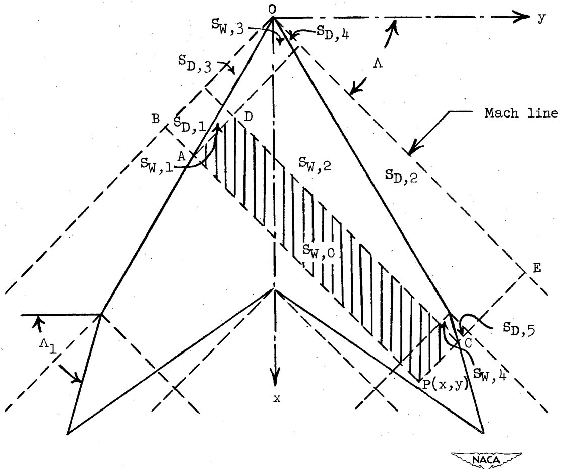
Figure 2.- Sketch of wing regions S_{W(0,\dots,4)} and external flow regions S_{D(1,\dots,5)} .
