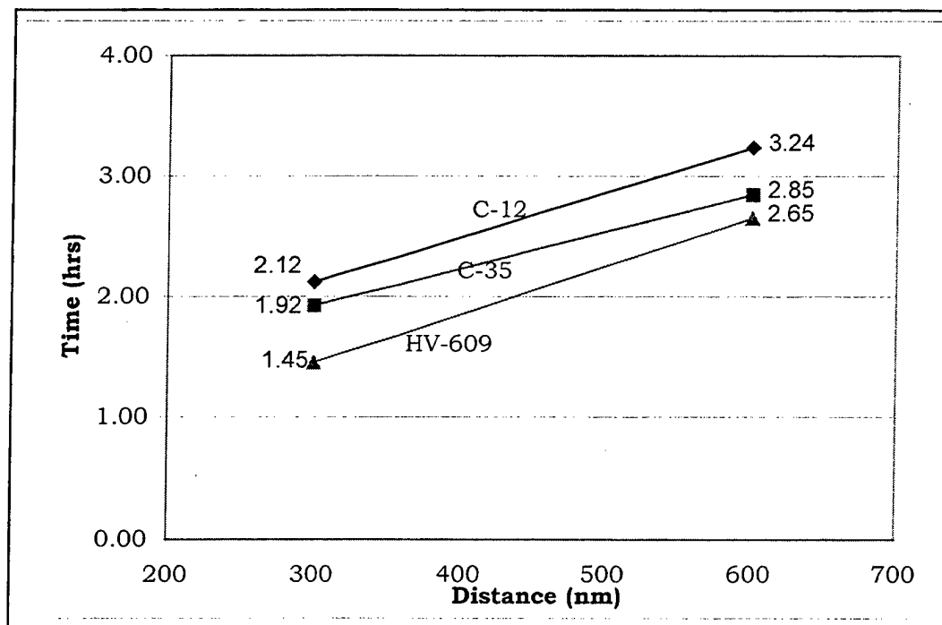
Figure 26. OSA Total Travel Time
