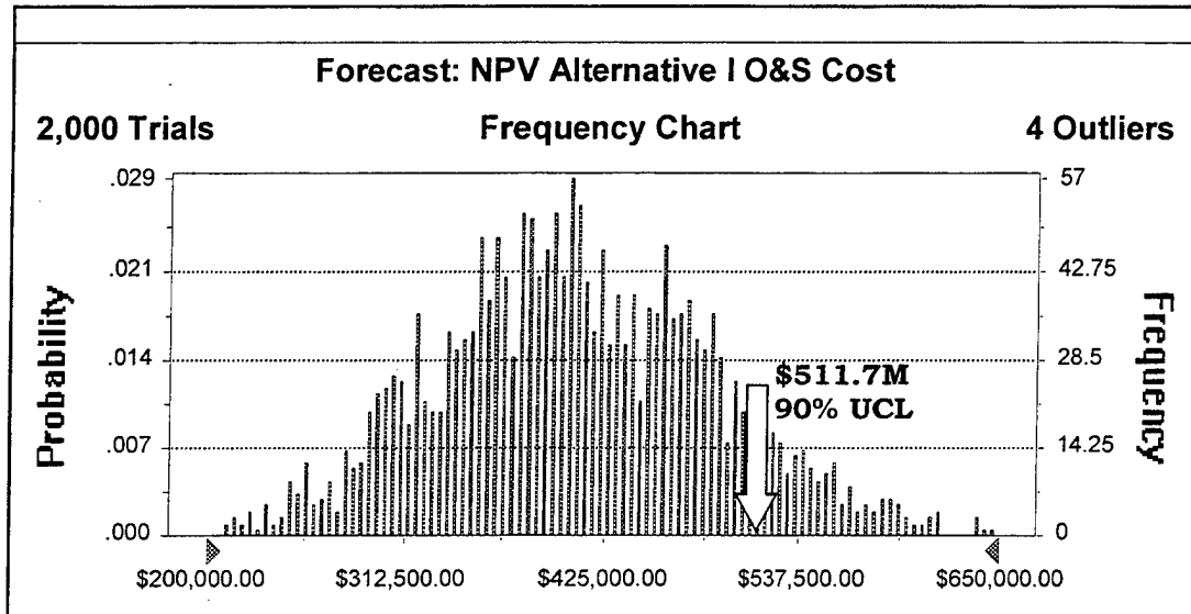
Figure 18. NPV of Estimated Alternative I Operating and Support Cost
