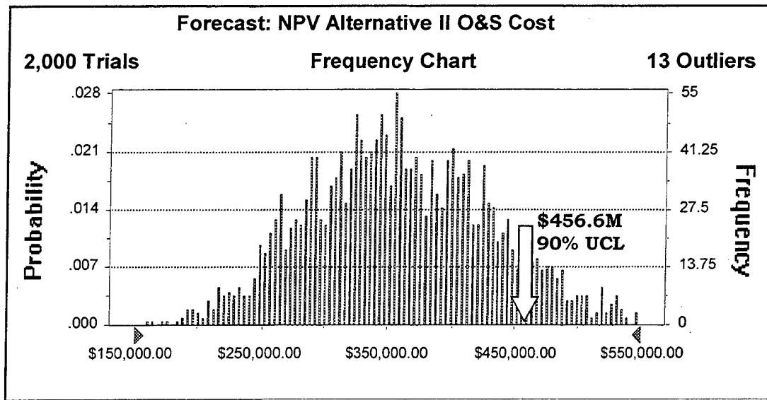
Figure 19. NPV of Estimated Alternative II Operating and Support Cost
