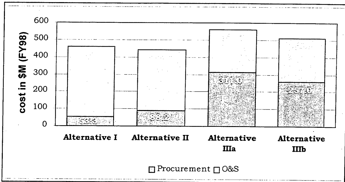
Figure 23. Comparison of Estimated 50th Percentile Total Cost
