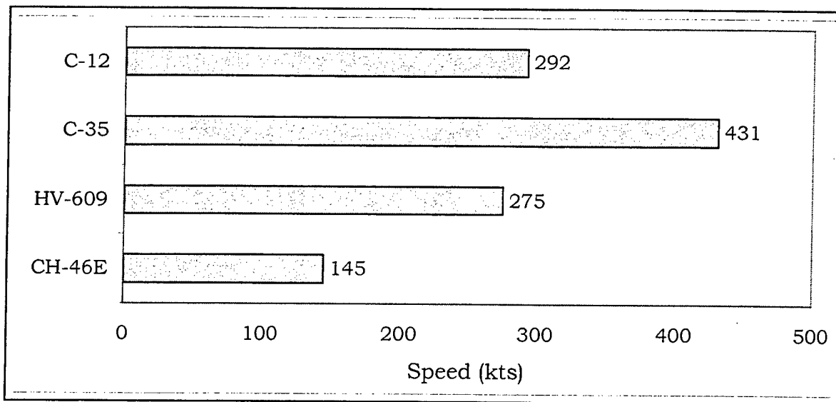
Figure 10. Maximum Cruise Speed Comparison
