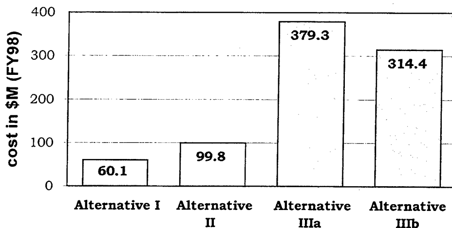
Figure 17. Comparison of Estimated Procurement and Conversion Cost
