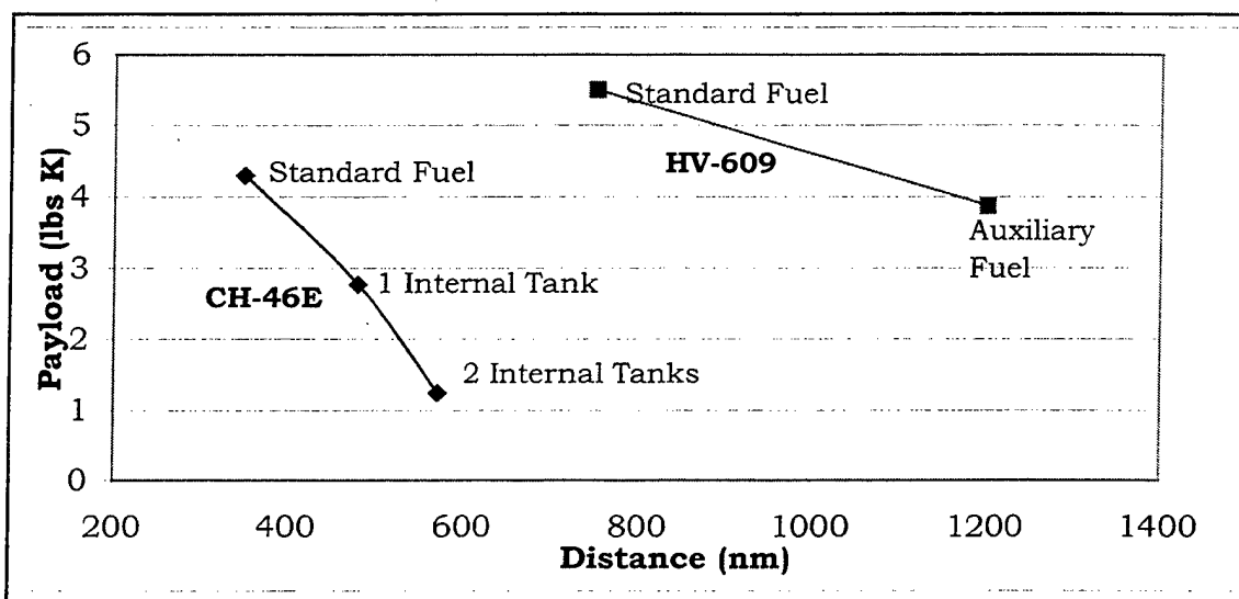
Figure 28. Payload versus Range
