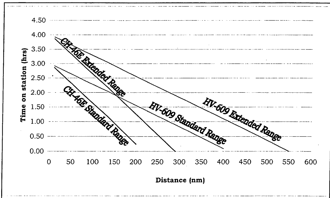
Figure 27. SAR Range versus Time on Station
