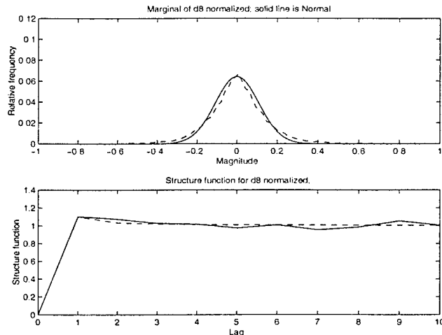
Figure 4.4: The top plot shows the empirical distribution of d_s . The solid line is a Gaussian distribution. The bottom plot shows the correlation of these wavelet coefficients. The dashed line is the theoretical correlation for fBm with H = 1/3 .
