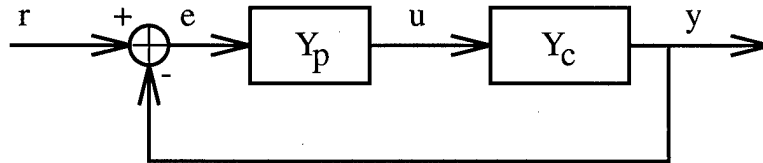
Figure 2.4 Pilot/Vehicle Closed Loop System
