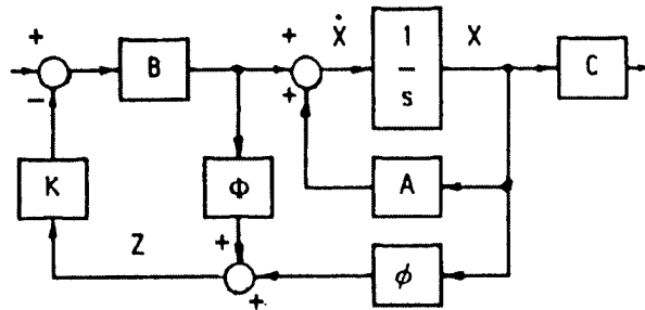
Figure 2.21 State Predictor System Diagram from Sobiski and Cardullo (52)
