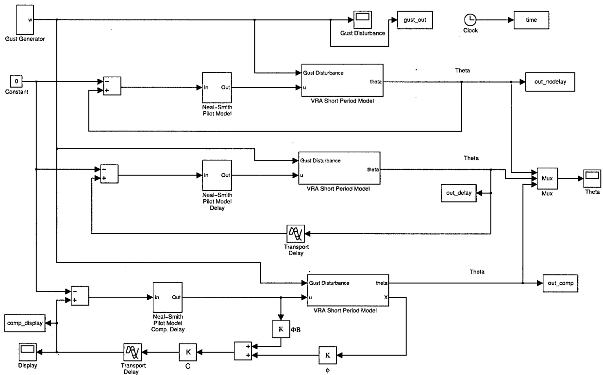
Figure 3.72 VRA Gust Rejection Model, Full State Predictor Compensation
