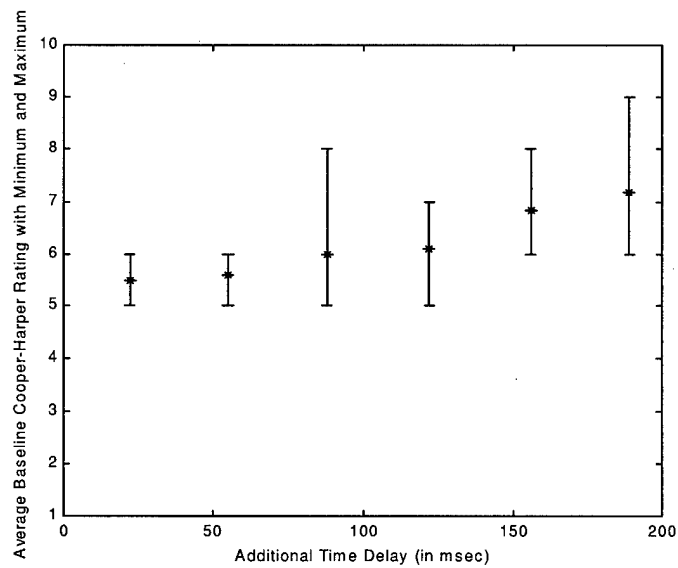
Figure 3.14 NASA UAV Flight Test Results
