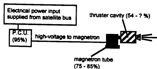
Fig. 1: System illustration with component efficiencies.
