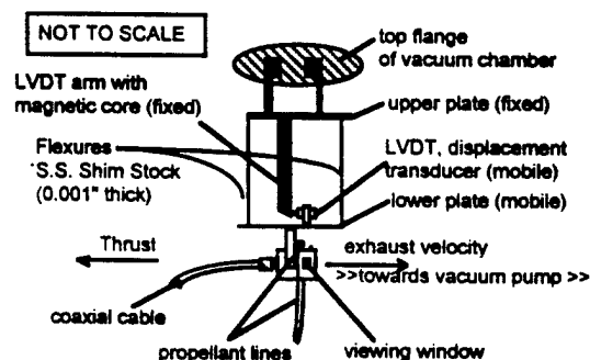
Fig. 6: Pendulum thrust stand
