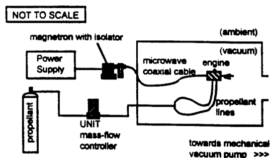
Fig. 5: Experimental setup.
