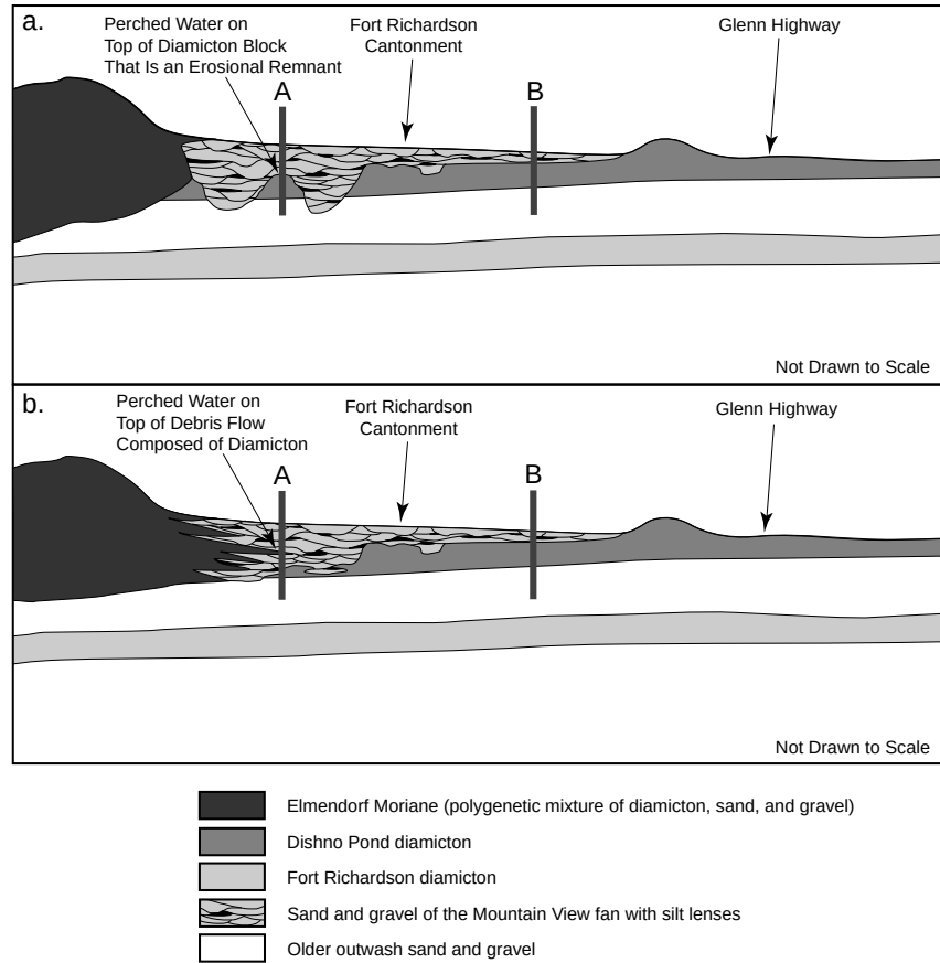
Figure 17. Proposed stratigraphy below the Fort Richardson cantonment. Erosive activity (a) during deposition of the Mountain View fan cut through the Dishno Pond ground moraine and edges of the Elmendorff Moraine. Erosion and deposition (b) associated with the Mountain View fan was accompanied by sediment failure along the margin of the Elmendorf Moraine, producing an interstratification between sand and gravel and diamicton. Wells drilled at site A would encounter a diamicton at an elevation roughly equivalent to the top of the diamicton encountered in well B.
