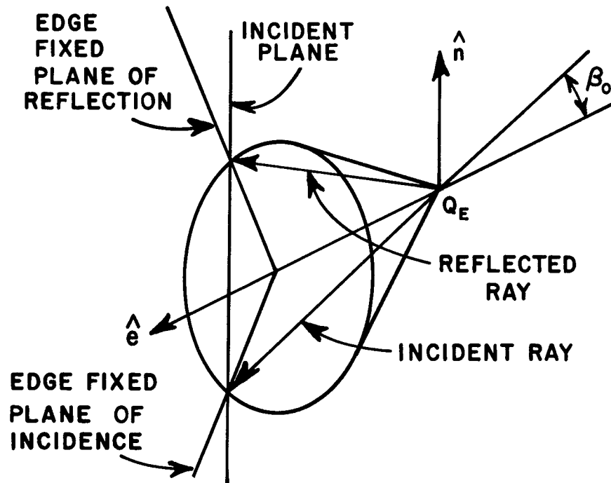
Fig. 9. Edge fixed plane of incidence and reflection.
