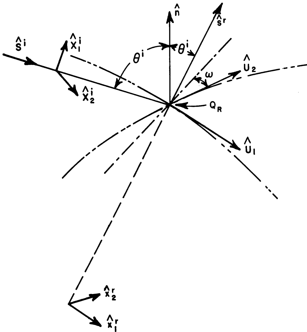
Fig. 2A. Geometry for the analysis of the reflected wavefront. The reflecting surface is S . ----- Intersection of a principal plane of S at Q_R with S ----- Intersection of the plane of incidence with the plane tangent to S at Q_R ----- Extension of the reflected ray below S .
