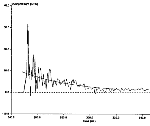
d) Overpressure P2
