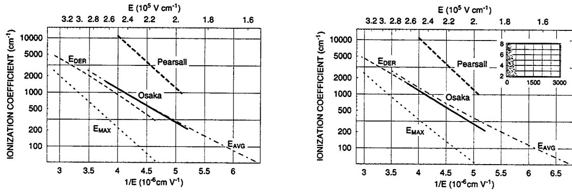
Fig. 13 Thick lines: Referenced hole impact ionization coefficients — Osaka et al. [9] ---- Pearsall [16] - - - - - average field — — — derivative - - - - maximum field In the inset is shown the extension of the dead space region compared with the total collector width Left: neglecting dead-space effects Right: considering dead-space effects
