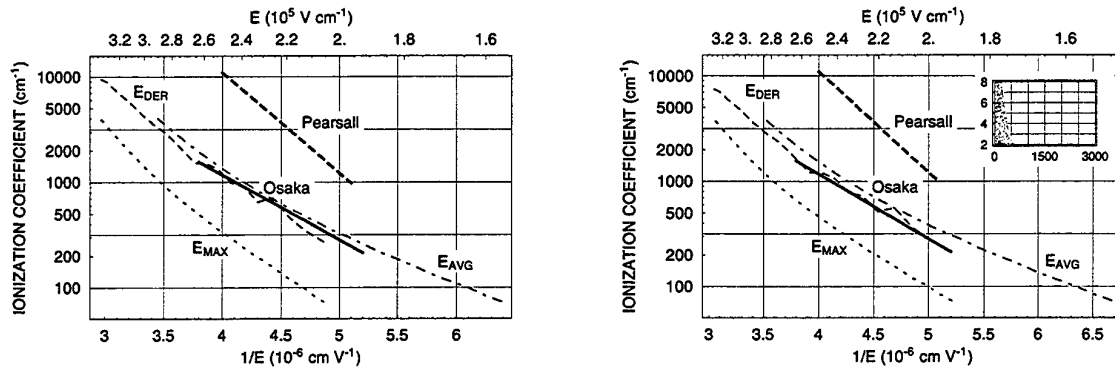
Fig. 16: Hole impact ionization coefficient for HBT JP3A Emitter area: 5 \times 10 \mu\text{m}^2 I_{C_{safe}} : 25mA I_{C_{max}} : 100mA left: neglecting dead space and Kirk effects right: taking into account dead space and Kirk effects In the inset is shown the extension of the dead space region compared with the total collector width - - - - our results - - - - average field - - - - maximum field ——— Osaka et al. [9] - - - - Pearsall [16]
