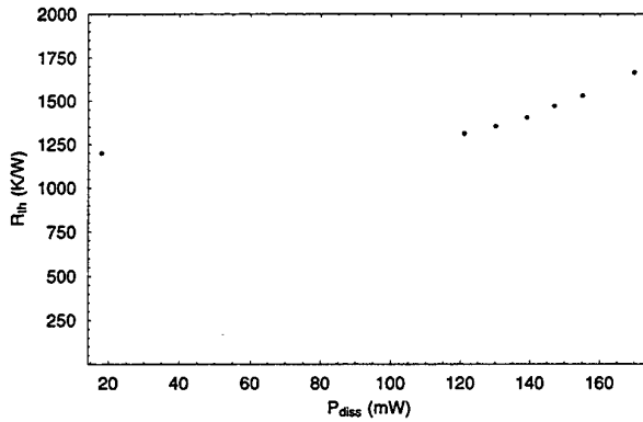
Fig. 18: Measured [18] thermal resistance at a constant base current ( I_B = 3 \text{ mA} ) for an HBT JP3A Emitter area: 5 \times 10 \mu\text{m}^2 I_{C_{safe}} : 25mA I_{C_{max}} : 100mA. Our data are summarized in the left-most point.
