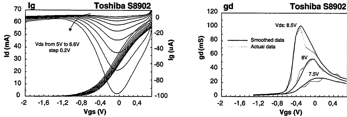
Figure 17: Left: gate current I_g in a Toshiba S8902 AlGaAs/GaAs measured as a function of V_{gs} with constant V_{ds} (from V_{ds} = 5\text{V} to 6.6\text{V} ; DC measurements). Right: Output conductance g_D = dI_D/dV_{DS} in the same device, measured at high V_{DS} (from V_{DS} = 7.5\text{V} to 8.5 ; 500\text{ns} TLP measurements) in on-state breakdown conditions.
