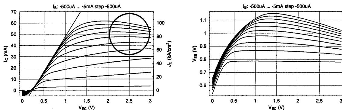
Fig. 2: HBT JP2C Emitter area: 2 \times 30 \mu\text{m}^2 I_{C_{safe}} : 30mA I_{C_{max}} : 120mA
