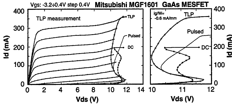
Figure 7: Left: TLP I_d vs V_{ds} in the tested GaAs MESFETs. I_d curves are truncated by the I_d - BV_{ds} locus at constant I_g = -300 \mu A , extrapolated from the I_g vs V_{gs} characteristics (not shown). TLP, pulsed and DC I_d - BV_{ds} locus at constant I_g = -300 \mu A measured as in [8] (right) are also depicted.
