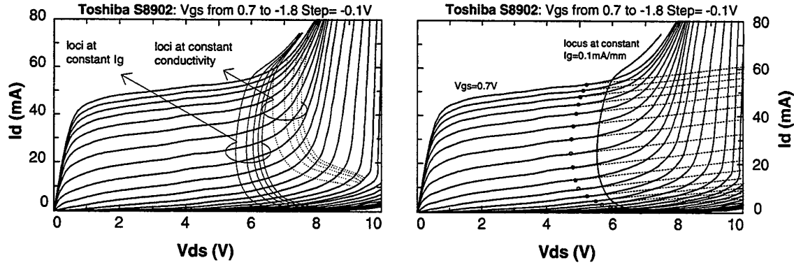
Figure 16: Left: comparison between the loci at constant gate current (from 0.1\text{mA/mm} to 0.5\text{mA/mm} , step 0.1\text{mA/mm} ) and the loci at constant conductivity (from 150\text{mS} to 350\text{mS} , step 50\text{mS} ). The I_d vs V_{ds} curves were obtained by sampling TLP pulses at 50\text{ns} . Right: comparison between a locus at constant current gate ( 0.1\text{mA/mm} ) and the points in which the I_d vs V_{ds} curves deviate from linear behavior. The I_d vs V_{ds} curves were obtained by sampling TLP pulses at 50\text{ns} .
