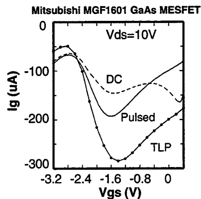
Figure 8: DC, pulsed and 500 ns TLP I_g vs V_{gs} in the tested GaAs MESFETs at fixed V_{ds} = 10 \text{ V} .
