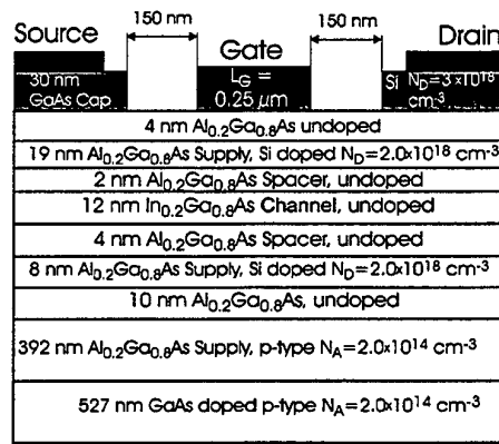
Figure 22: Schematic cross section of the simulated double heterojunction HEMT
