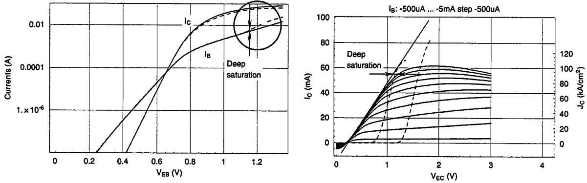
Fig. 7: HBT JP2C Emitter area: 2 \times 30\mu\text{m}^2 I_{C_{\text{safe}}} : 30mA I_{C_{\text{max}}} : 120mA Left: Gummel plot for V_{BC} = 0.5 V ——— and for V_{BC} = 0 V - - - Right: Common emitter output characteristics
