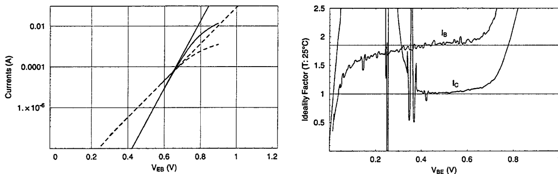
Fig. 3: HBT JP2C Emitter area: 2 \times 30 \mu\text{m}^2 I_{C_{safe}} : 30mA I_{C_{max}} : 120mA Left: ——— collector current - - - - base current
