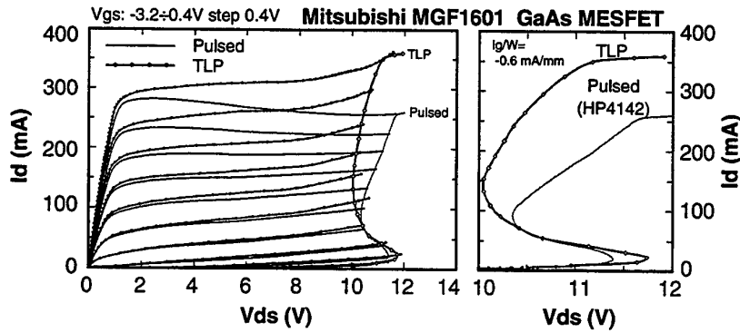
Figure 5: Left: pulsed and TLP I_d vs V_{ds} in the tested GaAs MESFETs (Mitsubishi MGF1601). Curves are truncated by the I_d - BV_{ds} locus at constant I_g = -300\mu\text{A} , extrapolated from the I_g vs V_{gs} characteristics (not shown). Right: pulsed and TLP I_d - BV_{ds} locus at constant I_g = -300\mu\text{A} measured as in [8].
