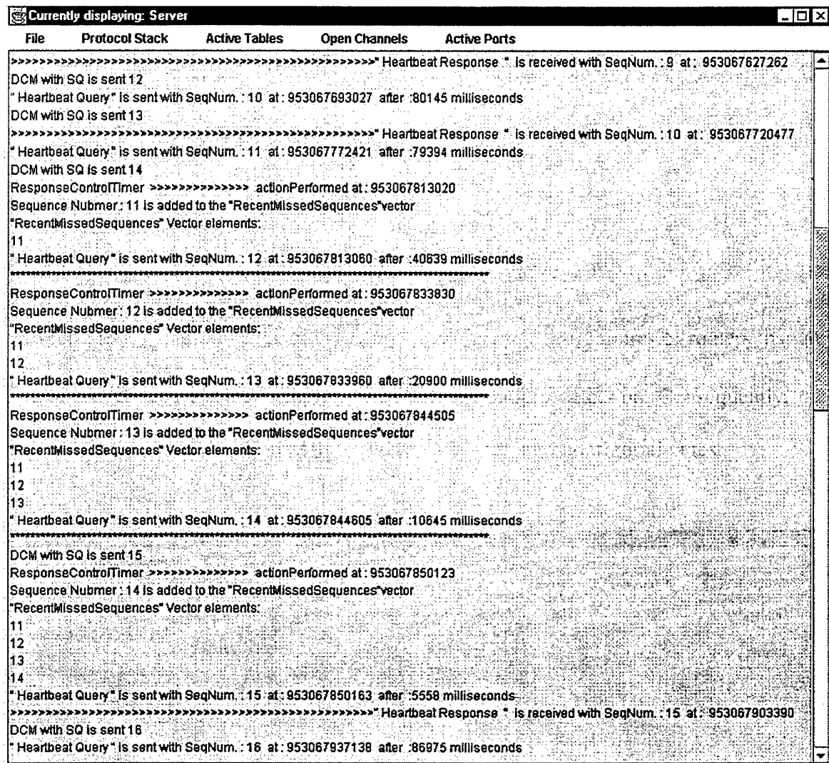
Figure 5.44. The Backup Server GUI During Control Channel Auto-Configuration Test.
