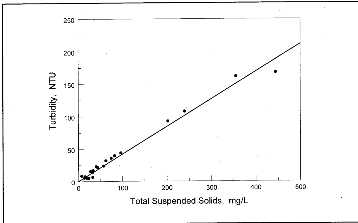
Figure 2. Laboratory column data showing relationship of turbidity and TSS for Middle Ground Island sediment
