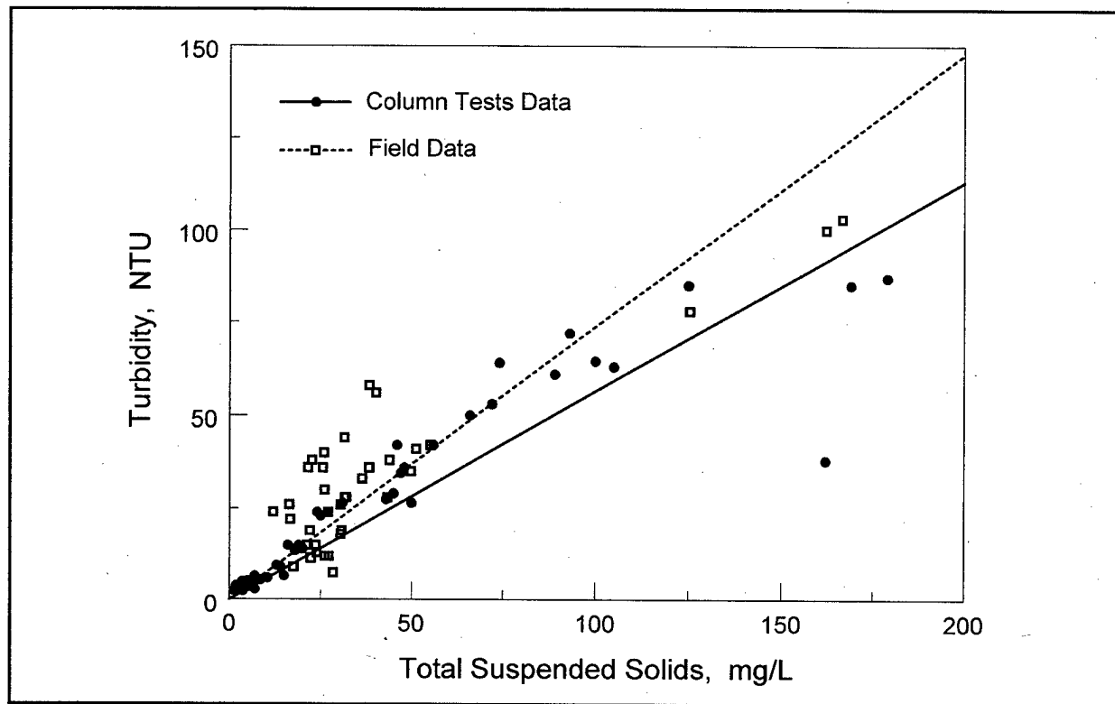
Figure 1. Comparison of laboratory column and field data and linear regression lines for Mobile Bay sediment
