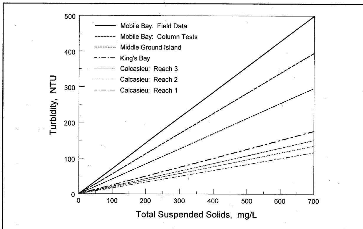
Figure 3. Combined regression plots, showing differences among lines for different sediments
