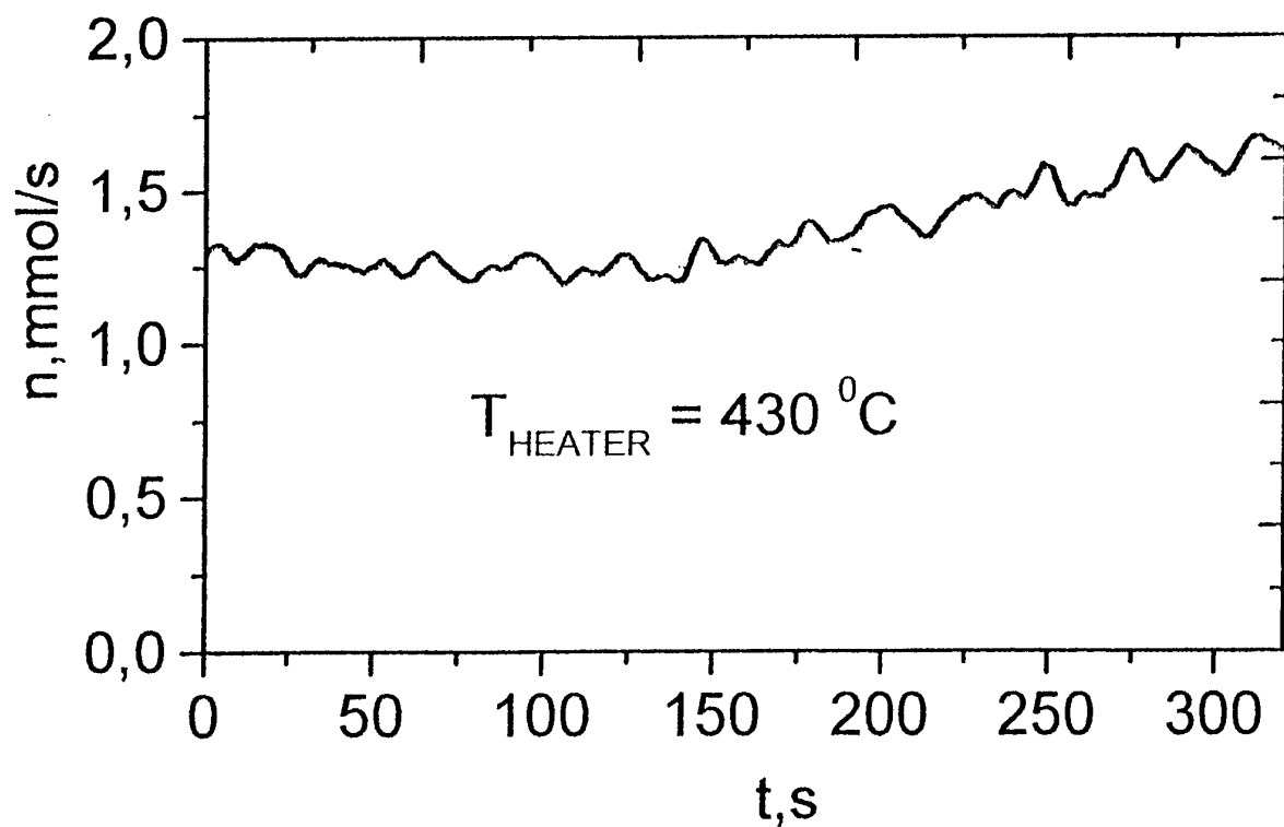
Fig.5 : Plot of \text{I}_2 flowrate on time
