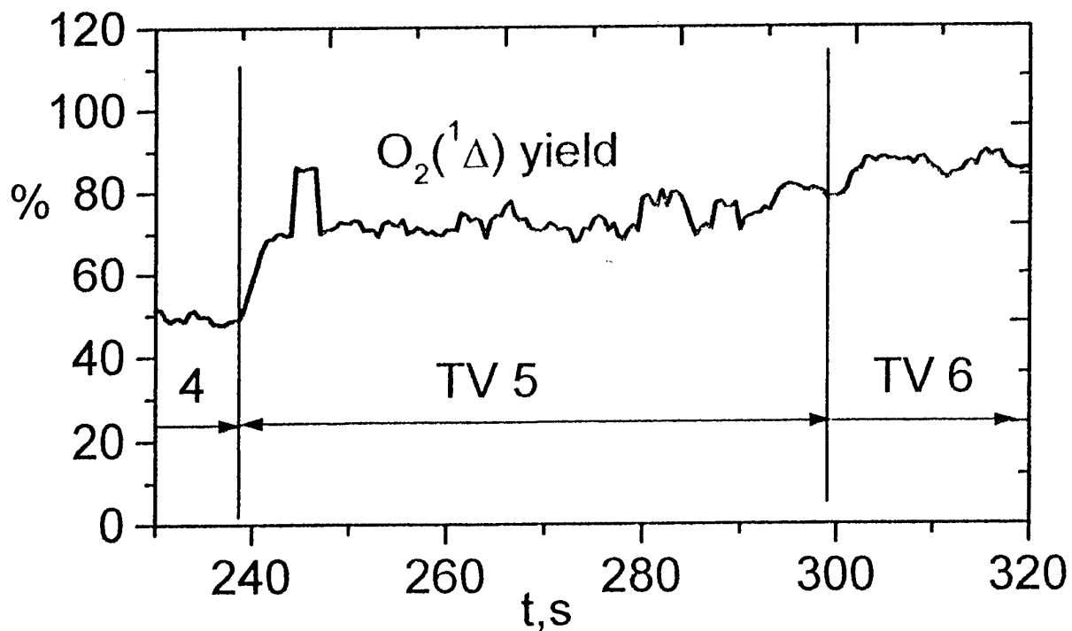
Fig.2a,b : Generator and subsonic channel pressure and O_2(^1\Delta) yield on time (prim.He into chlorine)
