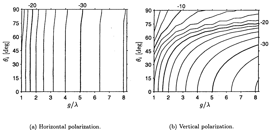
Fig. 5. Relative RMS error [dB] at z = 0 for the tapered wave introduced in this paper.
