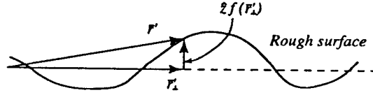
Fig. 2. The local position vector \bar{r}' on a rough surface is the sum of the horizontal and vertical components.
