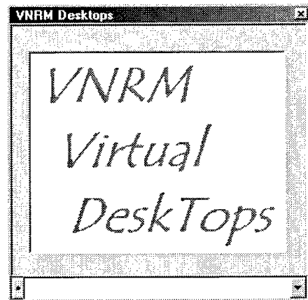
Fig. 8–VNRM Desktops interface
