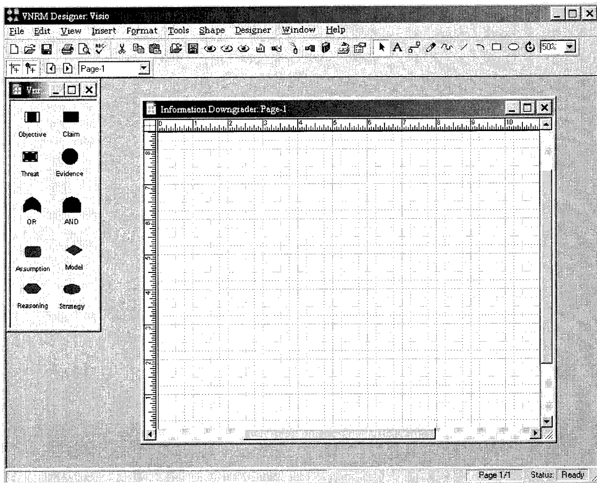
Fig. 6–VNR Designer interface
