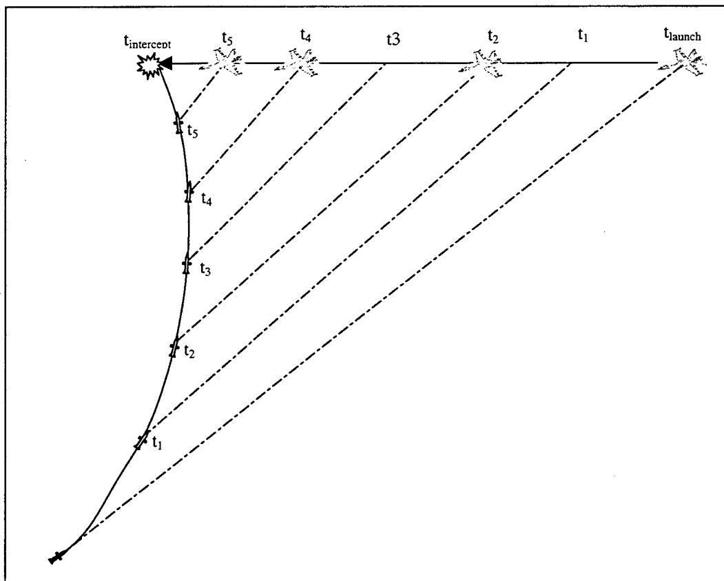
Figure 5. Proportional Navigation Flight Trajectory
