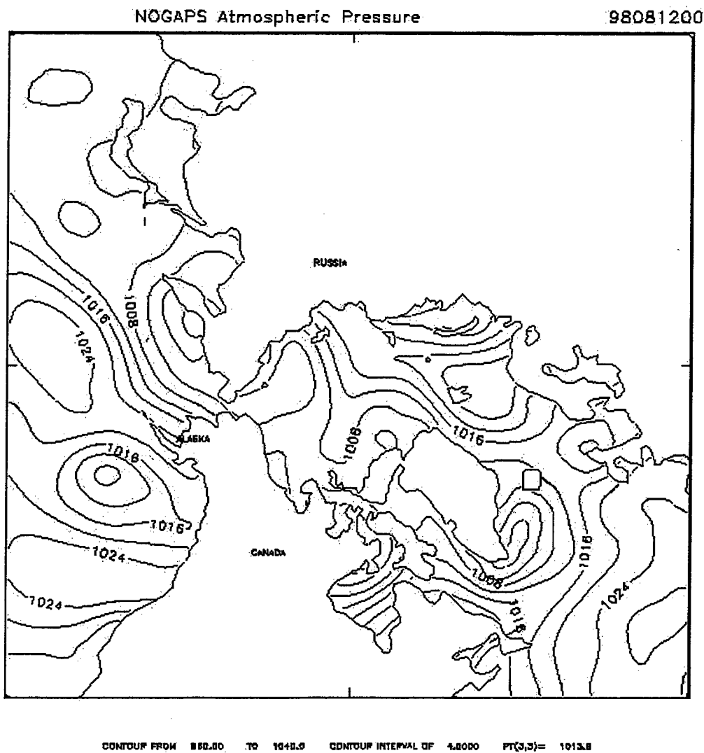
Figure 27. Atmospheric surface pressure chart for the first summer noise event (12 Aug 98). Note the presence of a weak low pressure trough extending from the Kamchatka Peninsula into the SHEBA region creating moderate (6-8 m/s) wind speeds and inducing a wind direction change.
