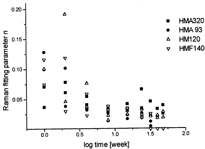
Figure 4: Time dependence of the Raman parameter n from the DS measurements
