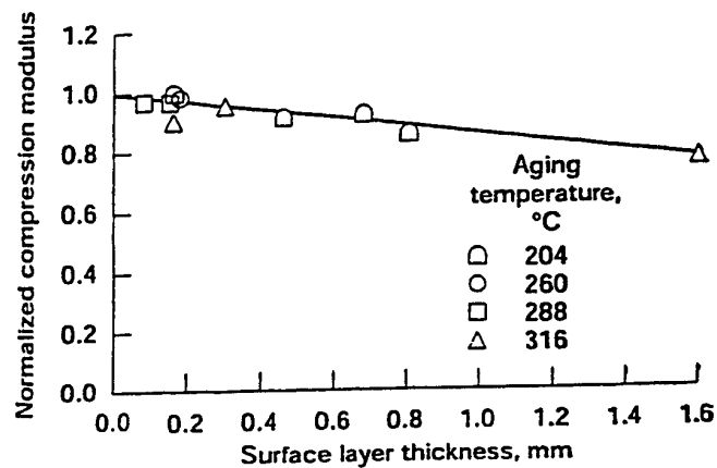
Figure 8. Composite compression modulus as a function of surface layer thickness at various temperatures. Number of plies, 20.
