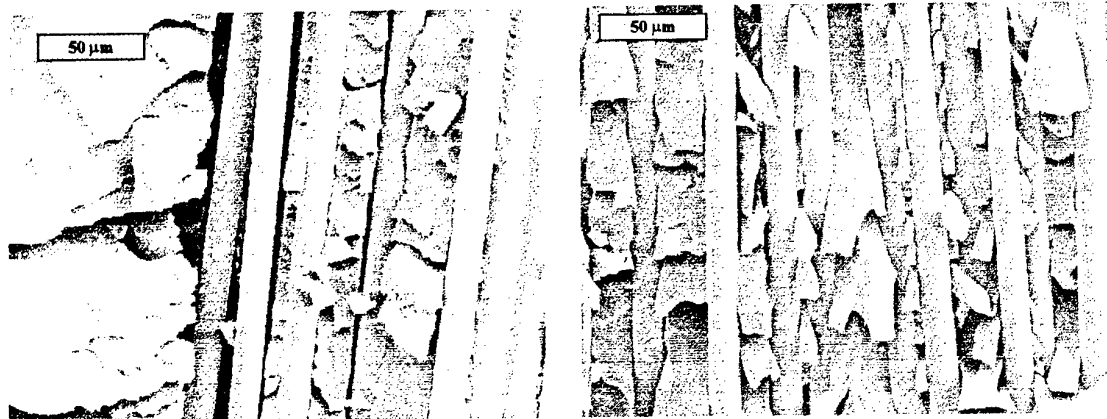
Figure 3. Sample cured at 20°C, 2160 h aged. X500
