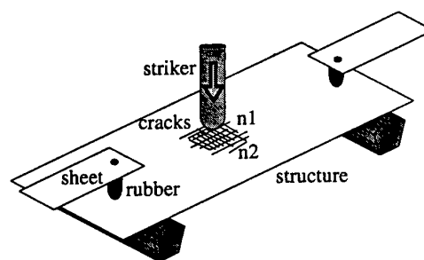
Figure 2. Boundary conditions.
