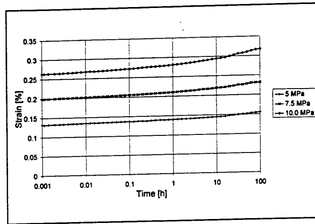
Figure 4: Creep curves of pin loaded non-reinforced polymer specimens
