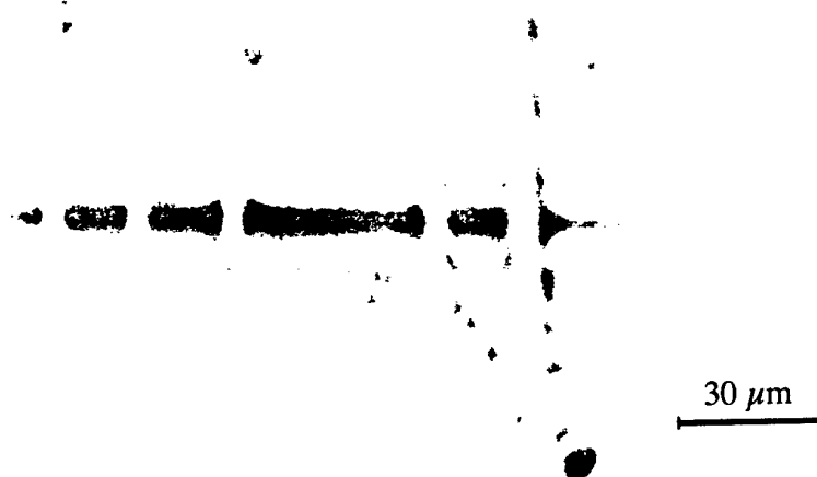
Figure 1. Fibre-bridged crack in fatigue of carbon fibre/epoxy at \epsilon_{\max} = 1.1\% and 10^3 cycles
