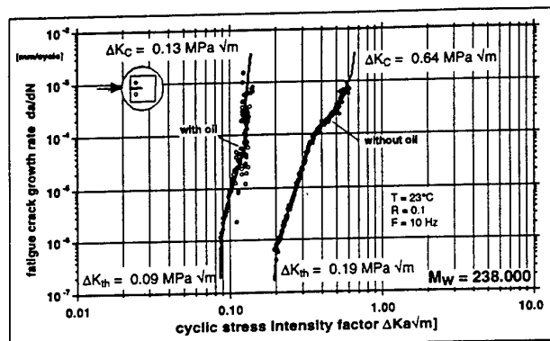
Figure 3. FCP with and without a stress cracking media - PS 148H.
