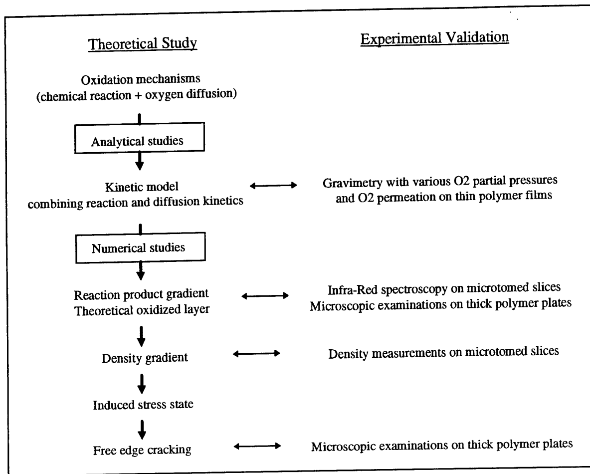
Figure 1 : Methodology followed for studying the polymer oxidation.
