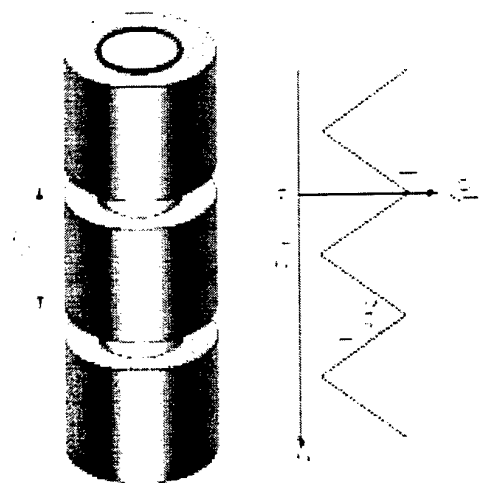
Figure 1.- Schematic representation of model unidirectional composite and axial stress profile for fibers.
