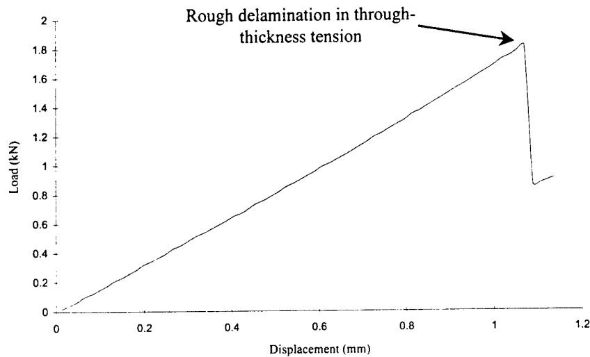
Fig 6 : Tension test of 0° curved beam specimen.
