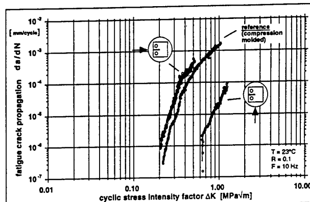
Figure 5. Molecule orientation effects on crack propagation - PS 148H.
