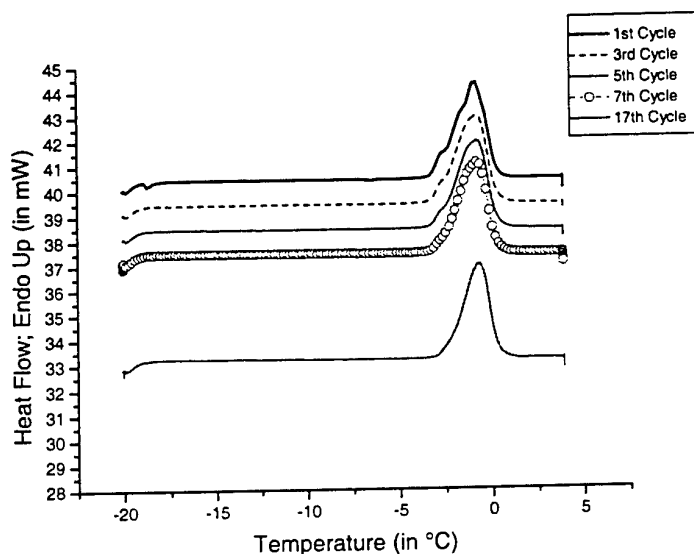
Figure 3: Cyclic DSC data on the composite specimen. The pan contained both the saturated specimen as well as a few drops of free-water.
