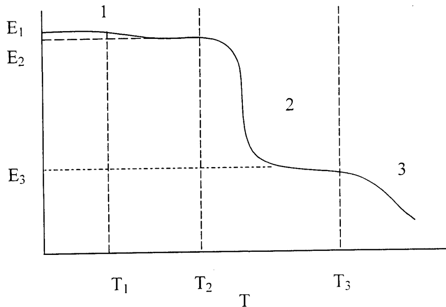
Figure 3 Schematic diagram of the variations of instantaneous stiffness of polymers across transitions in properties.
