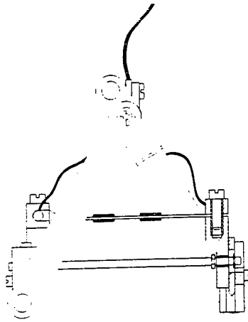
Figure 2: Extensometer
