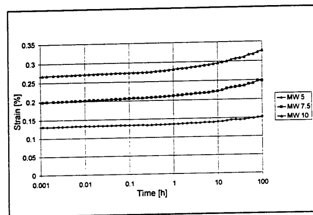
Figure 5: Creep curves of the non reinforced polymer (rectangular specimens)
