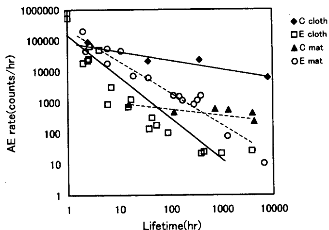
Fig. 5 Relationship between AE rate and lifetime
