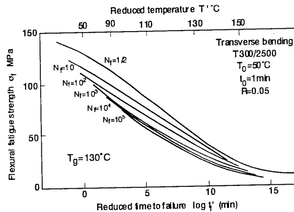
Fig.6 Master curves of fatigue strength under three types of loading
