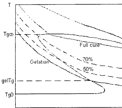
Fig5: Time-Temperature-Transformation Diagram
