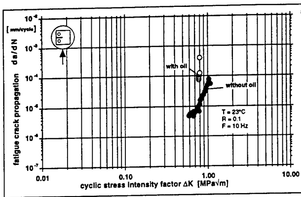
Figure 6. Injection molded samples tested perpendicular to the injection direction - PS 168N.
