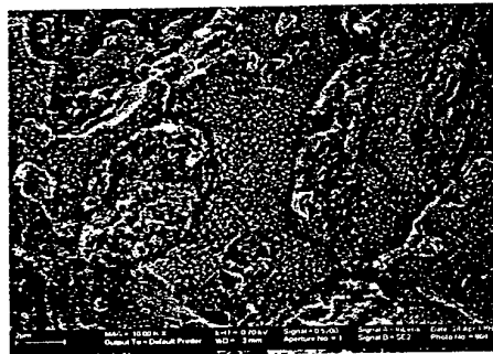
Figure 10. FCP fracture surface of PS 486M tested under oil environment.
