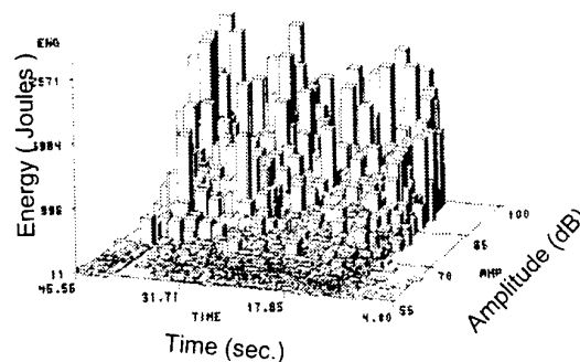
Figure 3. Amplitude, energy and time plot of acoustic emission data under tensile loading.
