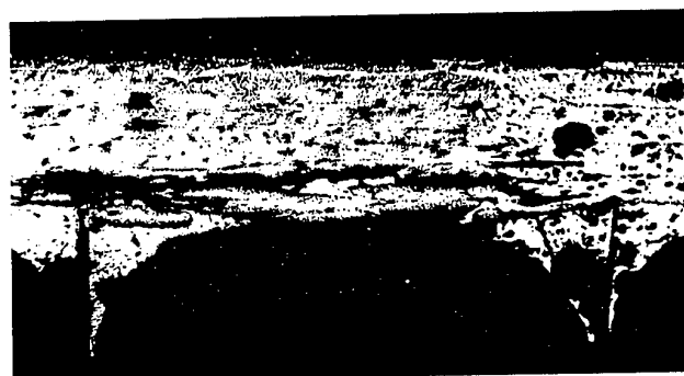
Figure 5. Photomicrograph of a fiberglass core bay impacted with 4.1 J at 25X magnification.
