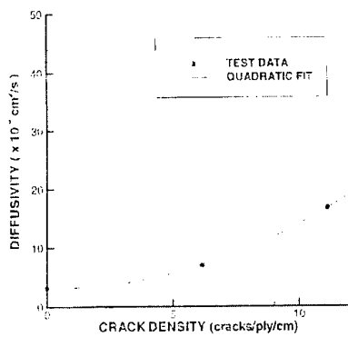
Figure 2. Change in Diffusivity with Micro-crack Density
