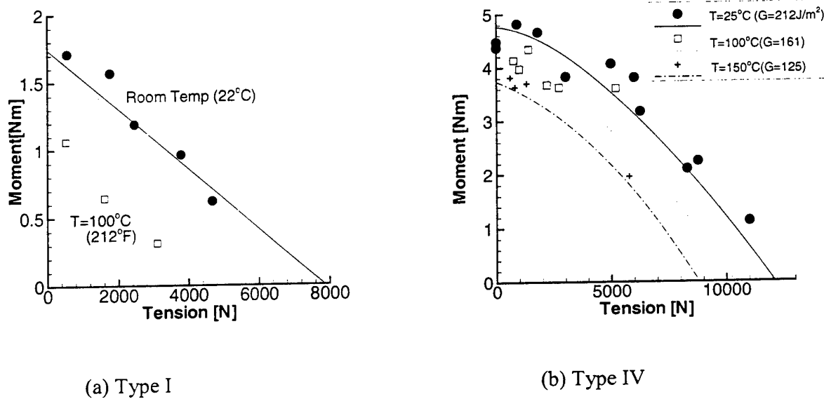
Figure 2. Moment-tension interaction at failure initiation for Type I and IV specimens
