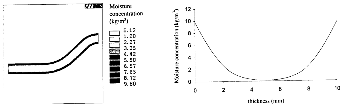
Fig 5 : Example of moisture concentration profile ( \text{kg/m}^3 ) along the specimen thickness after a 3000 hours conditioning.
