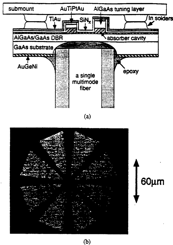
Fig. 14. (a) Schematic cross section of a bottom-illuminated multiple-channel resonant-cavity Schottky photodetector array with the Burrus-type packaging configuration. (b) A photograph of a finished eight-channel "pie"-shaped Schottky photodetector array.
