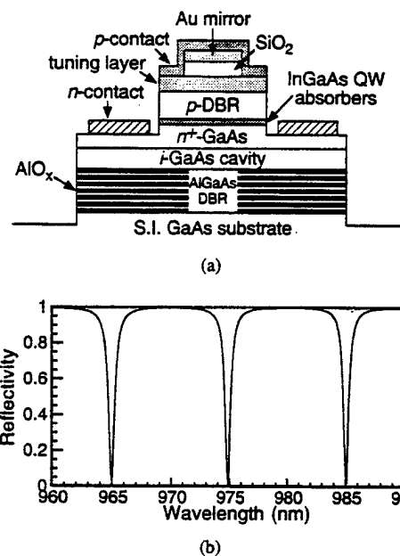
Fig. 16. (a) Schematic device cross section and (b) theoretical reflectivity spectra for the proposed P-i-N photodetector with an antiresonant oxide aperture underneath the ring p-contact to suppress undesired absorption which may cause linewidth broadening in photoresponses. The solid-curve reflection spectra shown from left to right are for positions under the Au back mirror with tuning layer thicknesses of 0.40 , 0.50 , and 0.62\lambda , respectively. The dashed curves are for positions under the ring p-contact with the above tuning layer thicknesses.
