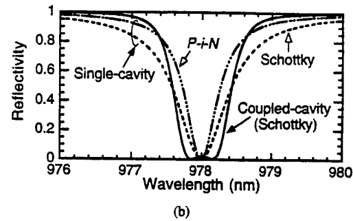
Fig. 18. A novel narrow-band coupled-cavity photodetector design proposed in our earlier work [42]. (a) Refractive index profile of a coupled-cavity Schottky photodiode design. (b) Comparison of the theoretical power reflectivity spectra for the single-cavity (both Schottky and p-i-n) and the coupled-cavity (Schottky) structures.
