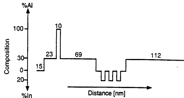
Fig. 11. A schematic of the undoped MBE grown structure used for IFVD using laterally oxidized AlAs. The QW region is the same as in Fig. 3. The surface is on the left.
