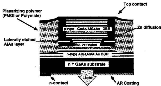
Fig. 6. Schematic of IID-VCL [40].
