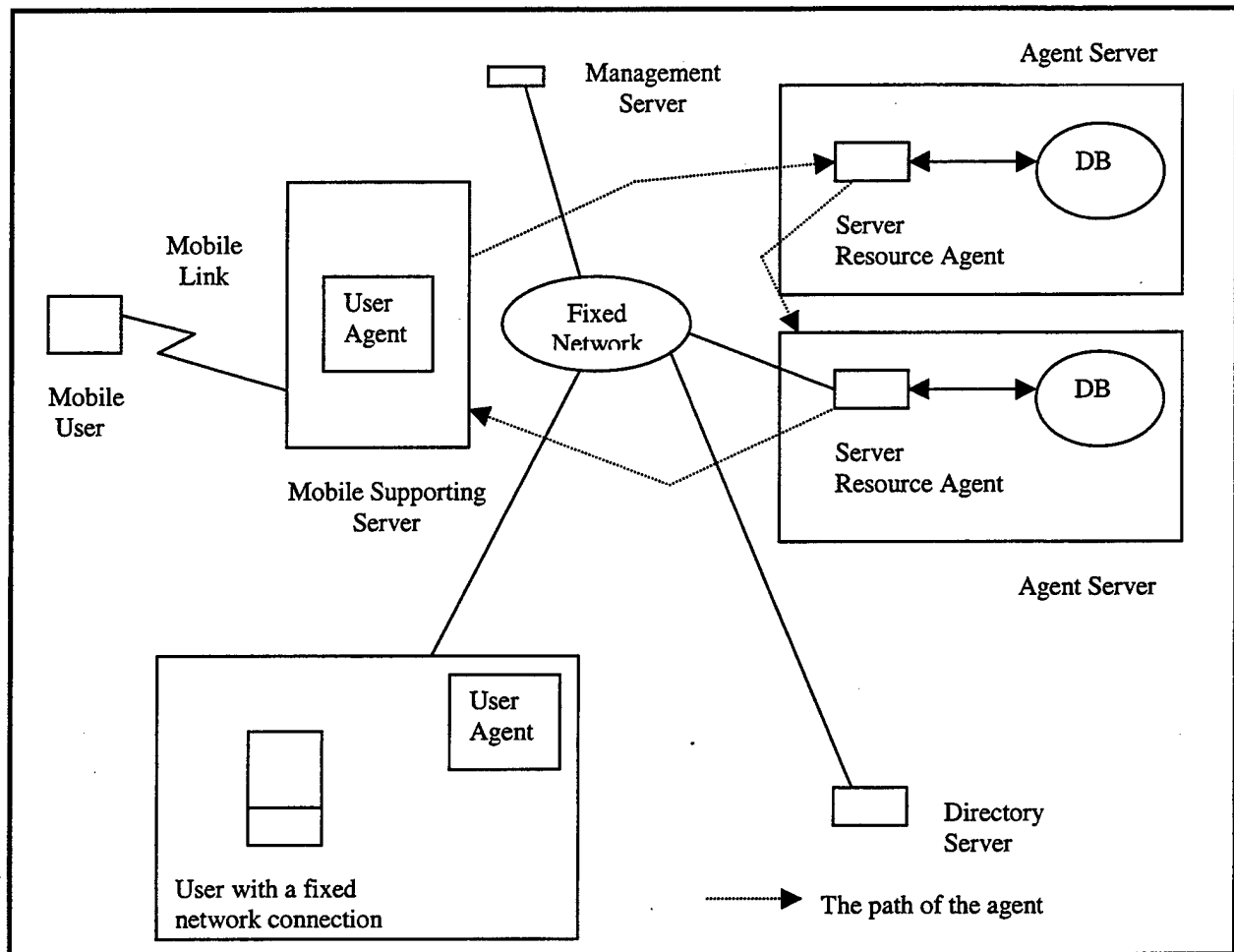
Figure 4.1: The Infrastructure of a Mobile Agent System. [From Ref. 29]
