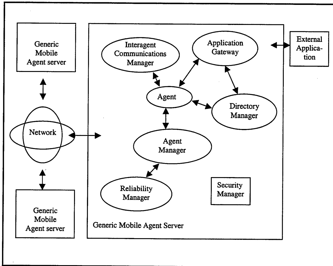
Figure 4.2: Generic Mobile Agent System Architecture. [From Ref. 19]
