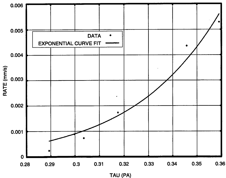
Figure 3. Erosion rate of 300- \mu m "Ottawa" test sand versus flow shear stress in channel.
