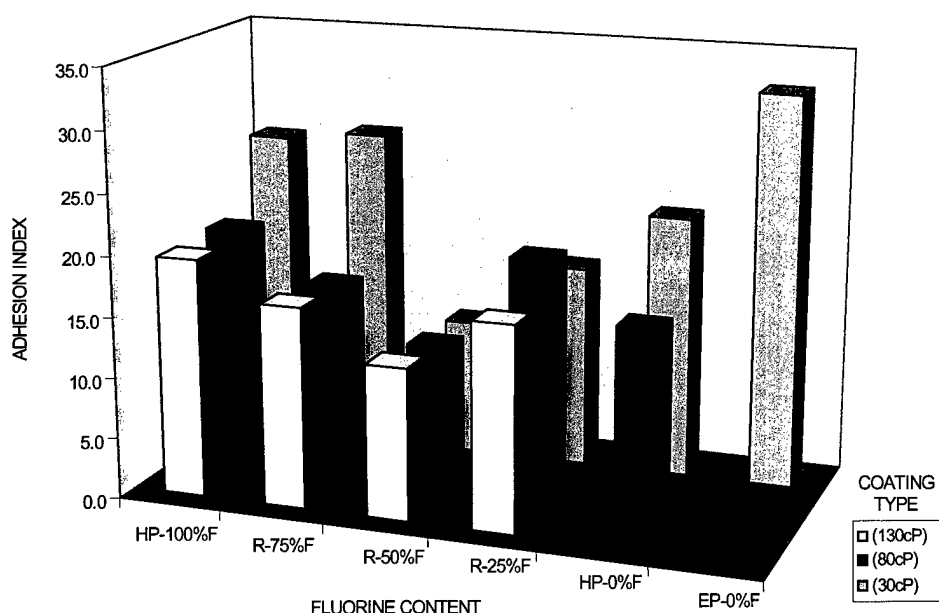
Figure 1. Ice-release properties of a low surface free energy coating series as a function of fluorine content (%F) for three types of coatings prepared with a design for varied coating crystallinity (30, 80, and 130 cP). A lower adhesion index indicates better ice-release.
