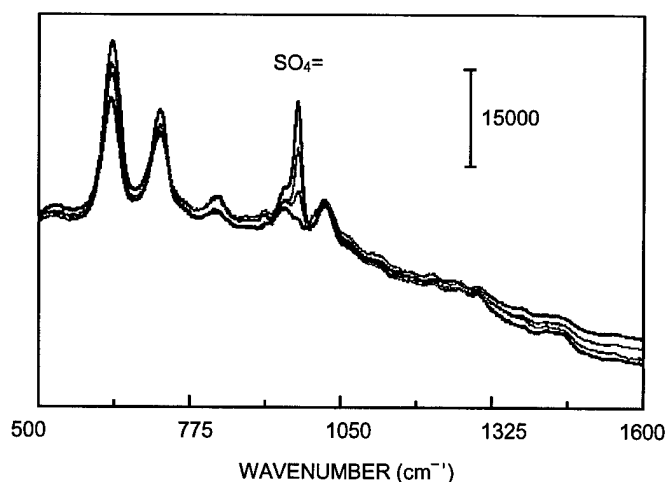
Figure 1. SERS response of cysteamine hydrochloride on silver as a function of sulfate concentration (0', 10', 100', and 2500-ppm sulfate).
