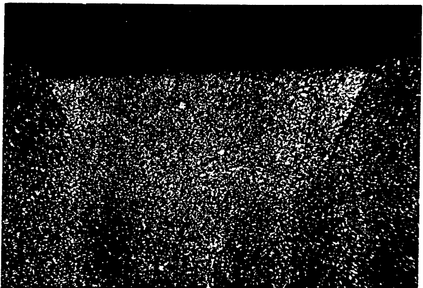
Fig.4.4. Macrostructure of specimen, loaded with energy 50,7 J. LM, x20 Fig.4.5. Macrostructure of specimen, loaded with energy 54,4 J. LM, x20 Fig.4.6. Macrostructure of specimen, loaded with energy 64,2 J. LM, x20
