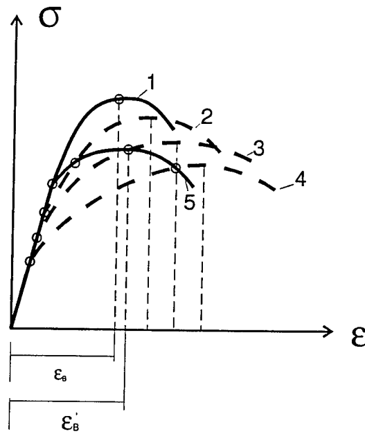
Fig.1.2. Shift of the critical strain \epsilon_c for materials sensitive to temperature.
