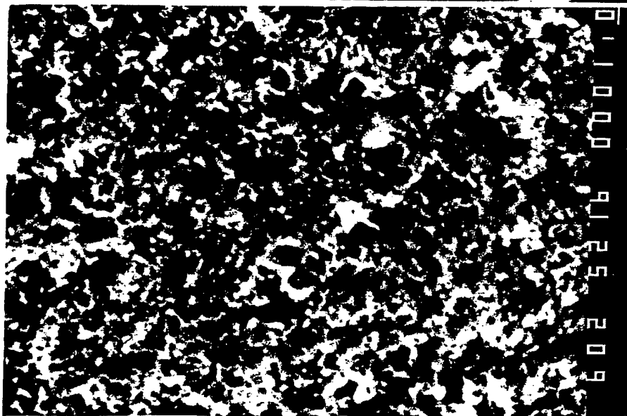
Fig.4.24. Etch-pits relief in the initial part of ASB in specimen, loaded with energy 54,4 J. Etching in 5% HNO 3 . SEM: a) x2000, b) x6000, c) x6000
