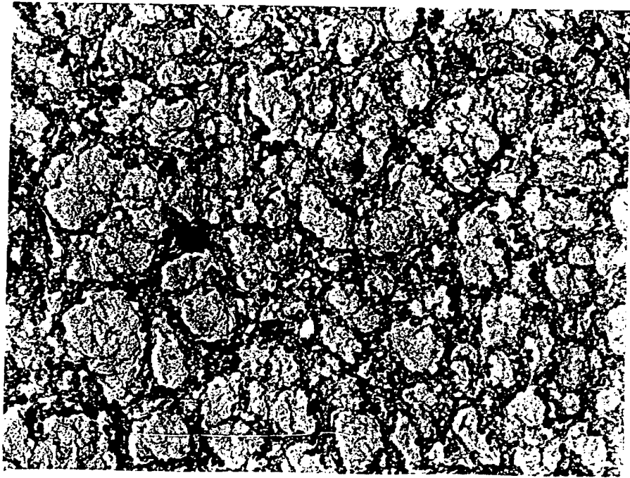
a) Fig.4.25. Cells in the initial part of ASB in specimen, loaded with energy 54,4 J. b) Etching in HCL:HNO 3 =1:3 solution. TEM replica: a) x6000, b) x20000
