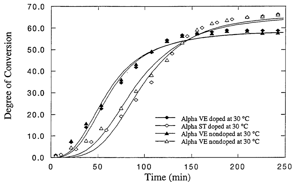
Figure 17. Degree of Conversion of VE and ST at 30 °C. Data Are Obtained Using T-FTIR. Markers Do Not Represent All Data Points Taken. Autocatalytic Curve Fit Is Shown as Solid Line.
