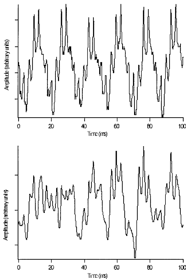
Figure 7. The AM on the Ar + pump laser (upper trace) and the frequency modulation waveform of the power spectrum of the Ti:Sapphire laser obtained by use of a spectrum analyzer as a frequency discriminator (lower trace).
