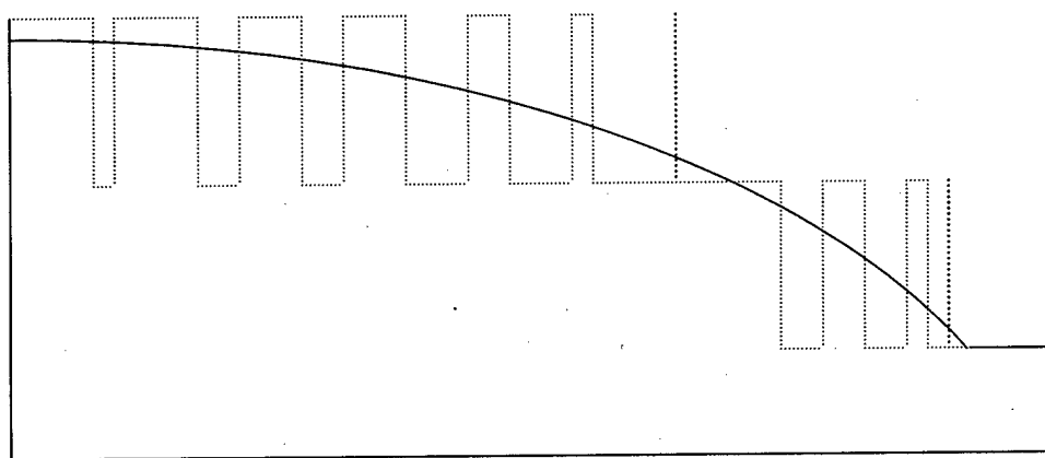
Figure 2.16. Combination multi-level and single-etch pre-form (side view); Before transport (dotted line) and after transport (solid line)
