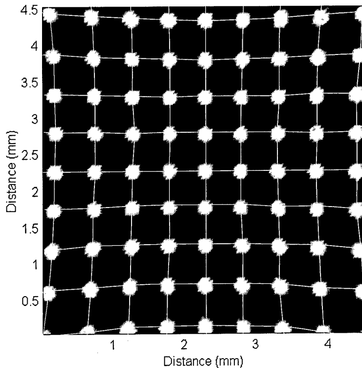
Figure 4.34. Image of clear aperture array through imaging system; simulation of distortion shown in system of Figure 4.28.
