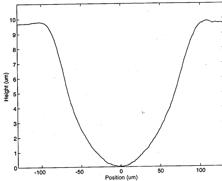
Figure 4.19. Profilometer trace through the center of a micromirror replicated in GaAs. The sag of the mirror is 9.7\text{ }\mu\text{m} .
