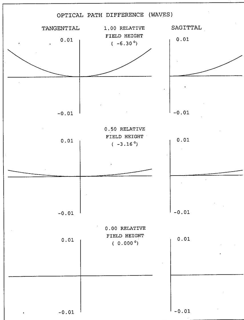
Figure 4.33. OPD calculation for steered beams (three object field points).
