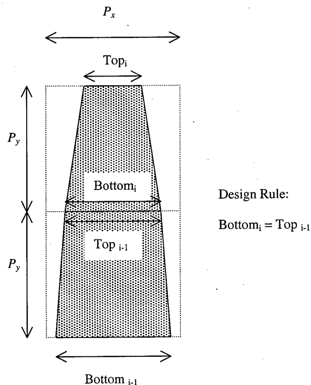
Figure 2.9. Trapezoidal one-dimensional pre-form method (top view)
