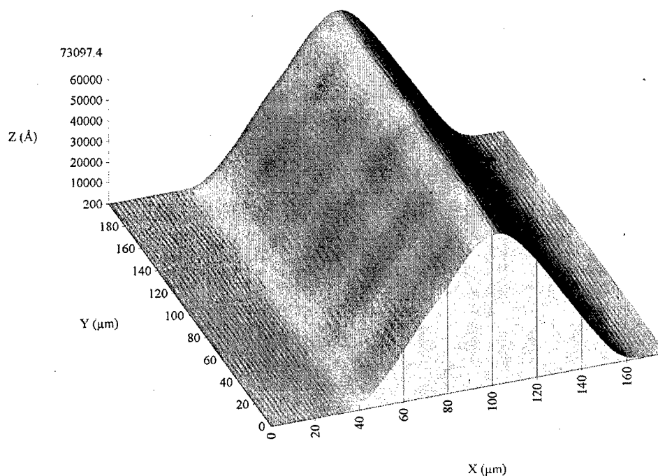
Figure 4.17. Profilometer measurement of a biprism, originally fabricated in GaP by mass-transport and subsequently cast into a thin polymer film. The height of the prism is 7.3\text{ }\mu\text{m} .
