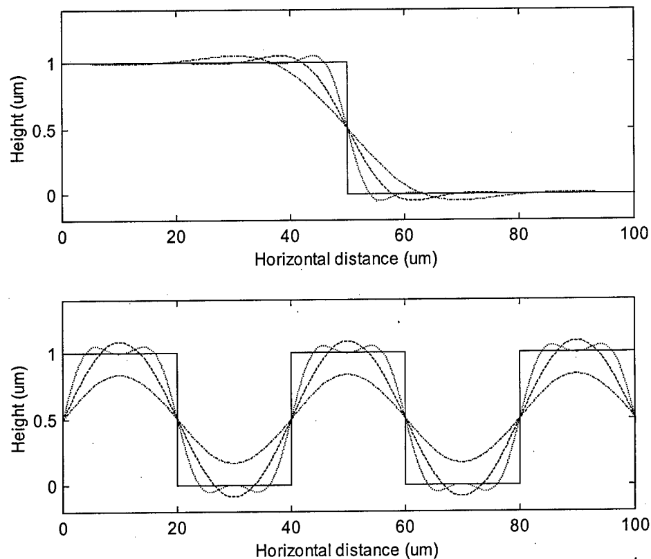
Figure 2.1. Simulated mass-transport smoothing of a vertical step (a) and square-wave grating (b); profile after zero (solid lines), 0.5 hours (dotted), 8 hours (dashed), and 64 hours (dot-dash).
