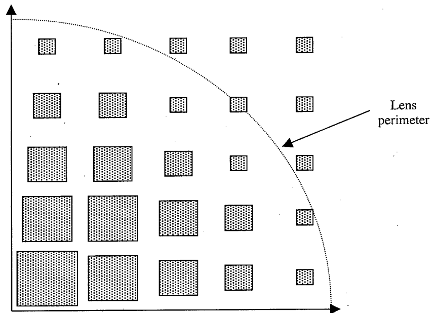
Figure 2.12. Design of convex lens using 2-D fill-factor modulation and reduced (20 – 80%) height range with square pixels (top view of one quadrant)
