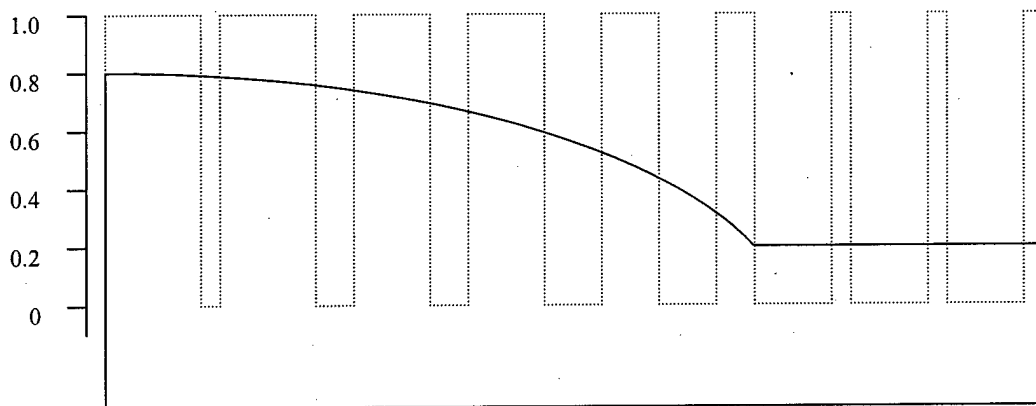
Figure 2.10. Reduced height range (20 - 80% of etch depth) for larger features (side view); before transport (dotted line) and after transport (solid line).
