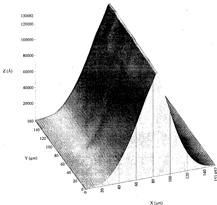
Figure 4.18. Profilometer measurement of the same biprism shown in Figure 4.17, but after transfer into GaAs. The height of the etched prism is 13.1 \mu\text{m} .
