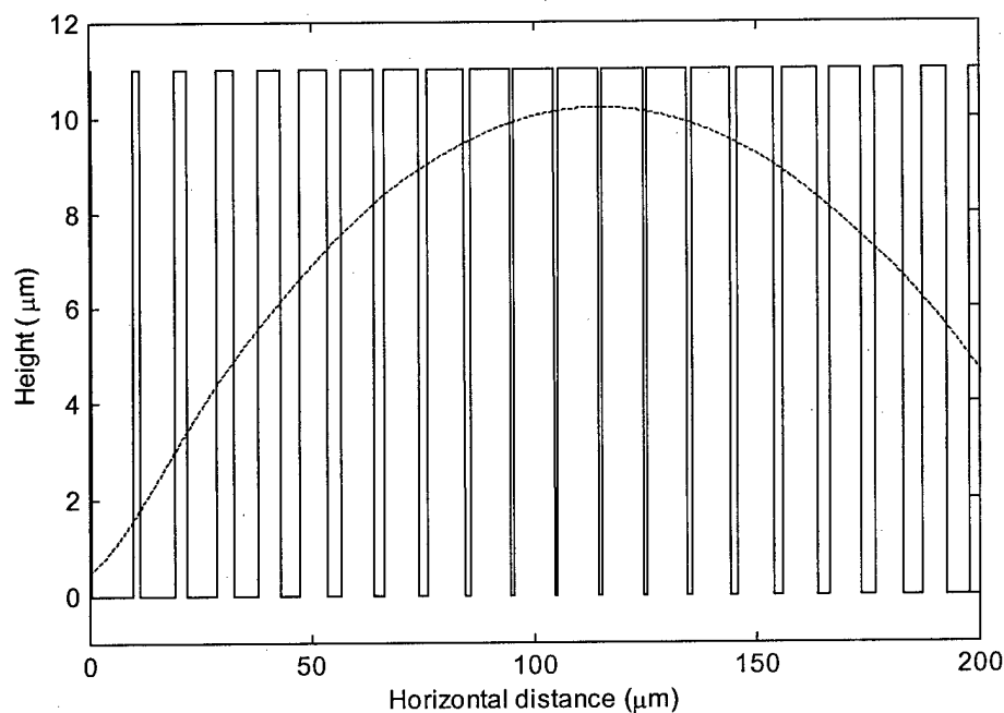
Figure 4.6. Simulated smoothing of a binary pre-form to generate an off-axis GaP lens ( f/1.5 , 200- \mu\text{m} diameter, 2.9^\circ steering angle) shown in cross-section. The solid line is the etched pre-form; the dashed line is the resulting surface after simulated mass-transport.
