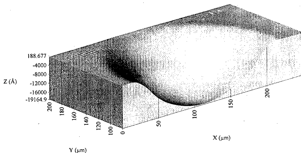
Figure 4.10. Profilometer measurement of a portion of the fabricated GaP concave micromirror.
