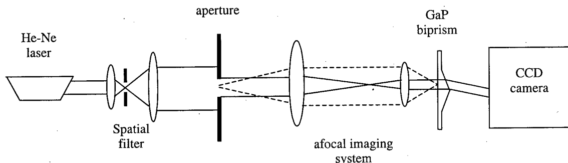
Figure 4.4. Experimental set-up for testing beam-steering of GaP biprism with normally-incident He-Ne beam.
