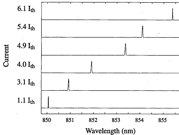
Figure 4.14. Spectral data for a 15- \mu\text{m} VCSEL with spatial filtering; the VCSEL stays single mode for currents up to 6I_{th} .
