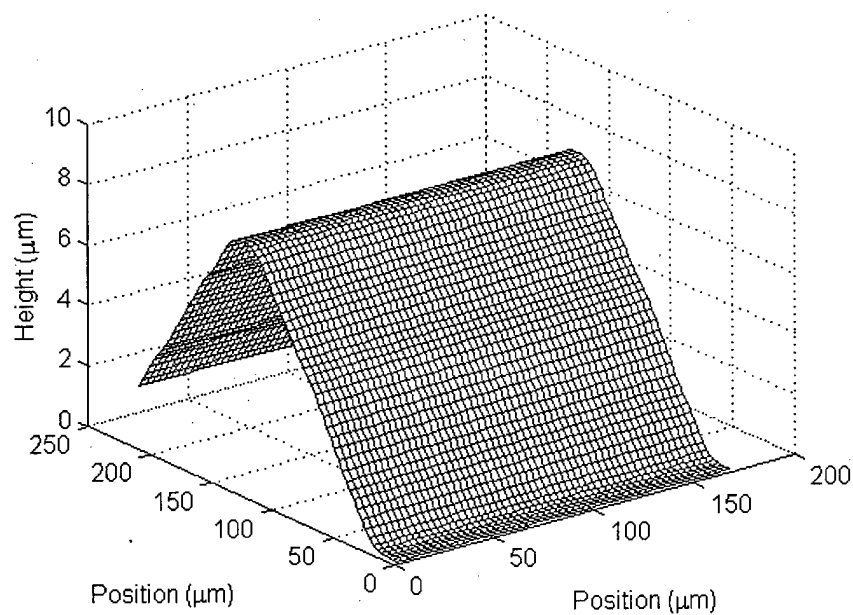
Figure 4.3. Scanning white-light interferometric microscope data for GaP biprism after transport.
