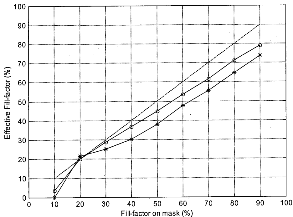
Figure 4.27. Calibration plot of effective fill-factor vs. mask fill-factor: ideal case (dashed line), 17.6 \mu\text{m} etch depth (o), 26.8 \mu\text{m} etch depth (*).
