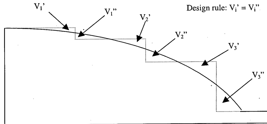
Figure 2.3. Equal-mass design method for multi-step pre-form; Before transport (dotted), after transport (solid).
