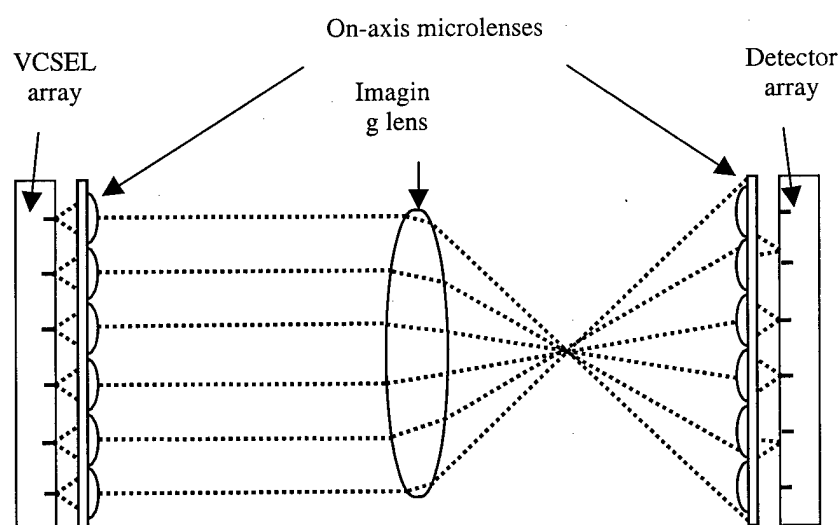
Figure 4.28. Optical interconnect system exhibiting distortion.
