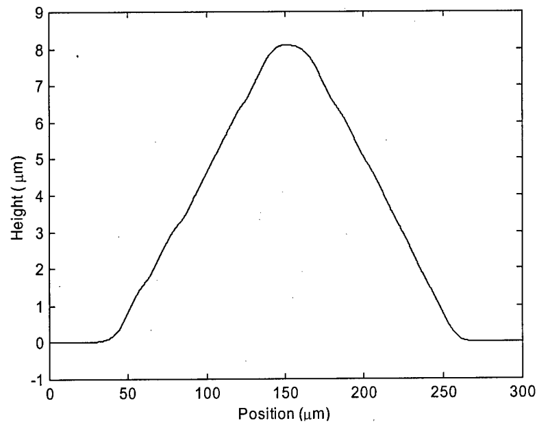
Figure 4.2. Surface profilometer data for GaP biprism after transport.
