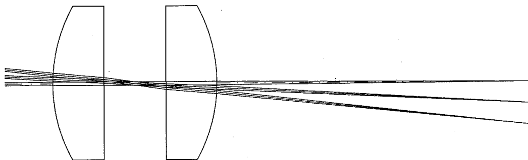
Figure 4.32. Code V system diagram showing three object field points; beams steered through center of imaging system.
