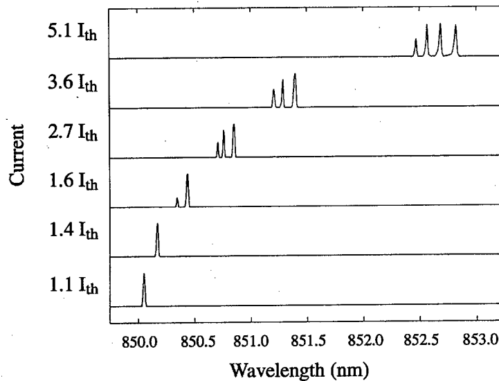
Figure 4.13. Spectral data for a 15- \mu m VCSEL without spatial filtering; the VCSEL becomes multimode at a drive current of 1.6I_{th} .
