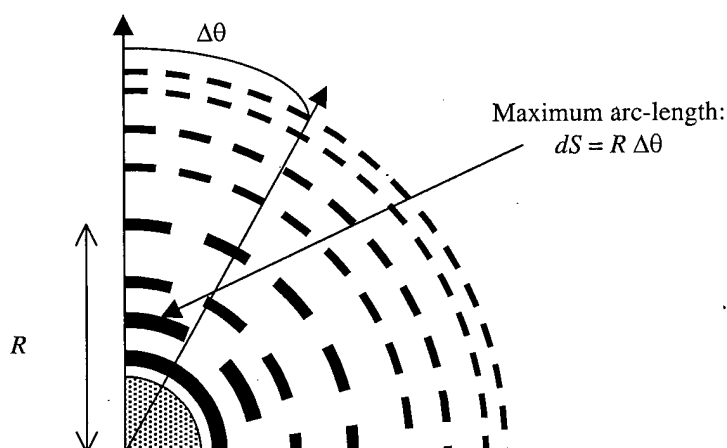
Figure 2.15. Segmented concentric ring pre-form to allow angular variation and larger ring width (top view of one quadrant).
