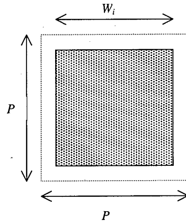
Figure 2.11. Two-dimensional fill-factor modulation design using square pixels (top view)
