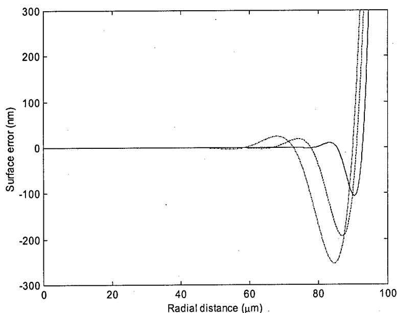
Figure 4.26. Preservation of surface figure: deviation of surface from parabola following simulated mass-transport for 1 (solid), 10 (dashed), and 28 hours (dot-dash).
