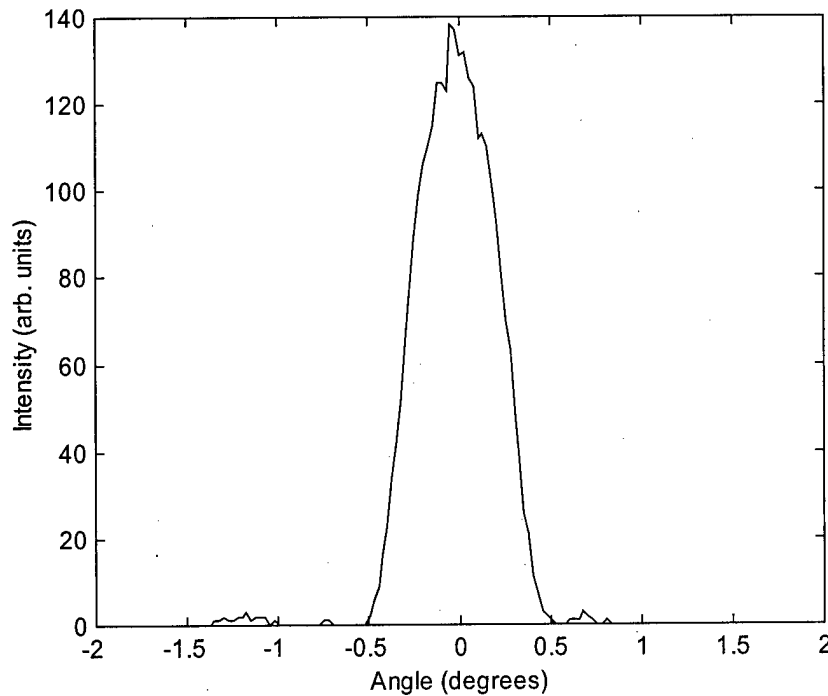
Figure 4.8. Far-field intensity data for GaP off-axis lens.
