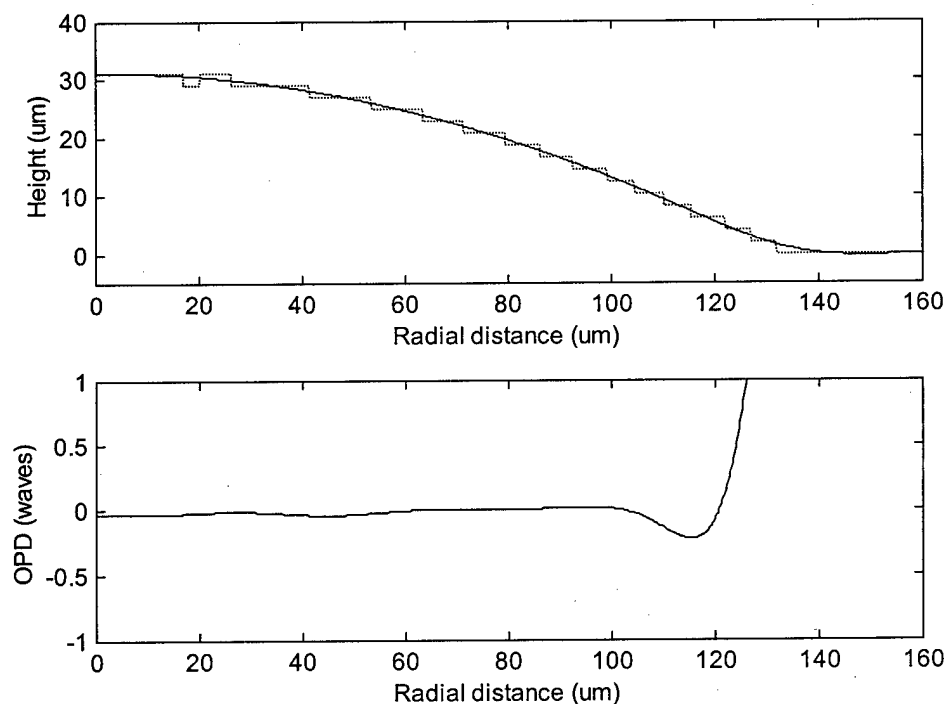
Figure 2.6. (a) Simulation before (dotted) and after transport (solid) with trench in top step and optimized step widths; 16 levels; (b) Optical path difference between simulated and design surfaces.
