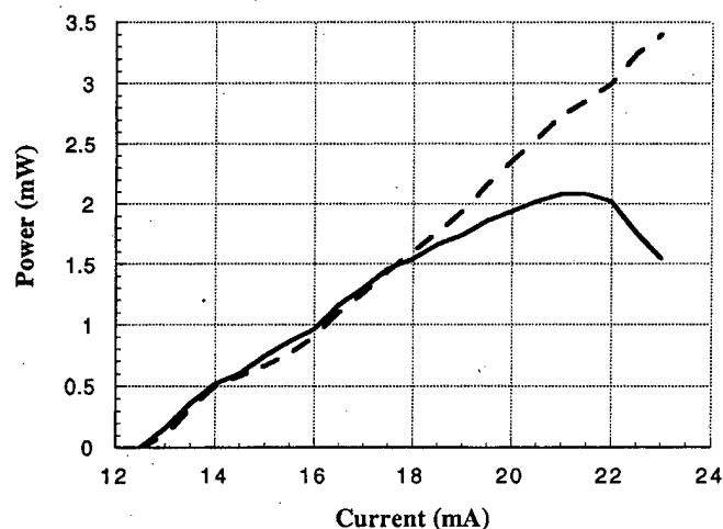
Figure 4.15. L-I curve for a 10- \mu m VCSEL with spatial filtering (solid line) and without spatial filtering (dashed line).
