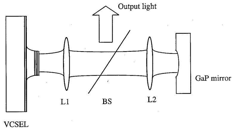
Figure 4.12. Experimental arrangement used to test the micromirror. The afocal system (L1 and L2) images the VCSEL onto the micromirror. Varying the focal lengths of the two lenses allows different beam magnifications to be obtained. A beam splitter (BS) couples light out of the cavity.
