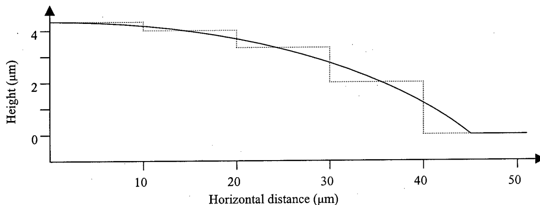
Figure 2.2. Multi-step pre-form before transport (dotted); after transport (solid).
