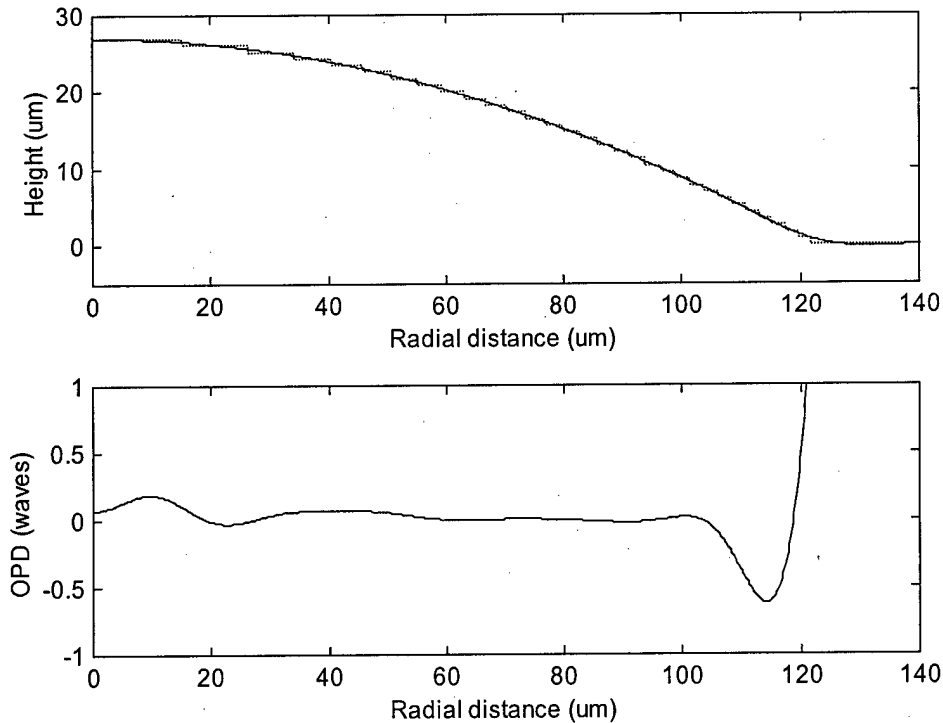
Figure 2.5. (a) Simulation before (dotted) and after transport (solid) with decreased top step height (b) Optical path difference between simulated and design surfaces.
