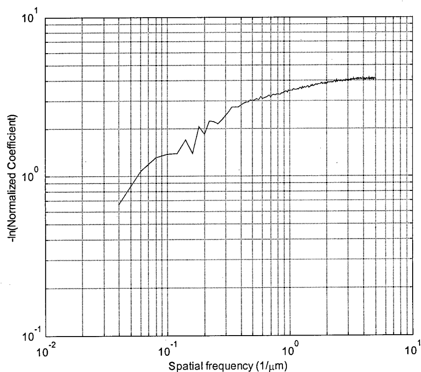
Figure 4.22. Amplitude decay of GaP surface roughness during mass-transport with 1- \mu\text{m} cover-wafer spacing.
