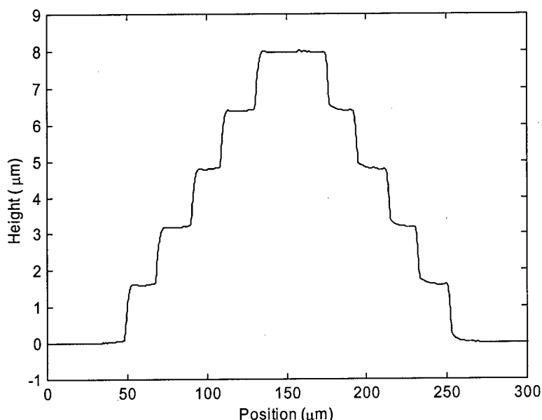
Figure 4.1. Surface profilometer data for GaP biprism pre-form before transport.
