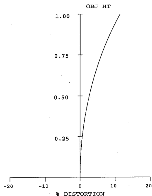
Figure 4.31. Plot of distortion as a function of fractional object height (1.0 object height corresponds to 2.828 mm) for system shown in Figure 4.30.
