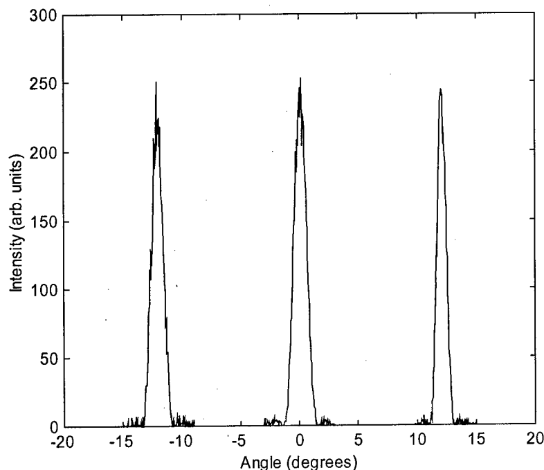
Figure 4.5. Far-field intensity data for He-Ne beam steered to three locations by GaP biprism.
