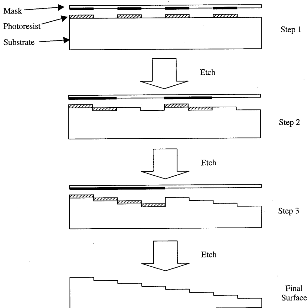
Figure 2.4. Binary optics fabrication of 8-level element using 3 masks; after [Swanson, 1989].
