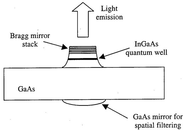
Figure 4.9. Micromirror integrated with an InGaAs VCSEL for spatial-mode discrimination through spatial filtering in the far-field.
