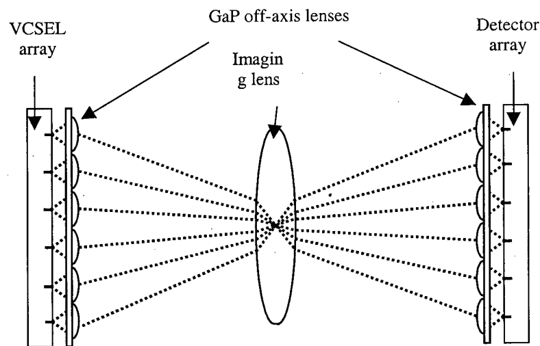
Figure 4.29. Diagram of optical interconnect system using off-axis GaP microlenses for distortion elimination.
