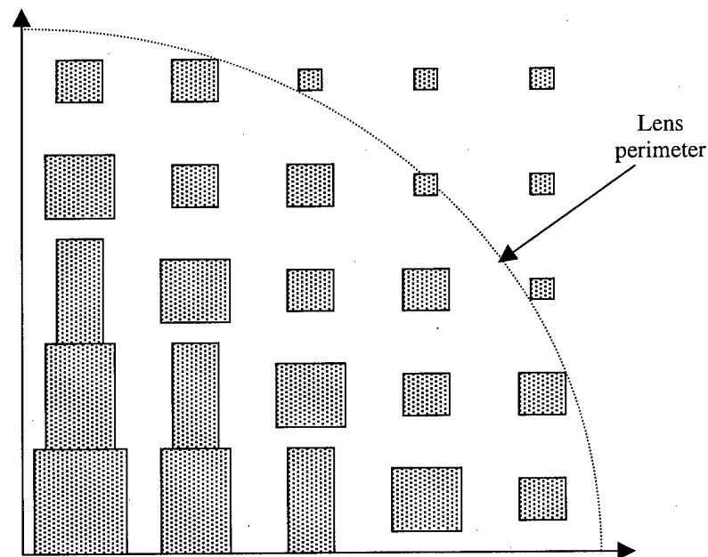
Figure 2.13. Hybrid 2-D/1-D fill-factor modulation method used to design a convex lens (top view of one quadrant)
