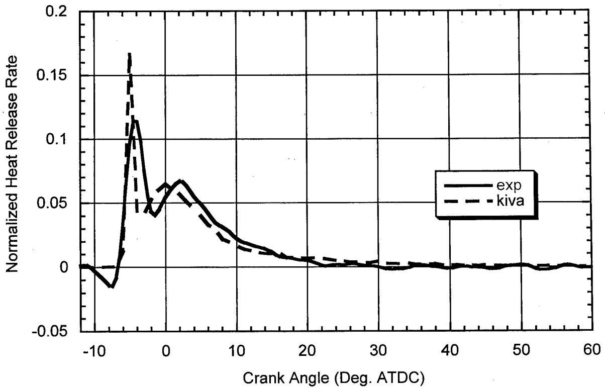
Figure 3: Comparison of coherent flamelet model with results for the Sandia engine (global equivalence ratio of 0.25).
