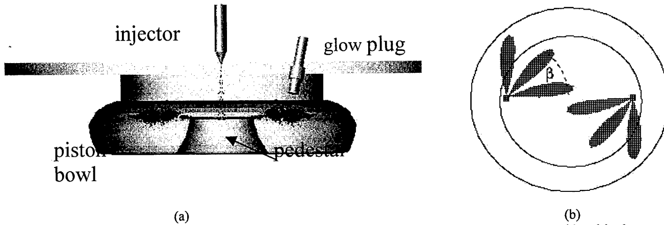
Figure 3: Schematics of the (a) SIMPLE combustion chamber geometry (glow plug was not considered in the present work) and (b) MICS-2 injection scheme.
