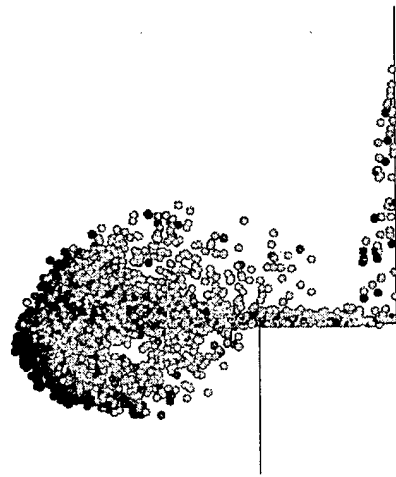
d) Computed spray drop distribution from KIVA.
