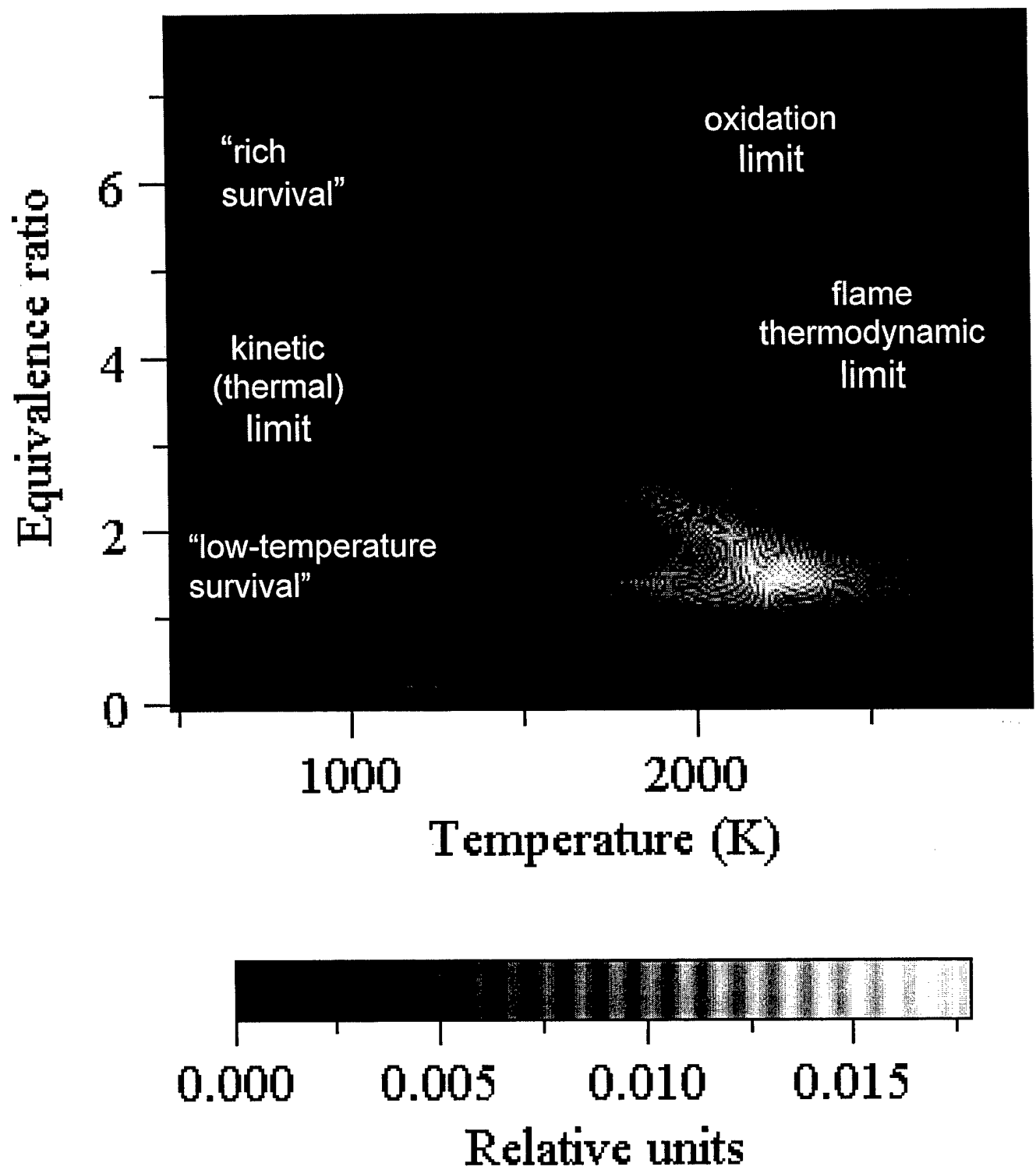
Figure 8: The cumulative history of soot formation and destruction during the engine cycle (see text).
