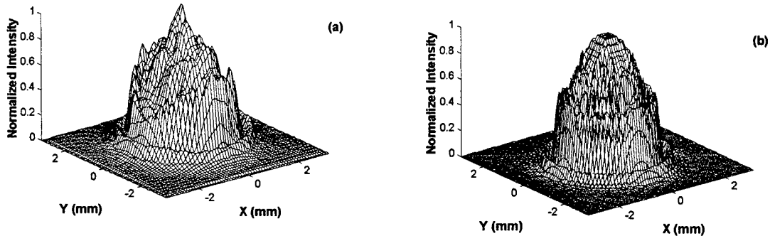
Fig. 9. (a) Observed far field pattern of a top-hat pulse propagating through a 10 mm thick CS 2 sample. (b) Calculated far field beam profile for the top-hat pulse. The entrance plane to the NLO medium is located at Z = 0 mm.
