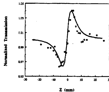
Fig. 5. Closed aperture Z-scan plot using a 1mm thick CS 2 cell, S=0.4. Points are the integrated signal from the CCD image. Solid line represents the integrated signal from the calculated far field beam profile by BPM.
