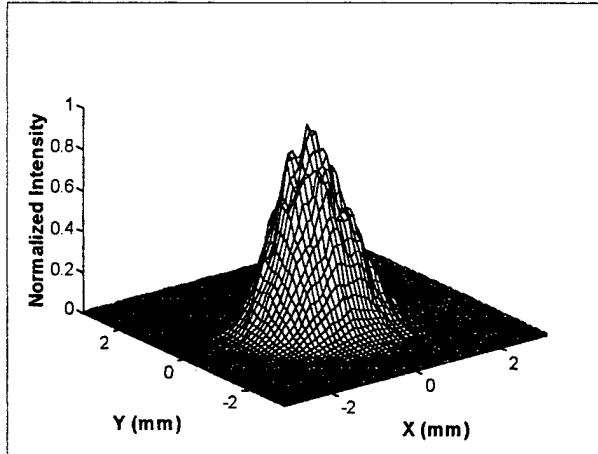
Fig. 2. Far field beam profile of the reference beam, recorded by a CCD camera.
