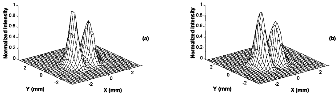
Fig. 10. (a) Observed far field pattern of a split Gaussian pulse propagating through a 10 mm thick CS 2 sample. (b) Calculated far field beam profile for the split Gaussian beam. The entrance plane to the NLO medium is located at Z = 0 mm.
