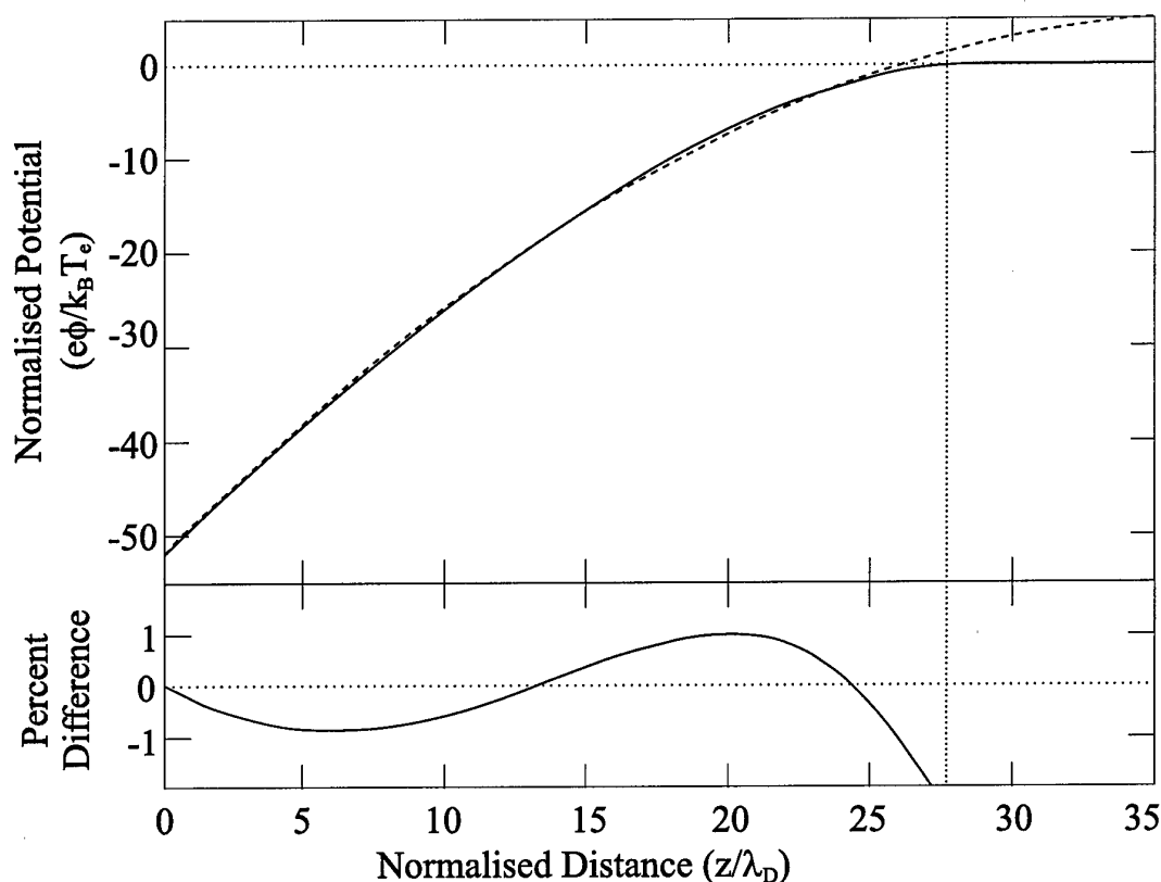
Figure 40: Parabolic Approximation to the Model of Bohm [1949]. This figure shows plots of the Bohm potential (upper plot, solid curve) and the best-fit parabolic approximation (upper plot, dashed curve) for the conditions stated in the text. The difference between the curves is shown in the lower plot. For these particular conditions, the approximation does not differ by more than 1% of the maximum potential from the numerical curve across a vast majority of the sheath.
