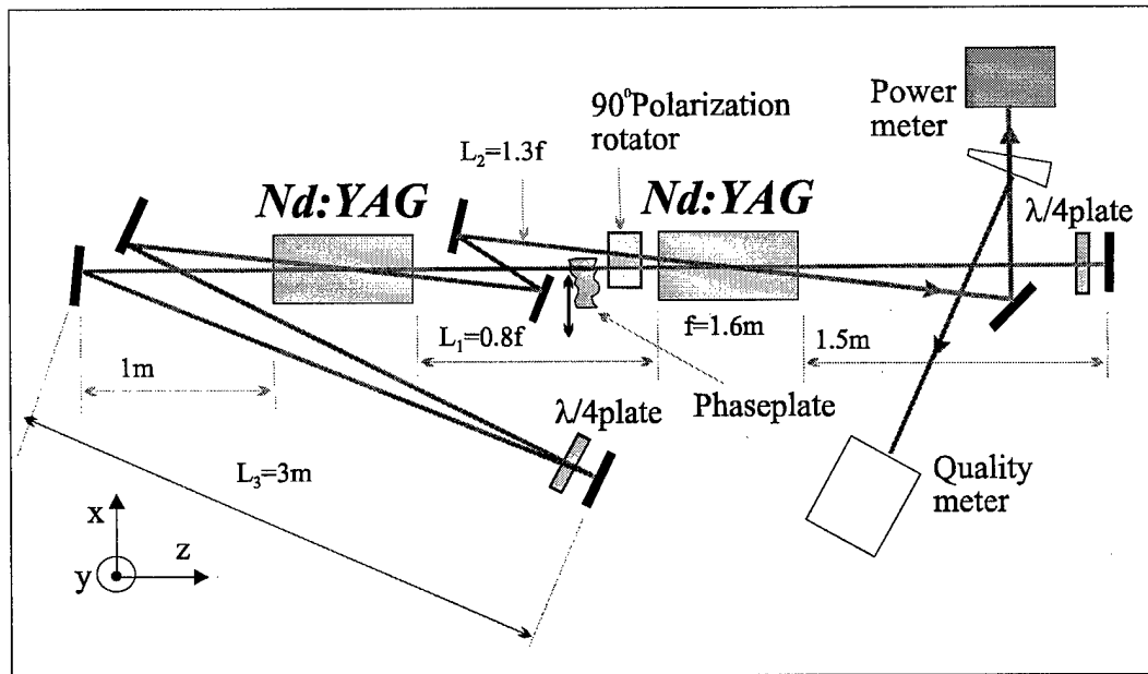
Fig. 8. The experimental setup of self-starting scheme based on two amplifiers (Nd:YAG rods with sizes \text{Ø}10 \times 135 \text{ mm} ).
