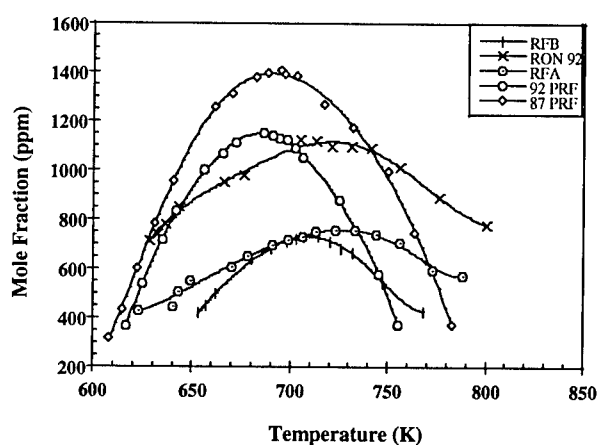
Figure 2: Olefin formation for multicomponent blends
