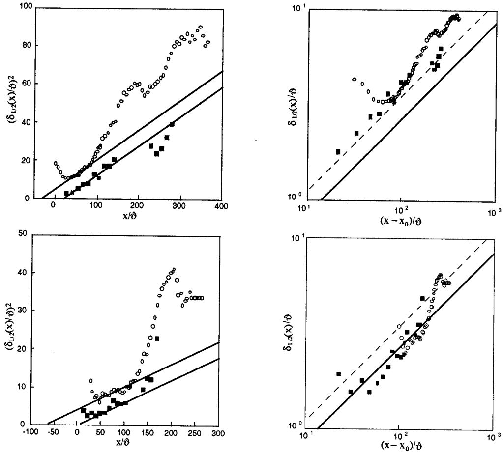
Figure 2. Flow width \delta_{1/2} obtained from mean PLMS intensity profiles ( circles ) and mean velocity profiles ( squares ) for M = 2 ( top ) and M = 3 ( bottom ). Straight lines show (\delta/\delta) \sim (x/\delta)^{1/2} incompressible wake scaling. Increased growth rates coincide with recompression wave intersections. Log-log forms show lines indicating 1/2-power law scaling for values of the far-field scaling constant c_\delta in forced incompressible wakes ( dashed line ) and unforced incompressible wakes ( solid line ).
