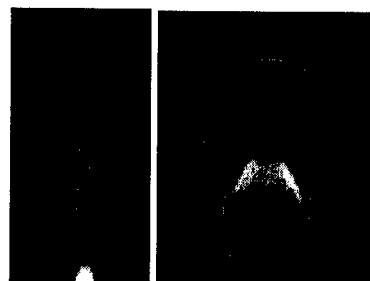
Fig. 1. (a) At left: single-shot visualization of the fuel region of a CO/Ar/H 2 laminar diffusion flame generated using IR PLIF of CO. (b) At right: single-shot visualization of mixing of a forced CO 2 /Ar jet in air generated using IR PLIF of CO 2 .
