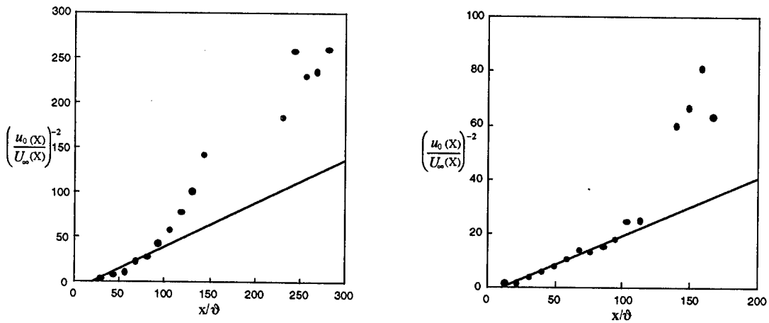
Figure 3. Comparison of velocity defect decay for M = 2 ( left ) and M = 3 ( right ) using the same \delta . Straight lines show classical (x/\delta)^{-1/2} incompressible wake scaling of the centerline velocity defect. Note that the compressible turbulent shear flow follows the same scaling as the corresponding incompressible flow, with the only apparent differences being due to reflected expansion and recompression wave intersections.
