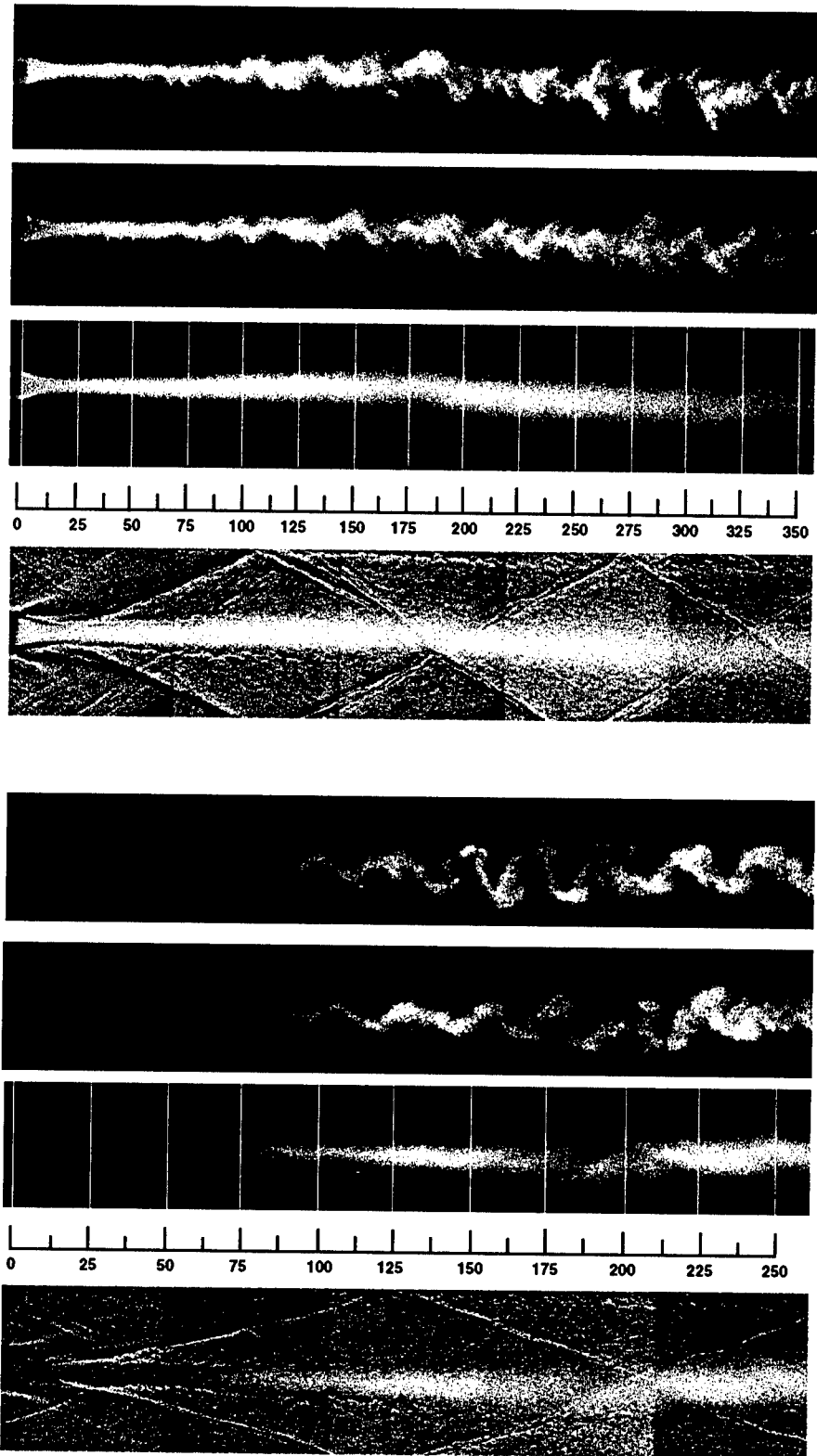
Figure 1. Instantaneous and mean planar laser Mie scattering (PLMS) images and instantaneous shadowgraph images of the supersonic planar turbulent wake at M = 2 ( top ) and M = 3 ( bottom ). Scales give the downstream distance in (x/\delta) . Note effect of wave intersections on growth rate and large scale structure of the flow.
