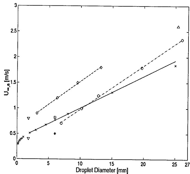
Fig. 2. Extinction velocity vs. droplet diameter: (x) - numerical predictions for n-heptane under zero-gravity ( T_{\infty} = 300 K and p_{\infty} = 1 atm). Experimental data under normal-gravity for various fuels in air at "room" temperature and atmospheric pressure; (o) - kerosene (Spalding, 1953), (h) - n-butyl alcohol (Agoston et al., 1952), (*) - n-heptane (Gollahalli and Brzustowski, 1975), ( ) - previous point corrected for natural convection, (V) - gasoline (Agafonova et al. 1960, lower: aiding natural convection, upper: opposing natural convection), (Δ) - n-heptane (Gore et al., 1990)
