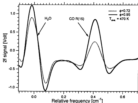
Fig. 3. Representative 2f lineshapes (~1.46 modulation index, 20-sweep average) for CO measurements in the 120-cm exhaust duct of a laboratory combustor.
