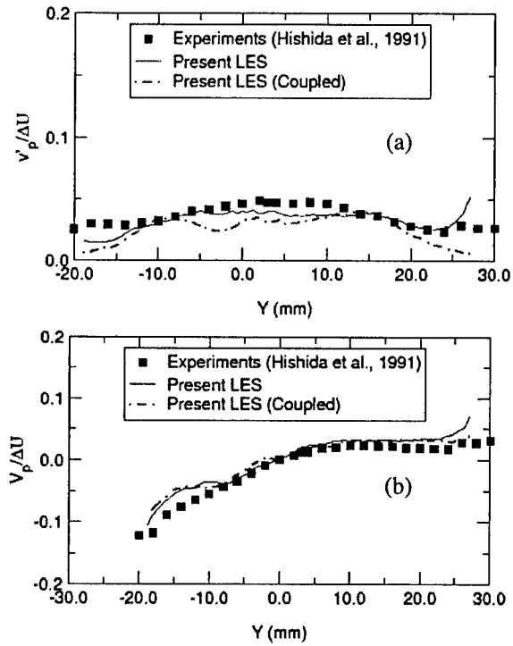
Figure 6. Particle phase velocity profiles at x=200 mm for 42 \mu\text{m} droplets: (a) v_{rms} , (b) v_{mean} .
