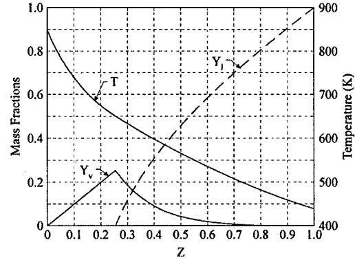
Fig. 4: Vaporization state relationship: T_a=850 K, \rho_a=60 kg/m 3 . T_f=438 K: liquid and vapor mass fractions and temperature.
