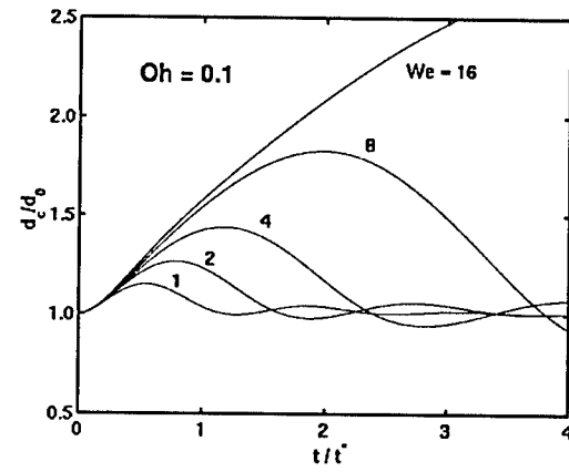
Fig. 4 Normalized liquid column deformation of nonuniform round liquid jets in uniform crossflows as a function of normalized time.
