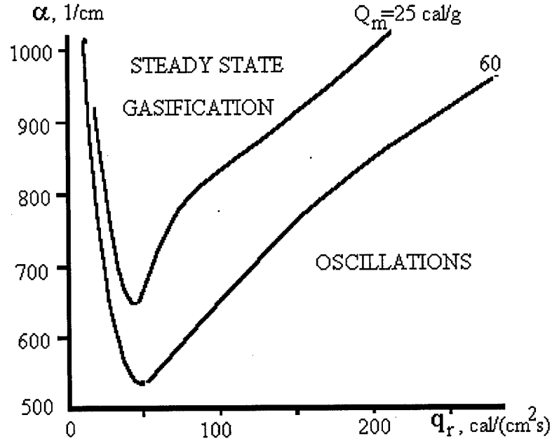
Fig.6.5. Map of the existence of stationary gasification regimes
