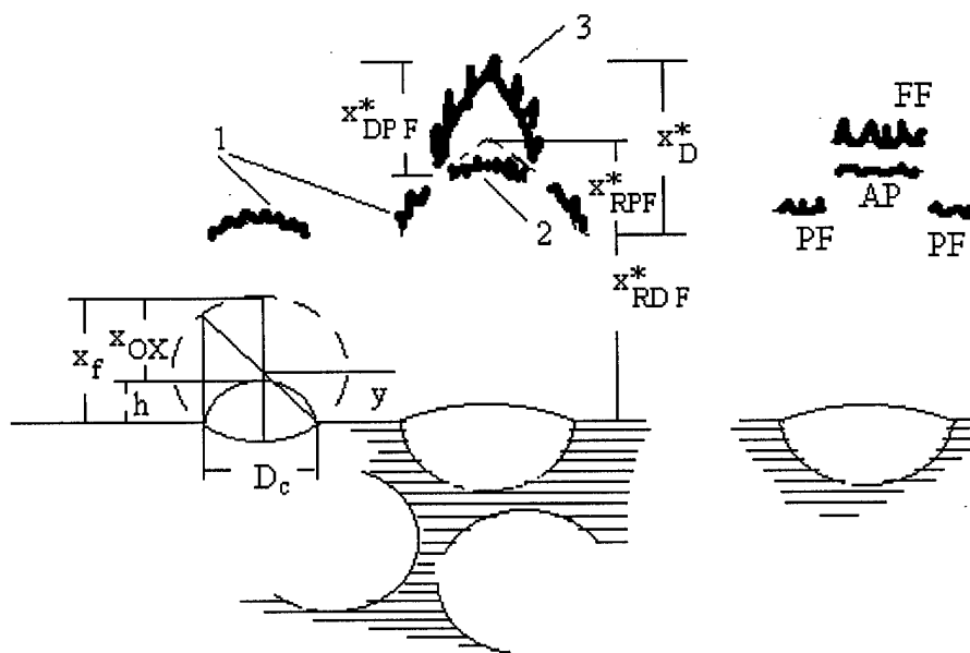
Fig. 3.2. Diagram of flames in BDP model.
