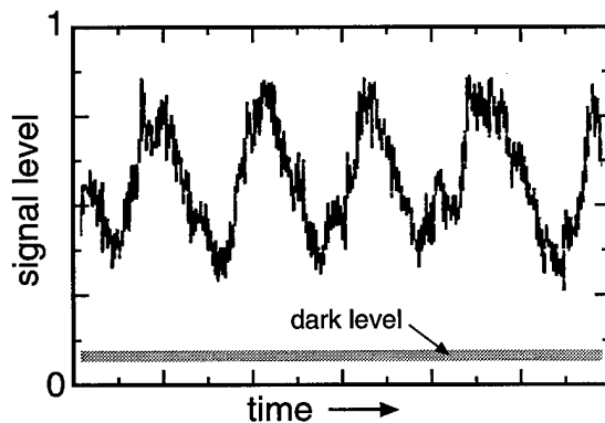
Figure 10. This signal was recorded from a 2- \mu m-period, organic, scintillating fiducial grating. An electron beam scanned the grating and a photomultiplier tube detected the modulated optical signal. The signal contrast (maximum-to-minimum ratio) was measured to be 2.8. This value is significantly higher than that obtainable from a fiducial grid designed for secondary-electron emission. The use of an organic scintillator is preferred over the use of metals for the fiducial grid.
