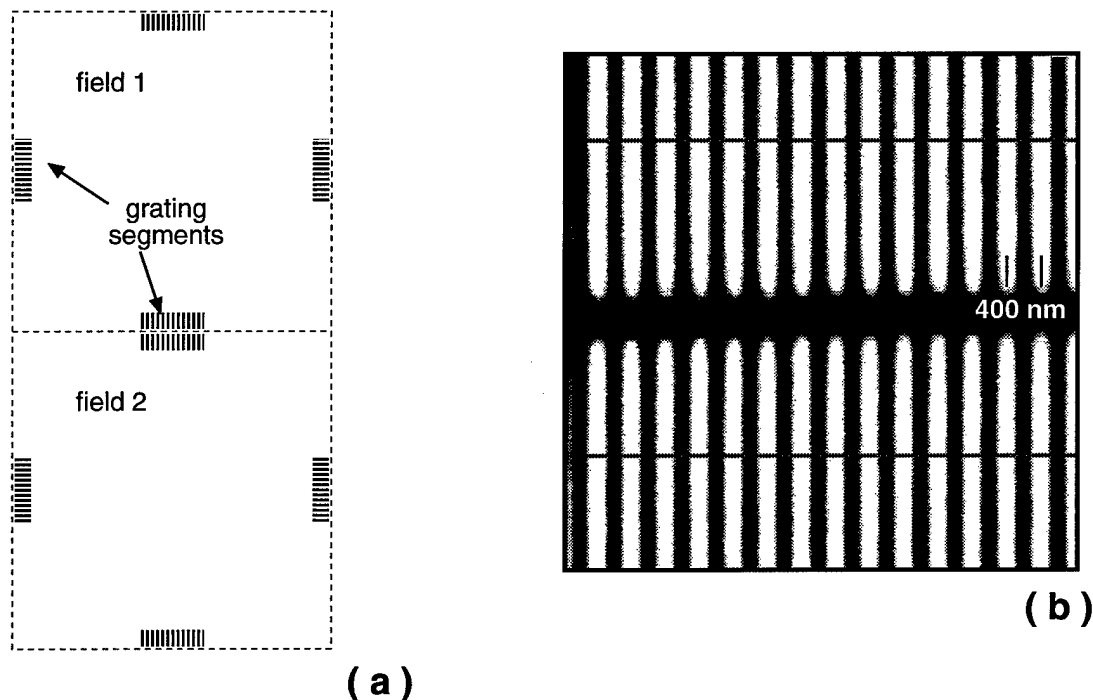
( a ) Figure 6. Grating segments were patterned near the edge of the e-beam field (a) in order to evaluate the field-stitching precision. A careful inspection of the paired grating segments (b) enables an evaluation of field-stitching precision at the sub-1 nm level. The horizontal lines in (b) indicate the e-beam scan path used to extract the spatial phase of each grating segment. Each segment was scanned 64 times to extract the spatial phase.
