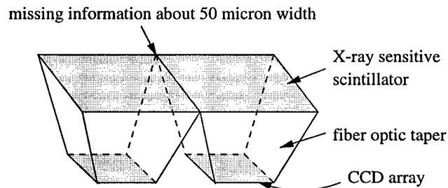
Figure 1. Demonstration of two scintillator/fiber/CCDs butted together.
