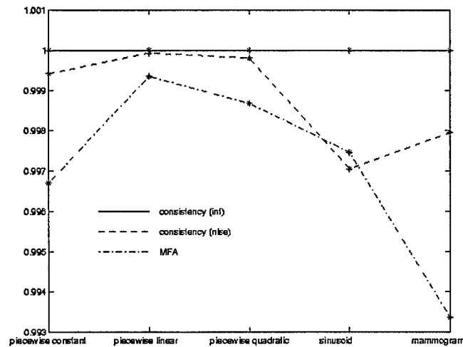
Figure 16. Cross-correlation comparison.
