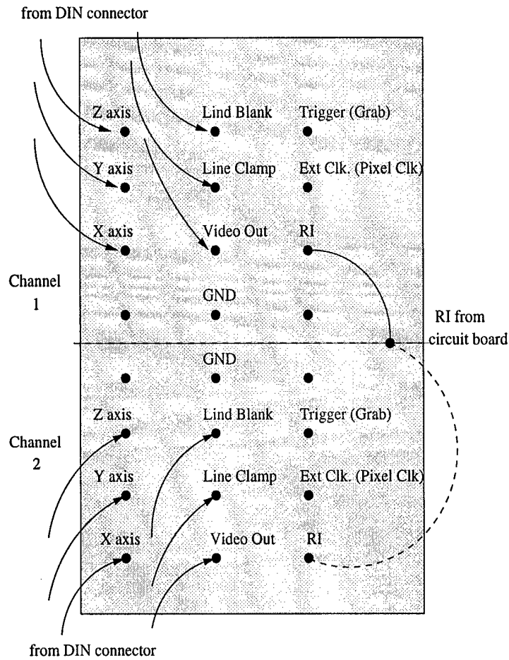
Figure 31. Test pod signals.
