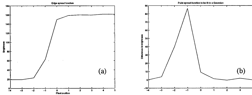
Figure 59. The edge spread function and the point spread function.
