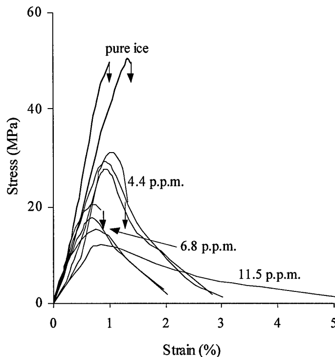
Figure 2. Comparison between engineering stress-strain curves for sulfuric acid-doped and undoped ice single crystals with the C axis at 3° to the loading direction, at an initial axial strain rate of 1 \times 10^{-5} \text{ s}^{-1} at -20°C. The downward arrows indicate specimen failure, which occurs at higher strains with increasing sulfuric acid concentration.
