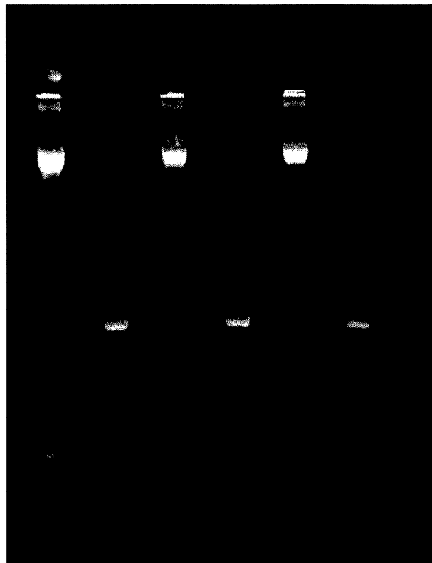
Fig. 2. The PCR products obtained from representative microorganisms using specific primer pairs. Lanes 2, 6, 10 C. albicans (704 bp); lanes 3, 7, 11 E. coli (384 bp); lanes 4, 8, 12 P. vulgaris (1226 bp). Marker lanes (M).
