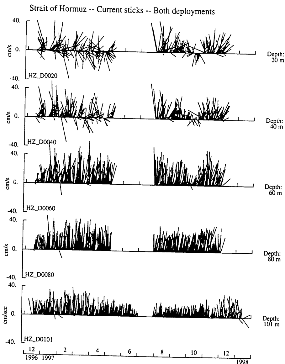
Fig. 7: Lowpass filtered current vectors from ADCP mooring in the Strait of Hormuz. Depth levels are 20, 40, 60, and 80 m from the ADCP, and 101 m from a near-bottom conventional current meter. Currents are rotated, up is 055^\circ true, out of the Strait.
