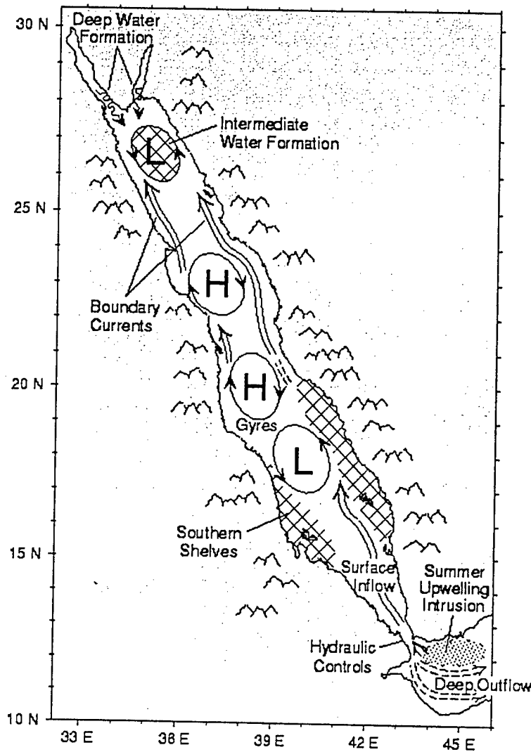
Fig. 3b: Circulation schematic for the Red Sea.
