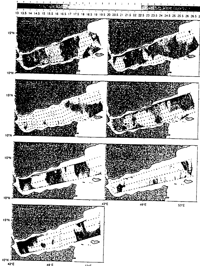
Fig. 12: Temperature at 100 m in the Gulf of Aden from repeated AXBT surveys conducted by NAVOCEANO. Color shading indicates temperature in 0.5°C intervals, and small dots show AXBT positions.
