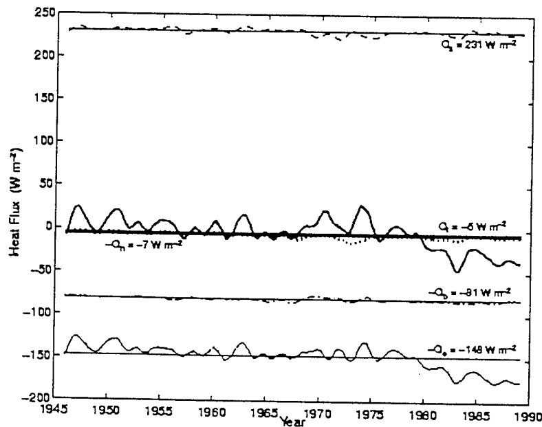
Fig. 14: Interannual variation of total heat flux and heat flux components in the Red Sea, after correction for systematic biases in the components.
