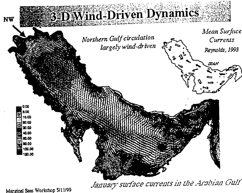
Fig. 23: Circulation snapshot from preliminary run of the NRL finite element Arabian Gulf model. The northern coastal boundary currents and general cyclonic circulation in the southeastern Gulf are clearly present, in general agreement with observations. (Forcing of thermohaline inflow from the Strait of Hormuz is not included in this model.)
