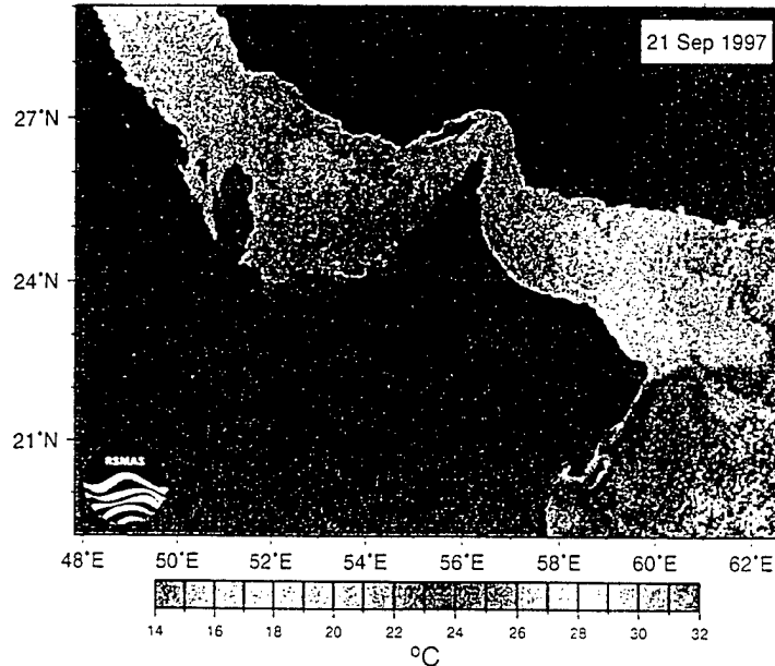
Fig. 17: AVHRR SST image for the Arabian Gulf and Gulf of Oman for September, 1997, showing evidence of a warm coastal plume emanating from the Strait of Hormuz.
