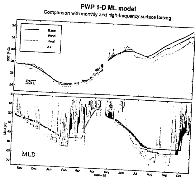
Fig. 15: Comparisons of results from the Price Weller Pinkel 1-D mixed layer model at the WHOI Arabian Sea mooring site, for monthly mean and high-frequency surface forcing. The base case (blue) is forced with monthly mean wind stress and heat flux, and no salt flux. The runs marked 'Wind' (cyan) and 'Heat' (purple) add high-frequency wind and heat forcing to the base case. The run marked 'All' (green) includes high frequency wind, heat, and salinity forcing. High-frequency forcing introduces both short term and low-frequency rectified effects on the SST and mixed layer depth.
