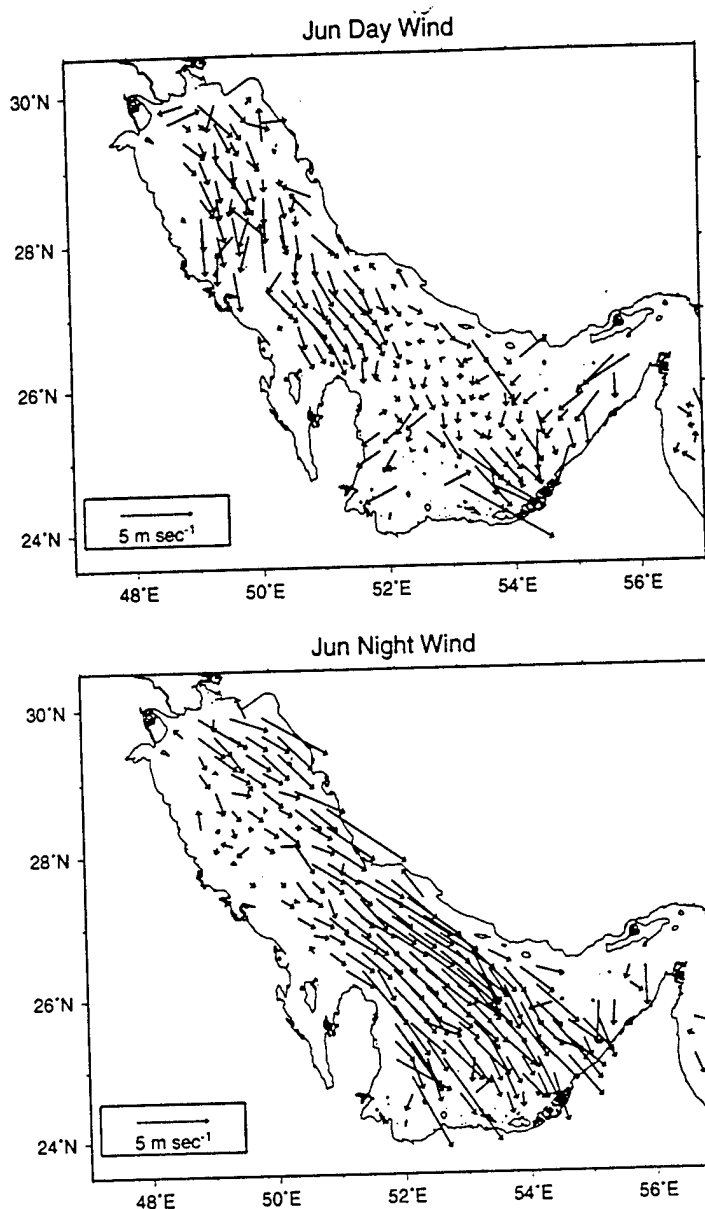
Fig. 21: Average day (top) and night (bottom) winds over the Arabian Gulf for June 1997 from the NSCAT mission.
