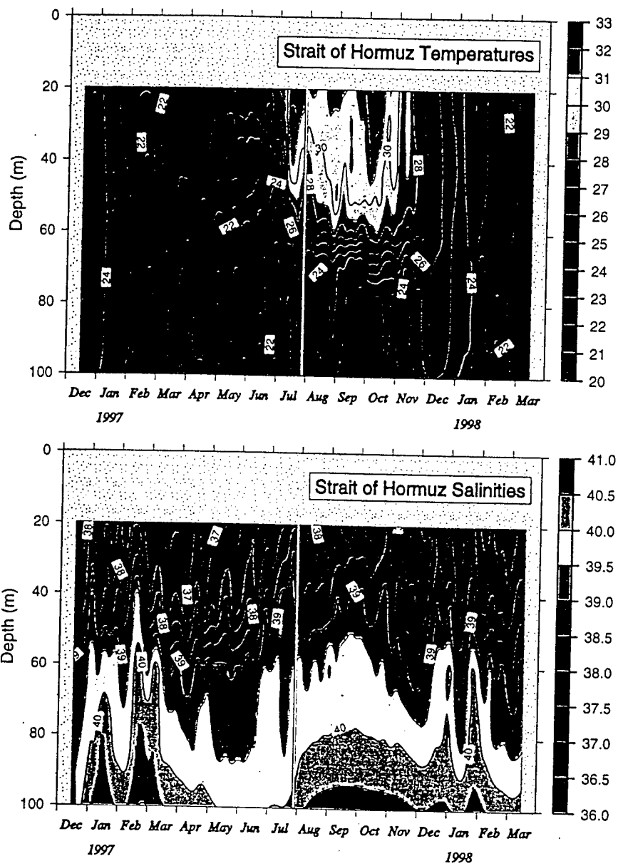
Fig. 8: Contours of temperature (top) and salinity (bottom) profiles in the Strait of Hormuz.
