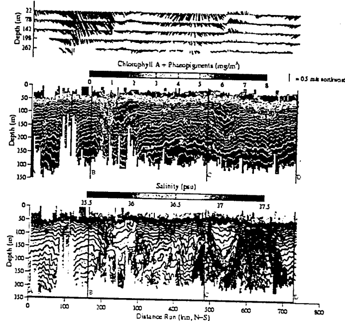
Fig. 13a: Sections of: (top) velocity, (middle) sigma-theta (in contours) and chlorophyll fluorescence (in colors), and (bottom) temperature (in contours) and salinity (colors) from the Northeast Monsoon. The section runs roughly parallel to the Omani coast. Point 'A' is within the Gulf of Oman, point 'B' is near Ras al Hadd and the remainder of the section runs southwestward along the coast well offshore of the shelfbreak. A large region of elevated salinities sits beneath an eddy at 250 km, and elevated salinities extend southward to 'C' at 500 km.
