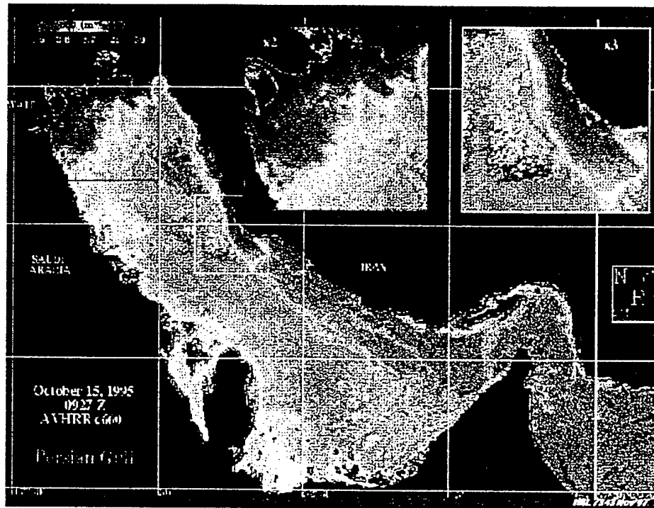
Fig. 19: AVHRR 660 nm band image of the Arabian Gulf for October, 1995. Strong signatures of the river outflow in the north and the coastal upwelling plume along the northern Iran coast are evident.
