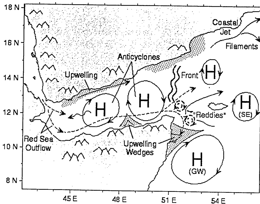
Fig. 3d: Circulation schematic for the Gulf of Aden and western Arabian Sea.
