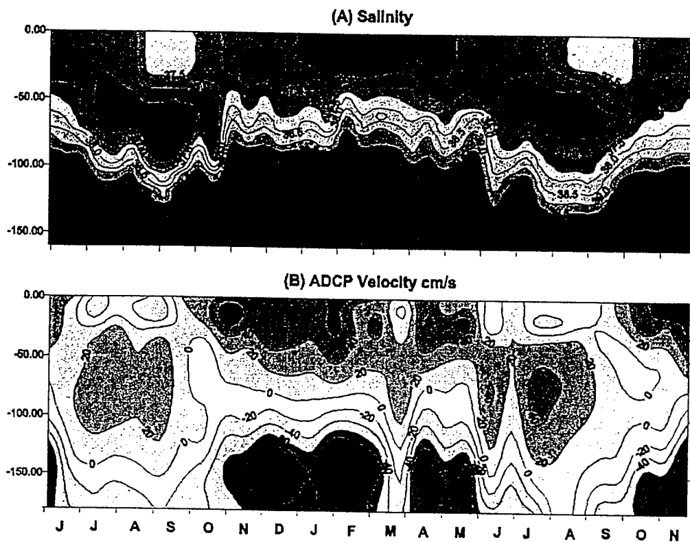
Fig. 5: Time series (June 1995 - November 1996) of salinity at the Hanish Sill (top) and ADCP alongchannel velocity at the Perim Narrows (bottom); negative velocities are outflow from the Strait. Note modulation of deep summer mid-depth intrusion, as well as a reversing surface layer.
