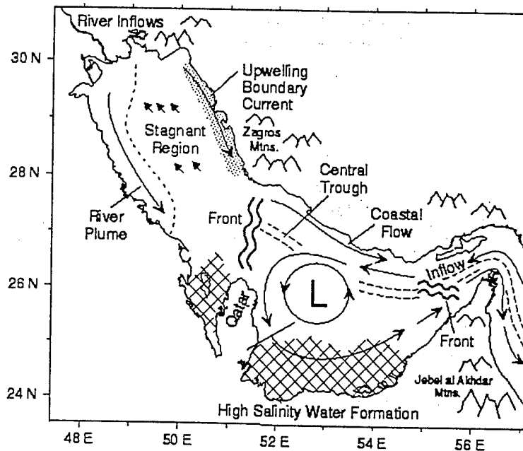
Fig. 3a: Circulation schematic for the Arabian Gulf.
