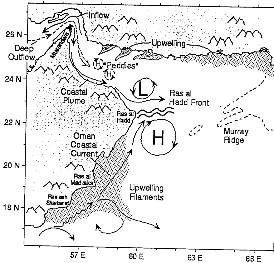
Fig. 3c: Circulation schematic for the Gulf of Oman and northern Arabian Sea.
