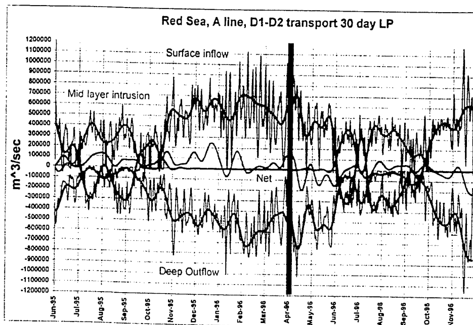
Fig. 6: Volume transports for the surface layer, the deep outflow layer, and the mid-depth summer intrusion in the Bab el Mandeb. The two-layer exchange in February reaches 0.7 Sv. Deep outflow diminishes to 0.05 Sv in summer. Annual average deep outflow \sim 0.39 Sv. Net flow into the Red Sea over one year (April 1995-1996) \sim 36,000 m^3/s .
