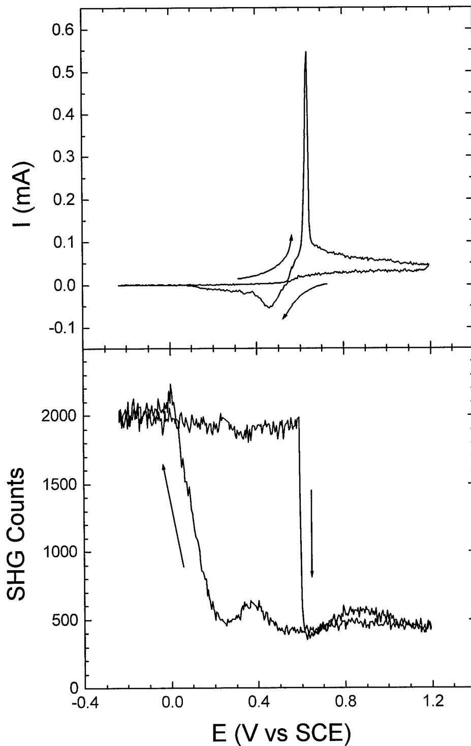
Fig. 5. Cyclic voltammetry (upper panel) and second harmonic generation signal (lower panel) obtained simultaneously for a Pt(100) electrode in a CO saturated 0.1 M \text{HClO}_4 solution in the range -0.2 to 1.2 V vs SCE. Scan rate: 50 mV/s. Electrode area: 0.32 \text{ cm}^2 .
