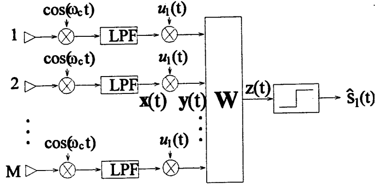
Figure 3.1: CDMA reverse link receiver model
