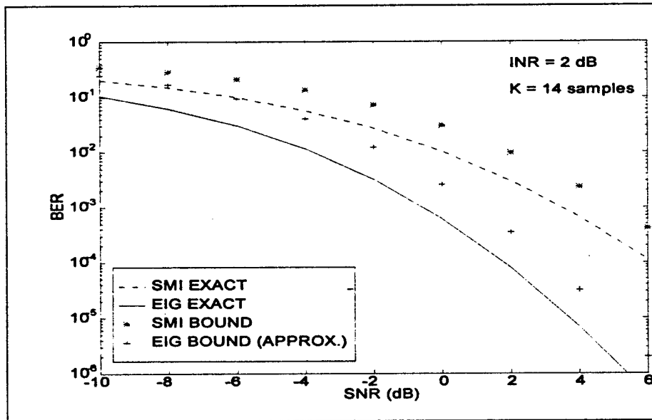
Figure 7.2: Bound and exact BER for SMI and eigencanceler with N = 9 elements and K = 14 training samples.
