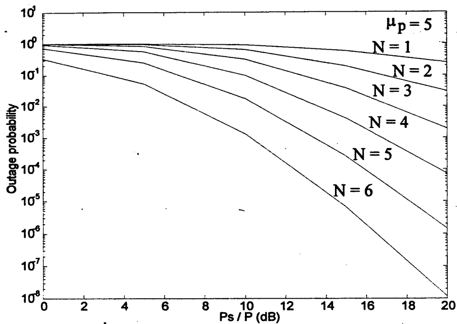
Figure 4.11: The outage probability versus \frac{P_s}{P_I} with the number of antenna elements N at the parameter
