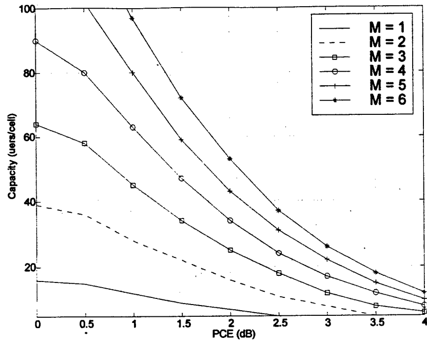
Figure 6.4: Capacity (users/cell) versus PCE for P_{oE} (\gamma_E < 7.5) = 0.01 . Analytical results for M = 1 to 6, and p = 3/8 .
